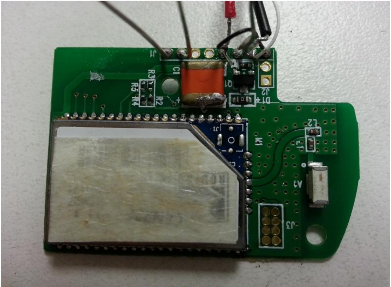
Front View
