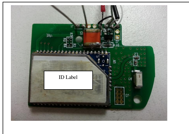
Figure 1 Proposed FCC/IC ID Label for 2.4GHz DTS Transmitter Module (The statement may be shown in its user manual for small size devices )
