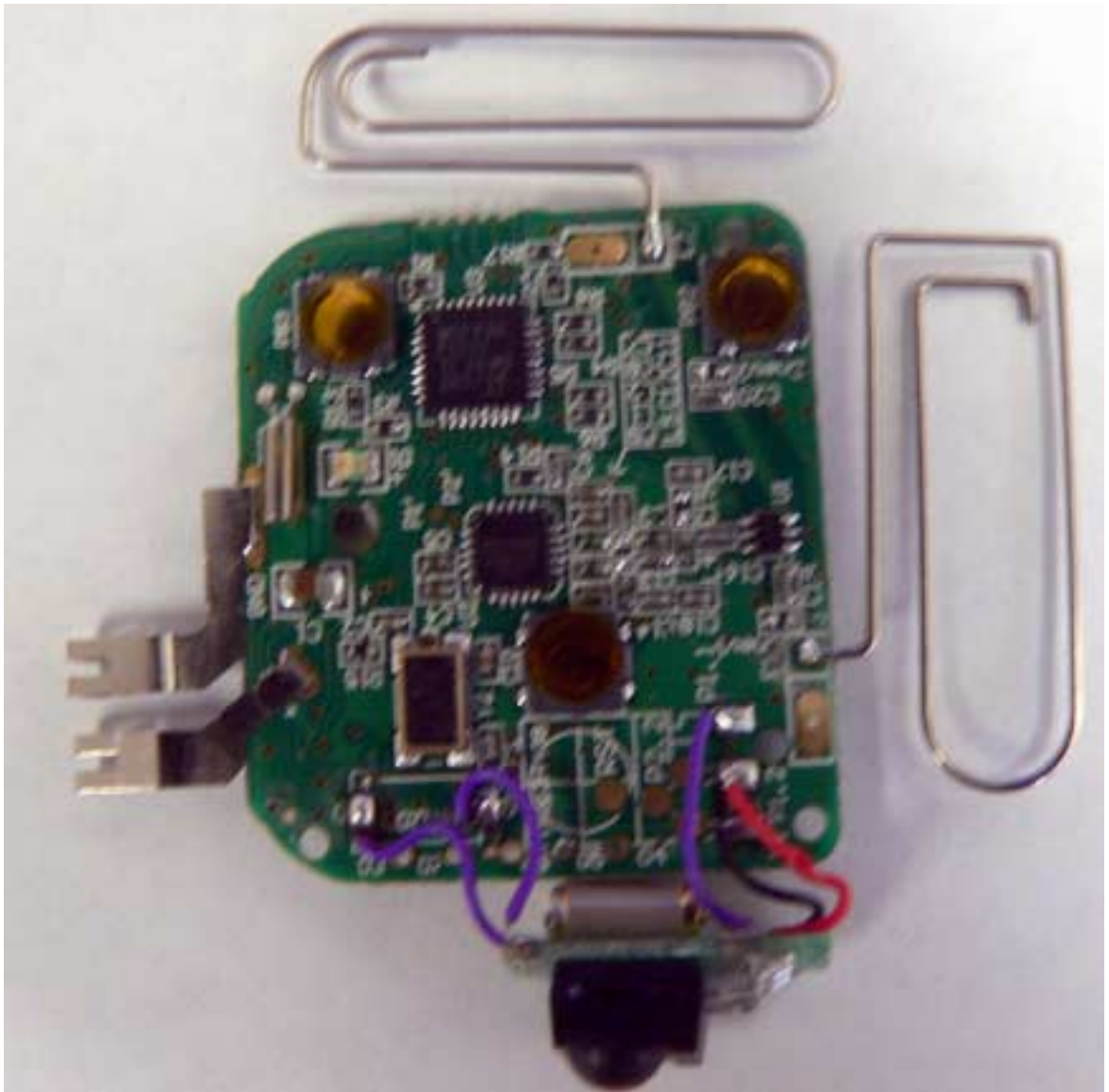
7.4 PCB Component View
