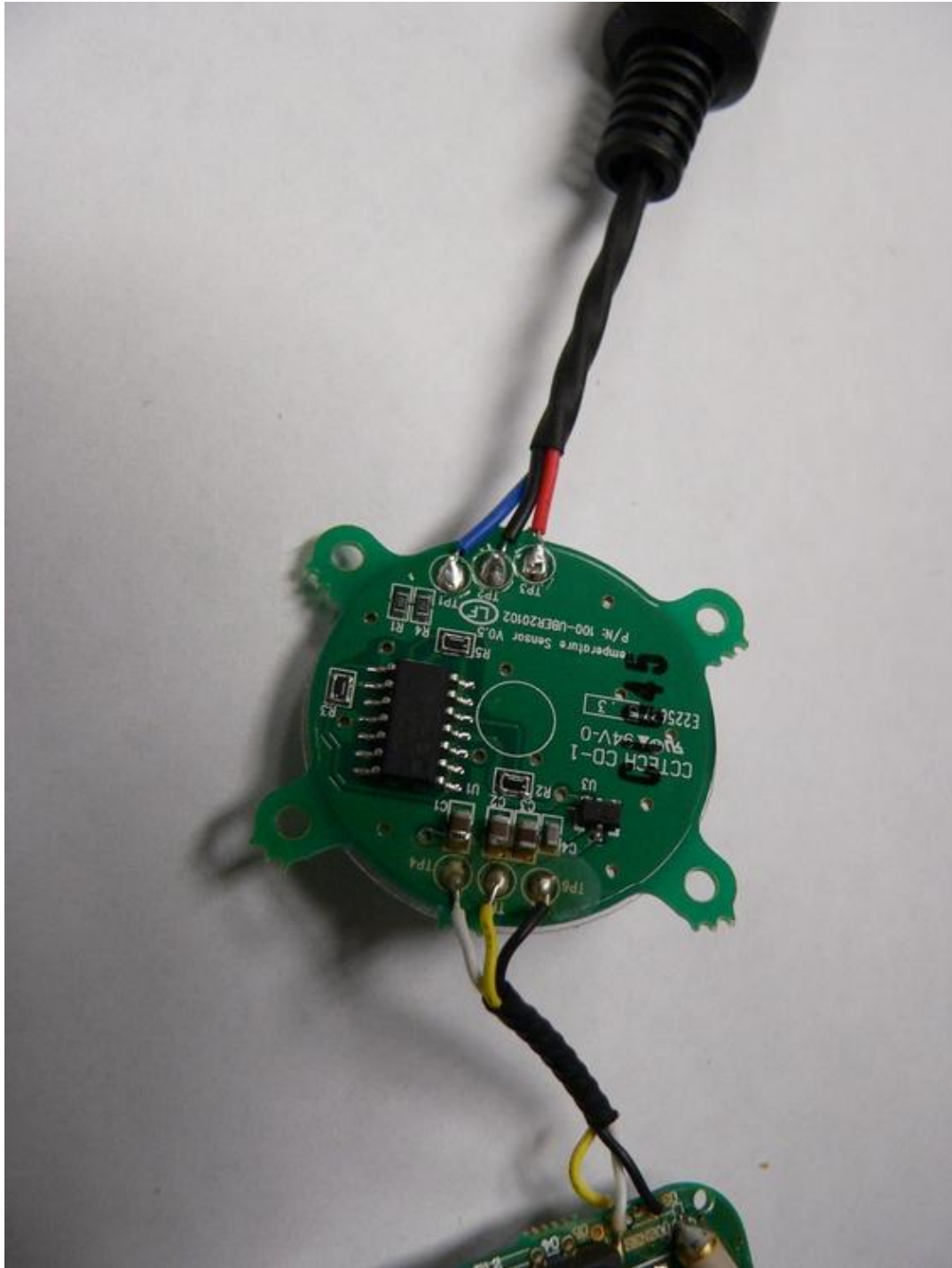
Temp Sensor PCB PCB Component View
