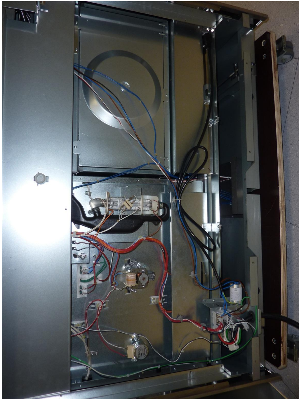
136015_3_d.JPG: HR1954, internal view 2 (rear cover removed)
