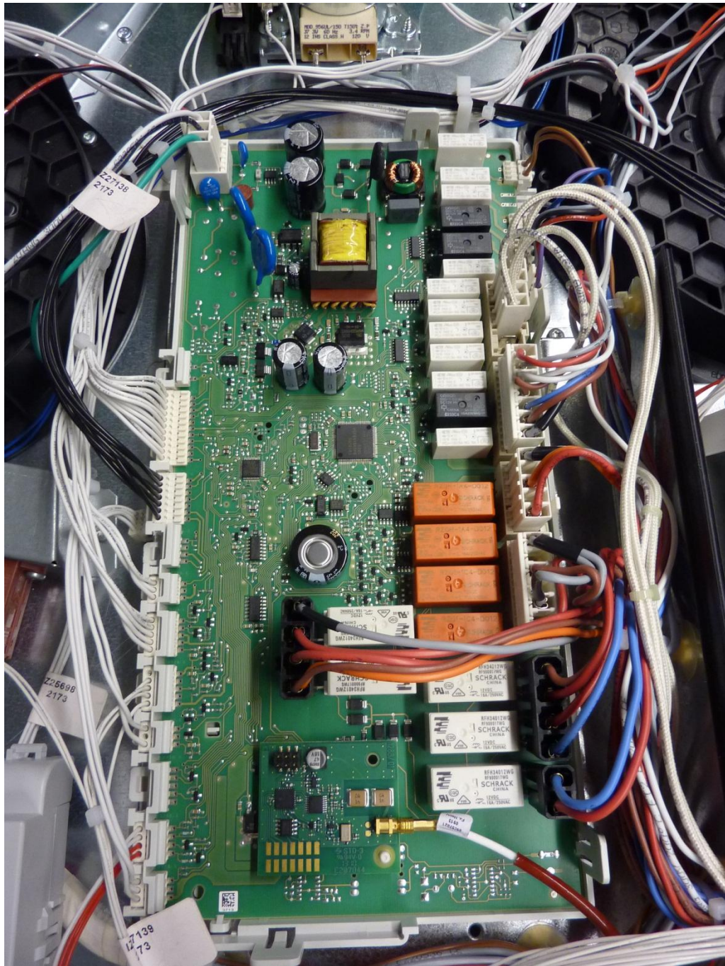
132604_3_f.JPG: EPI7674 inside H6780BP2, internal view to main PCB
