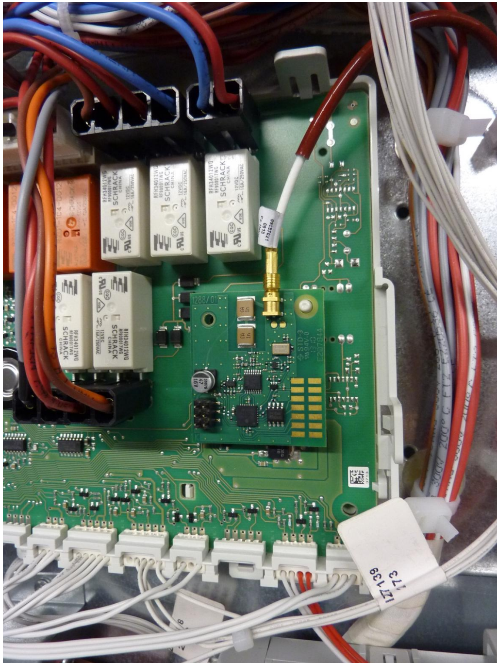
132604_3_g.JPG: EPI7674 inside H6780BP2, internal view to rf PCB on main PCB
