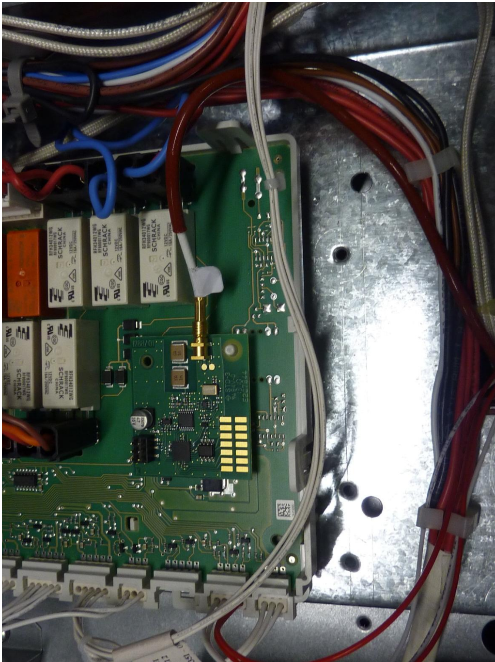
132604_1_m.JPG: EPI7674 inside H6780BP, internal view to rf PCB on main PCB
