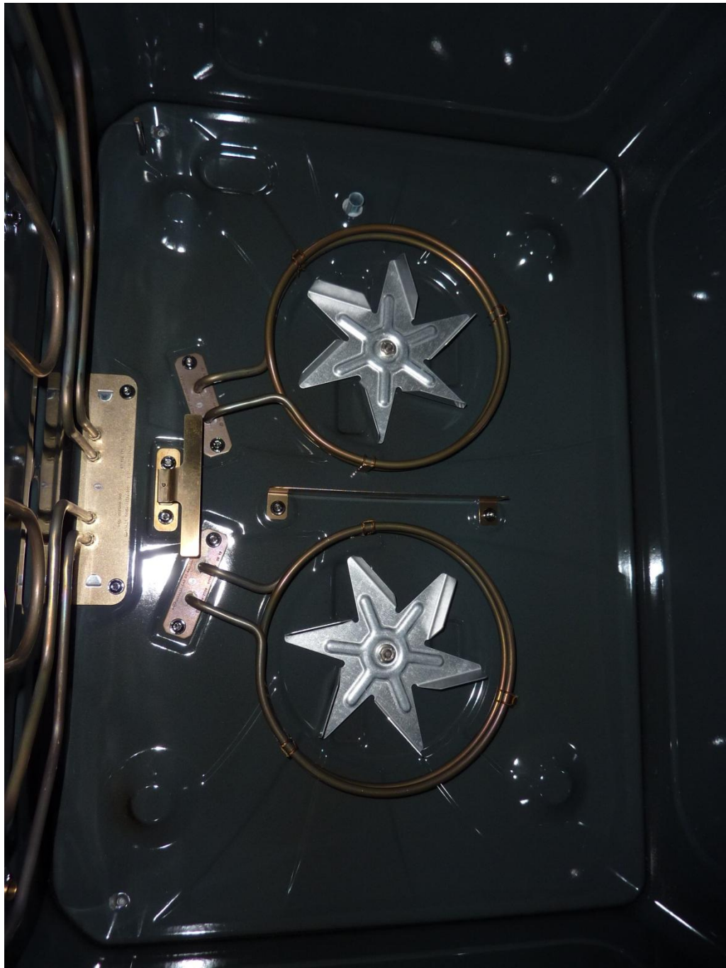
132604_1_p.JPG: EPI7674 inside H6780BP, antenna view
