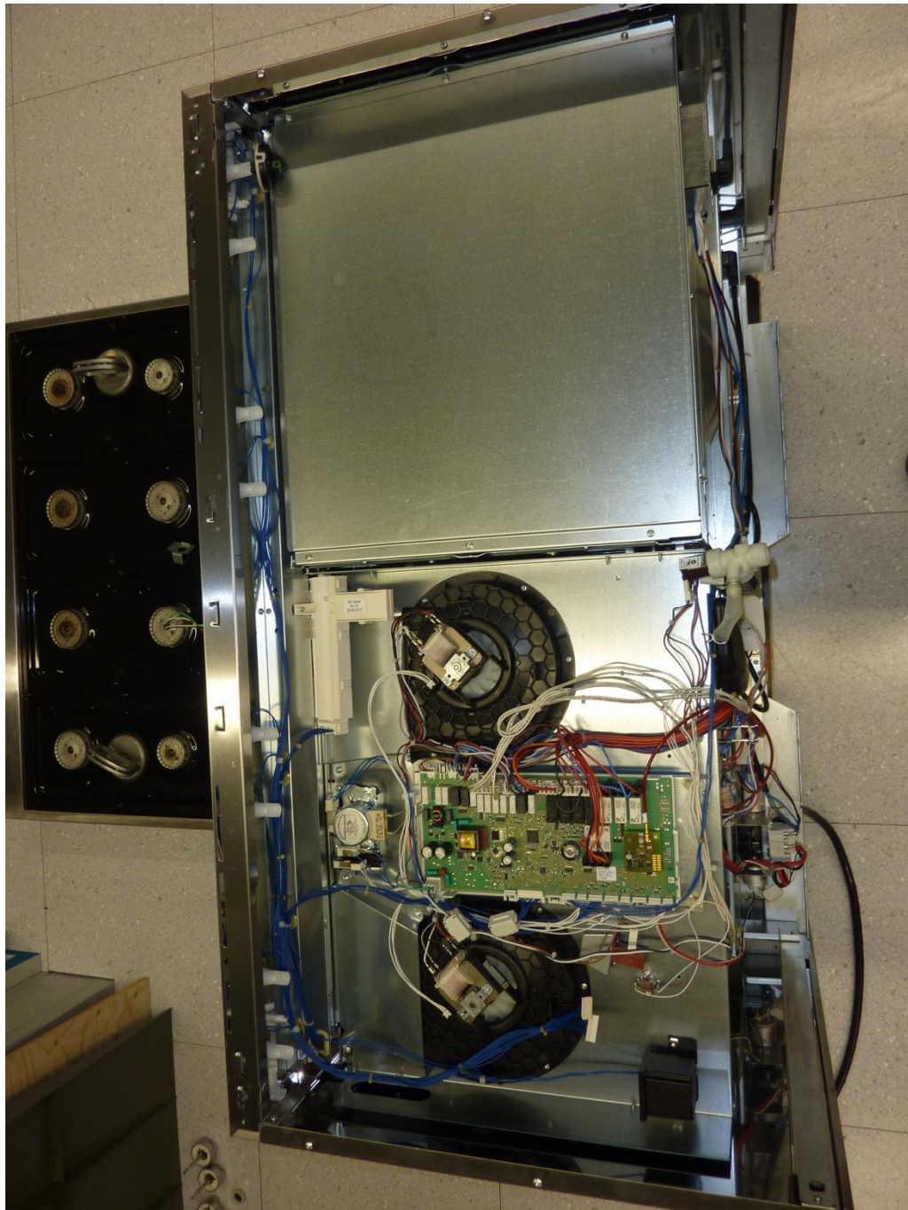
136015_3_g.JPG: EPI7674 inside HR1954, internal view 1 (cover removed)
