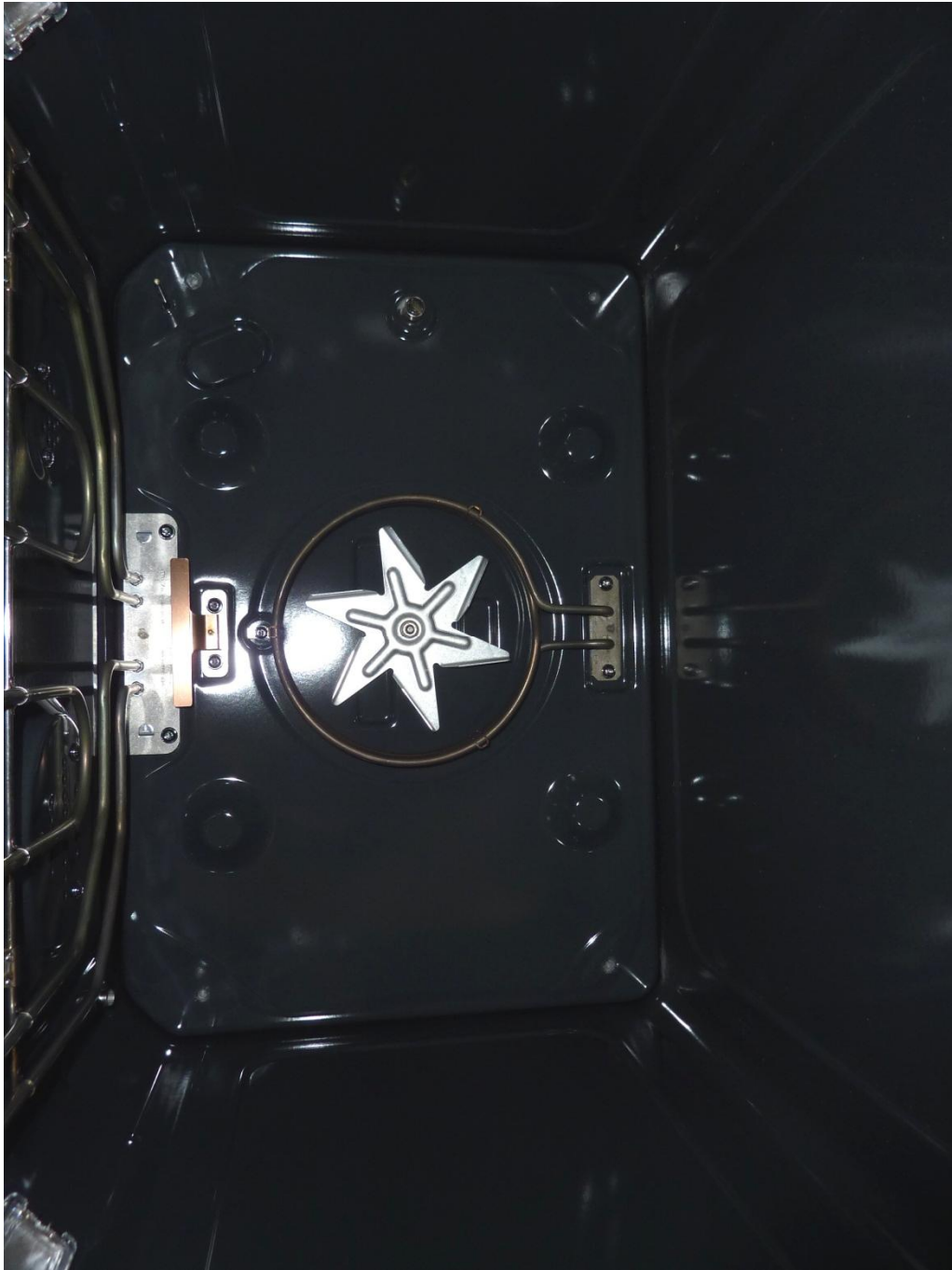
136015_3_a.JPG: EPI7674 inside HR1954, antenna view
