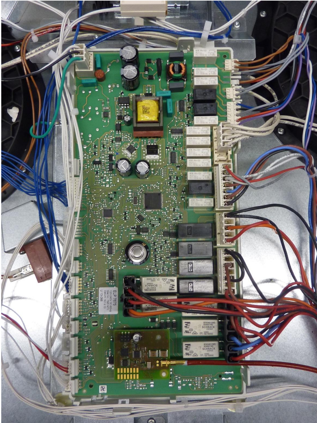
136015_2_h.JPG: EPI7674 inside HR1934, internal view to main PCB
