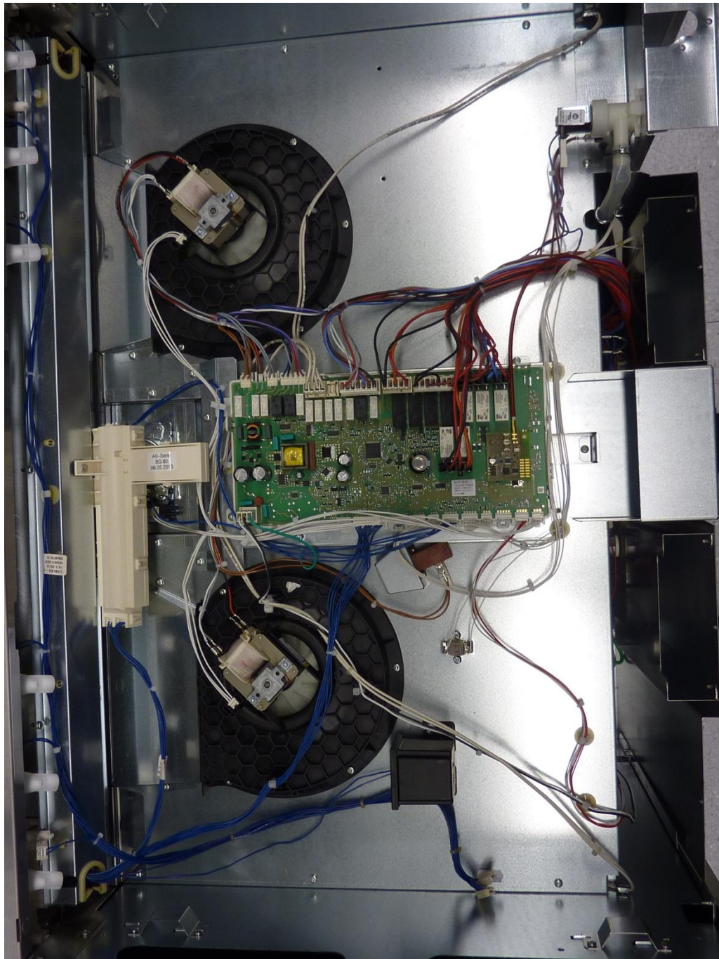
136015_2_i.JPG: EPI7674 inside HR1934, internal view 1 (cover removed)
