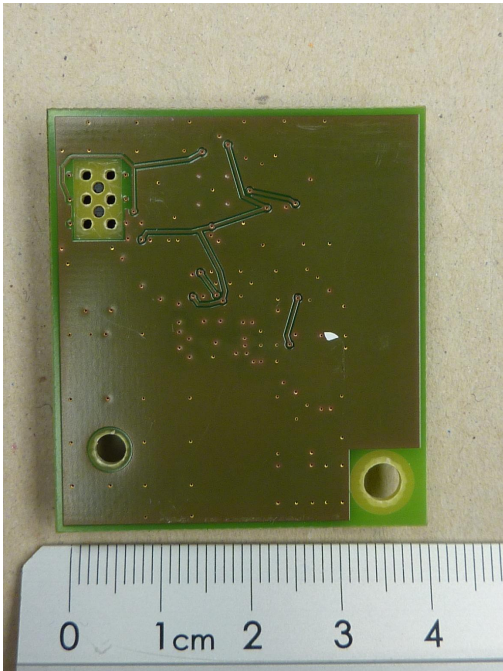
136015_2_d.JPG: EPI7674 bottom view, type plate removed
