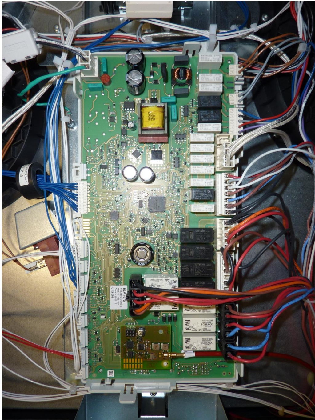
136015_1_j.JPG: EPI7674 inside HR1622, internal view to main PCB
