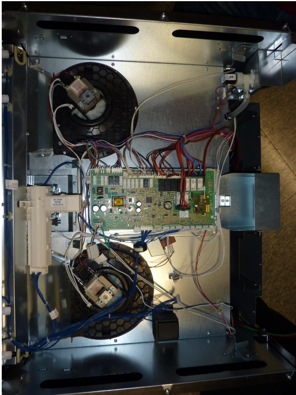
136015_1_k.JPG: EPI7674 inside HR1622, internal view 1 (cover removed)
