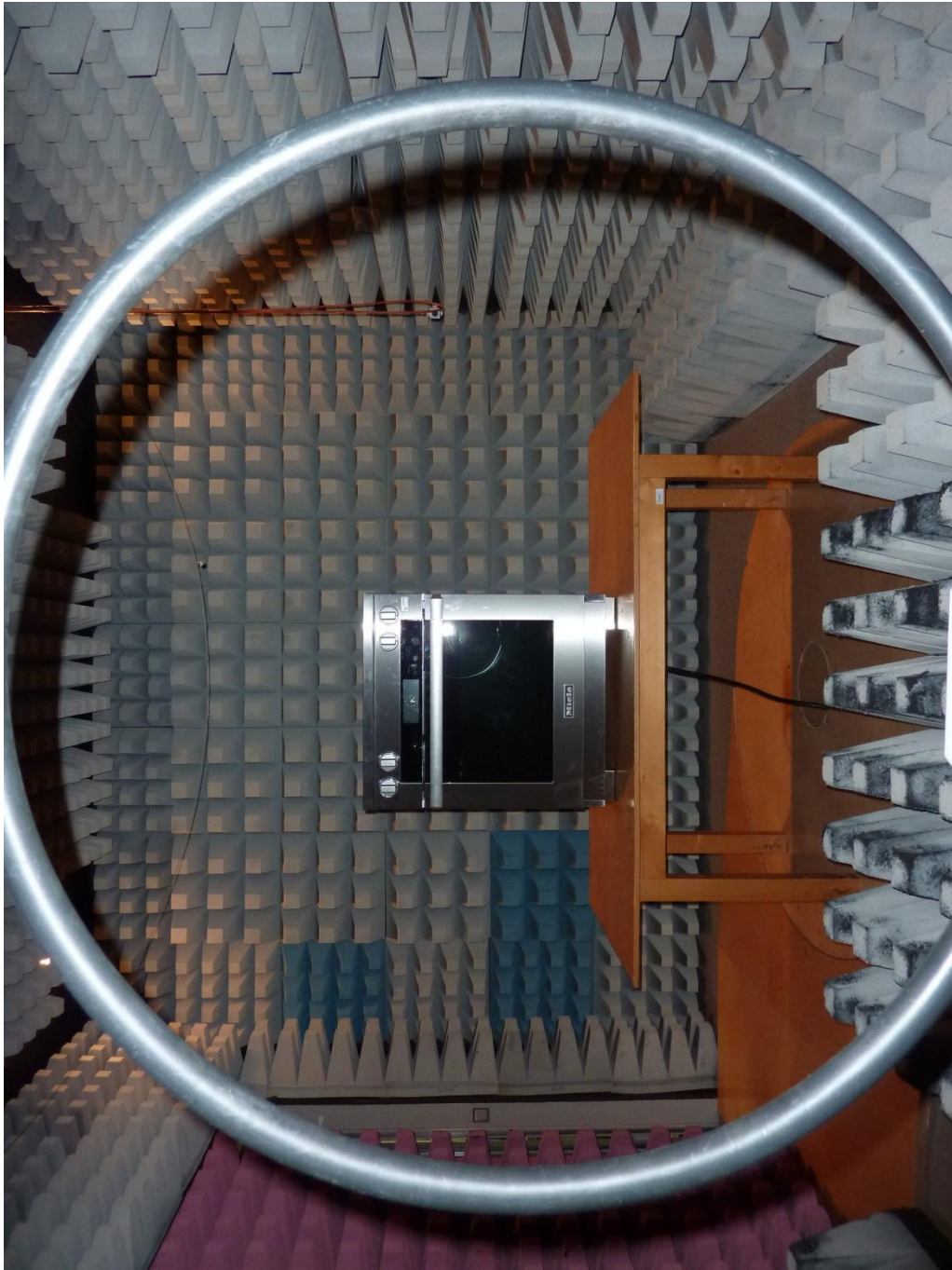
136015_1_4.JPG: EPI7674 inside HR1622, test set-up fully anechoic chamber
