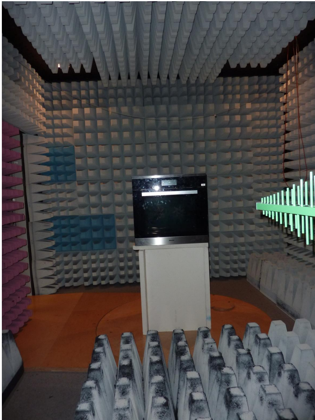
132604_2_1.JPG: EPI7674 inside H6880BP, test set-up fully anechoic chamber
