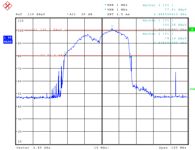
144218_010.wmf: Operation frequency with 135 VAC, 120 ° and 1000 ml load:
