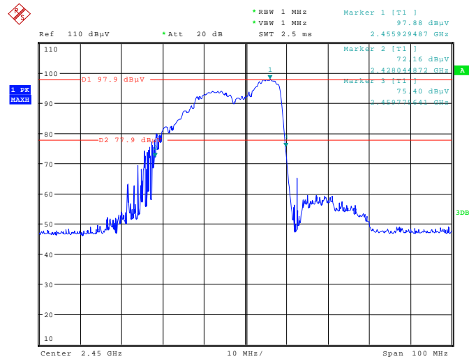
144218_014.wmf: Operation frequency with 96 VAC, 180 ° and 1000 ml load:
