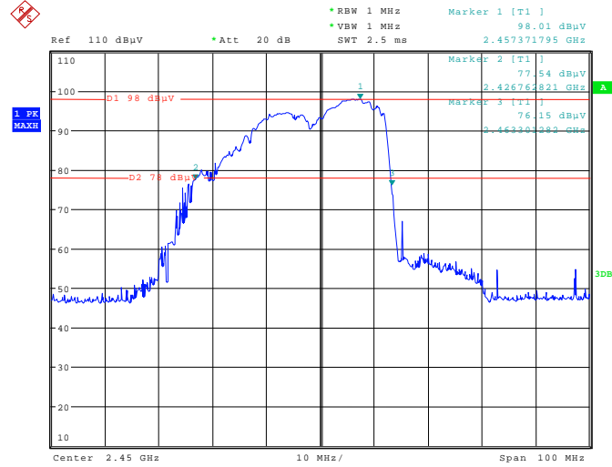
144218_013.wmf: Operation frequency with 108 VAC, 180 ° and 1000 ml load:
