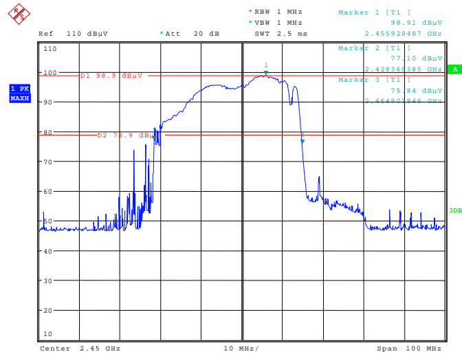
144218_012.wmf: Operation frequency with 120 VAC, 180 ° and 1000 ml load:
