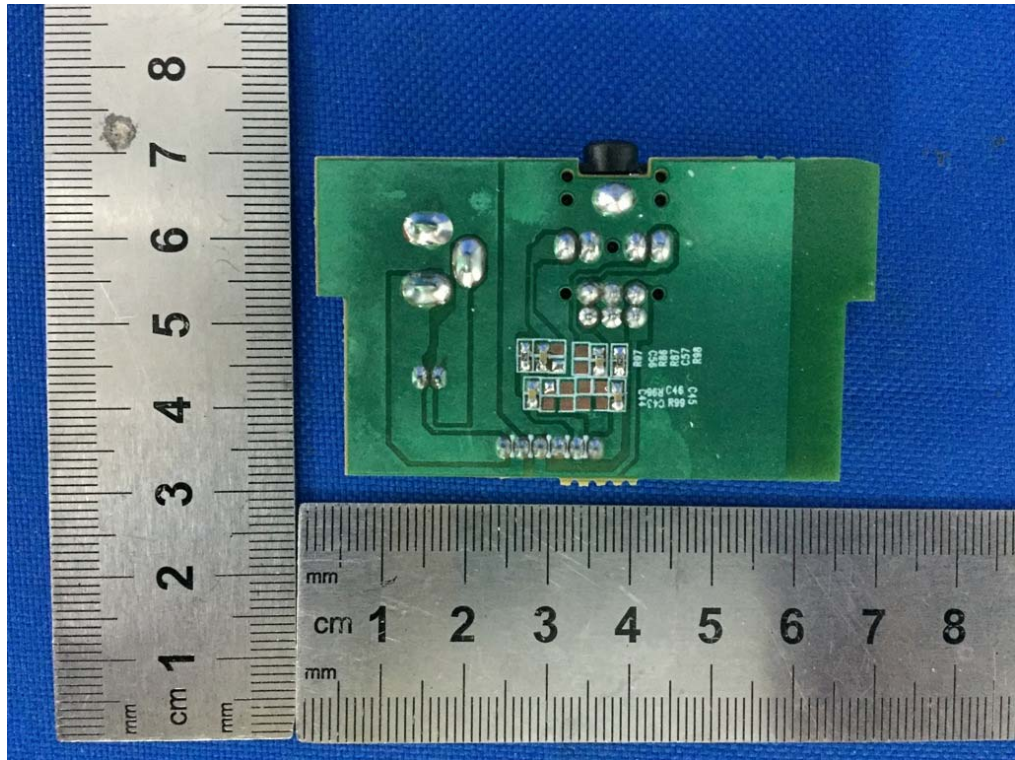
Fig. 13 Trace side view of DC jack board
