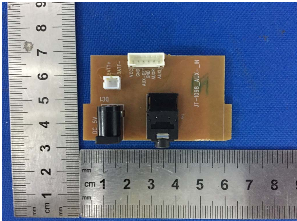
Fig. 14 Component side view of DC jack board
