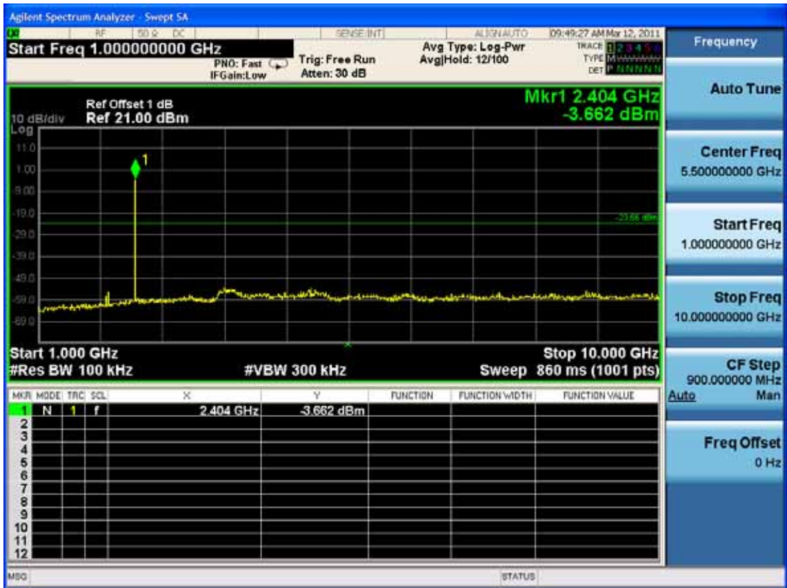
Hopping On 8-DPSK 2402MHz
