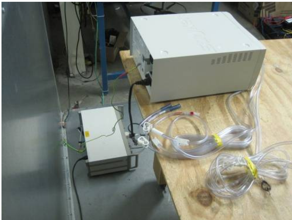
Conducted Emission Test Setup – Rear View
