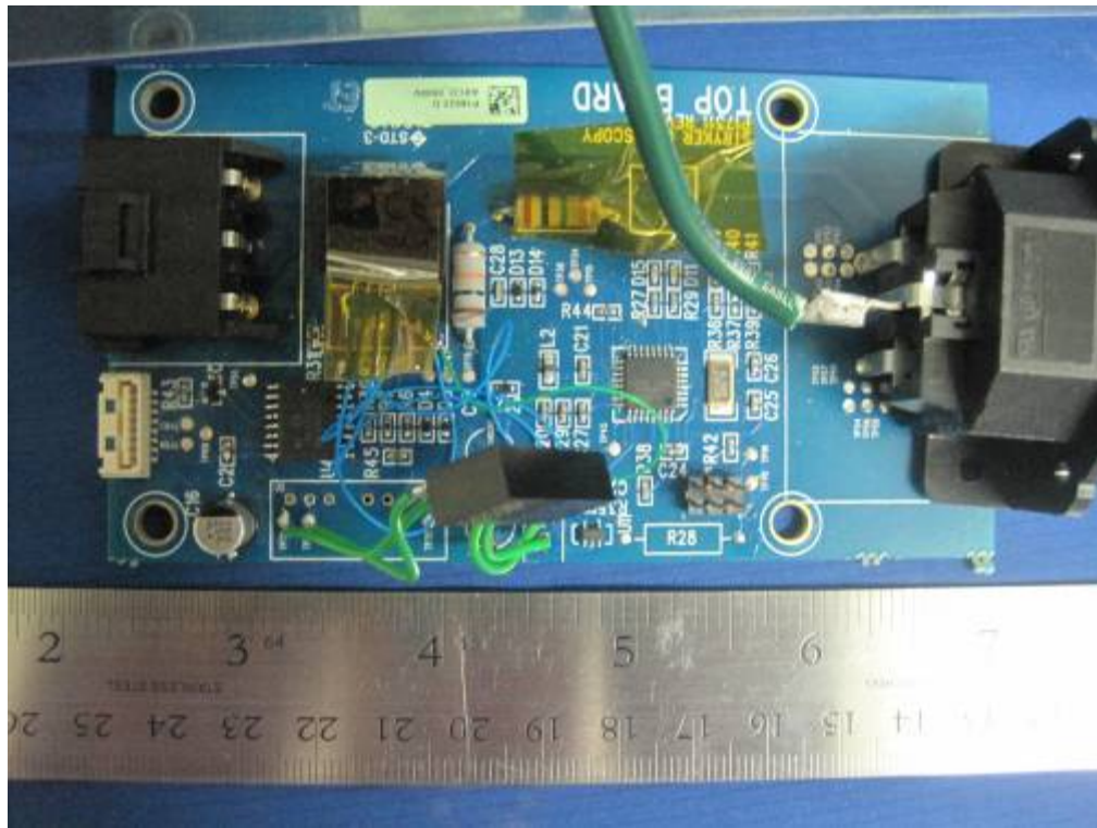
Top Board Top View
