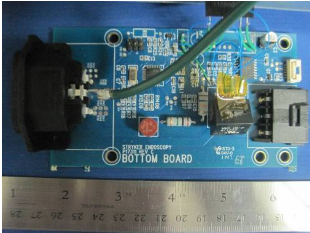
Bottom Board Top View
