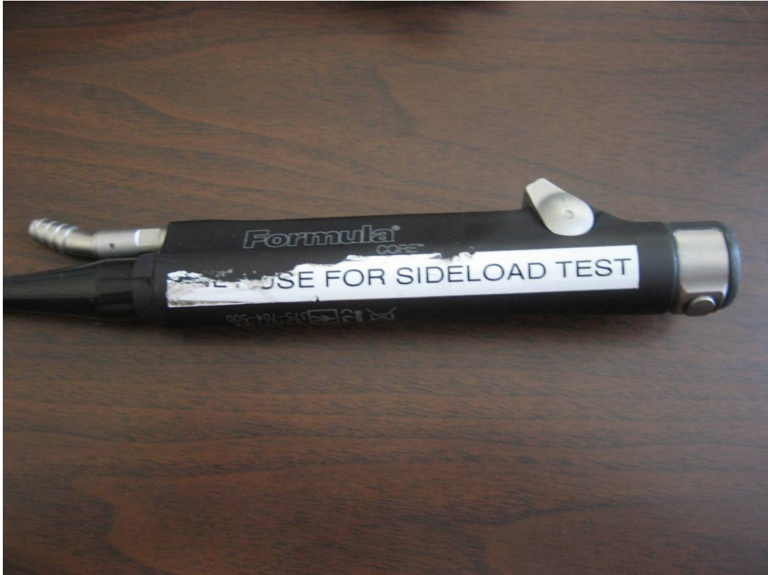
Powered shaver with RFID Antenna
