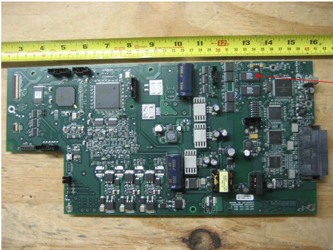
Upper PCB
