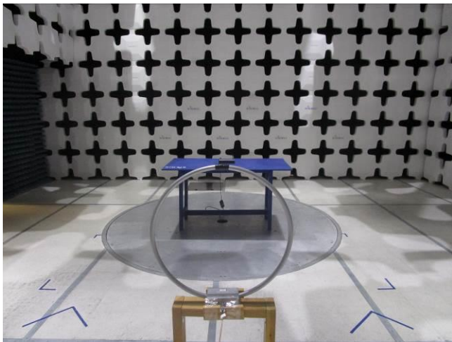
Radiation Emission Test setup (<30MHz) – Front View 0 deg
