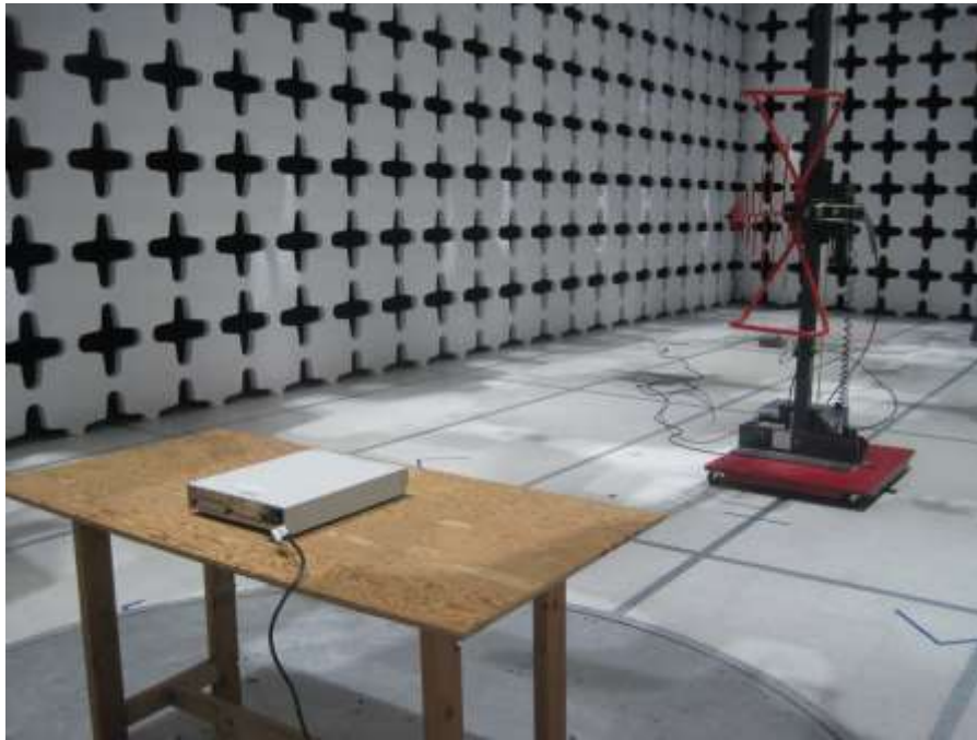
Radiated emissions below 1 GHz setup - Back view
