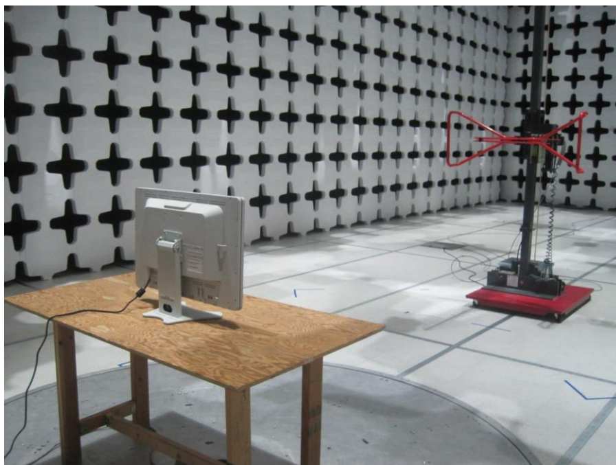
Radiated emissions below 1 GHz setup (With host: wireless LED display) - Back view
