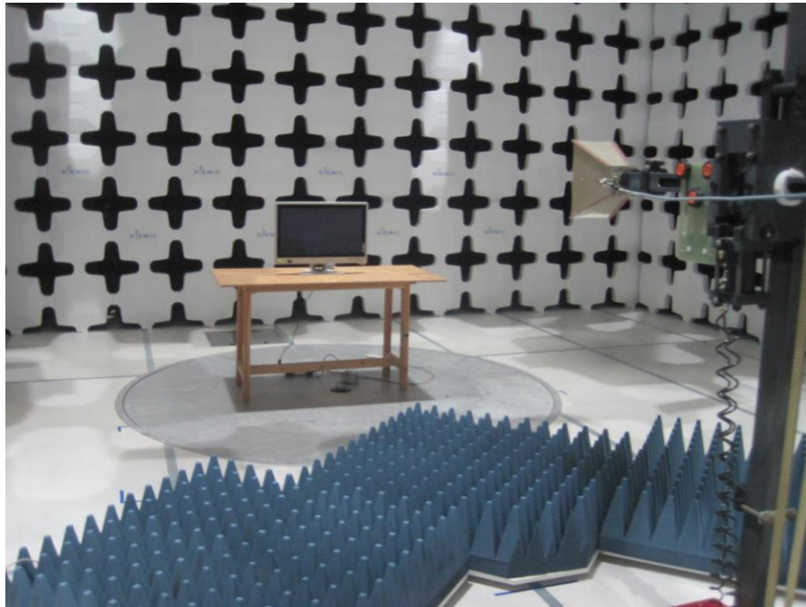
Radiated emissions above than 1 GHz setup (With host: wireless LED display) - Front view
