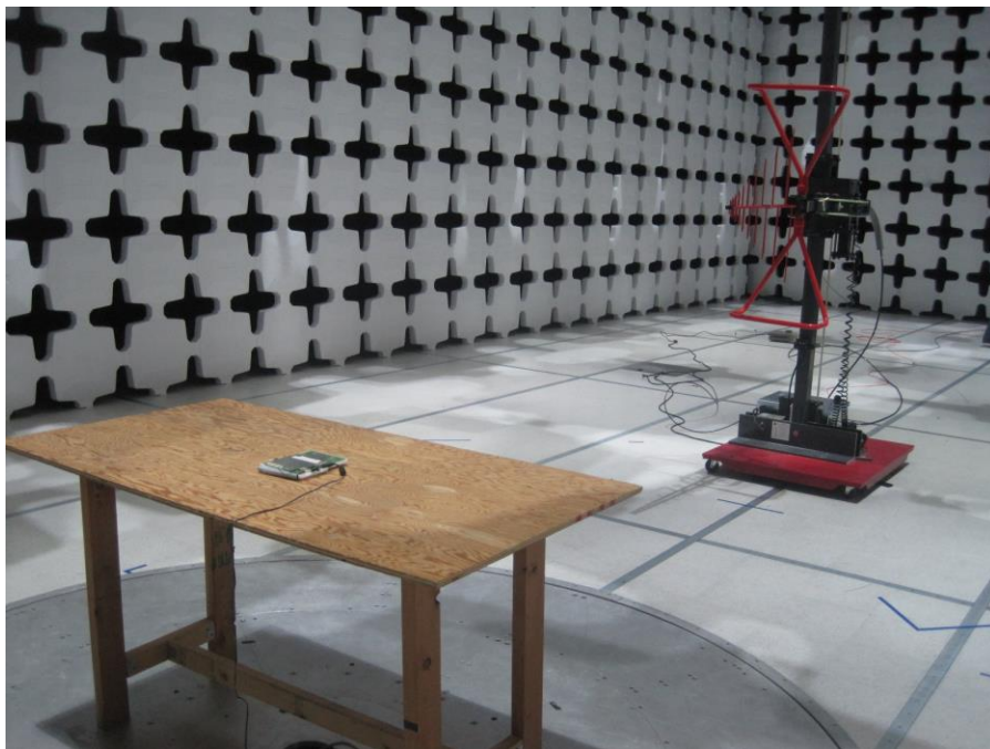
Radiated emissions below 1 GHz setup (Receiver module) - Back view
