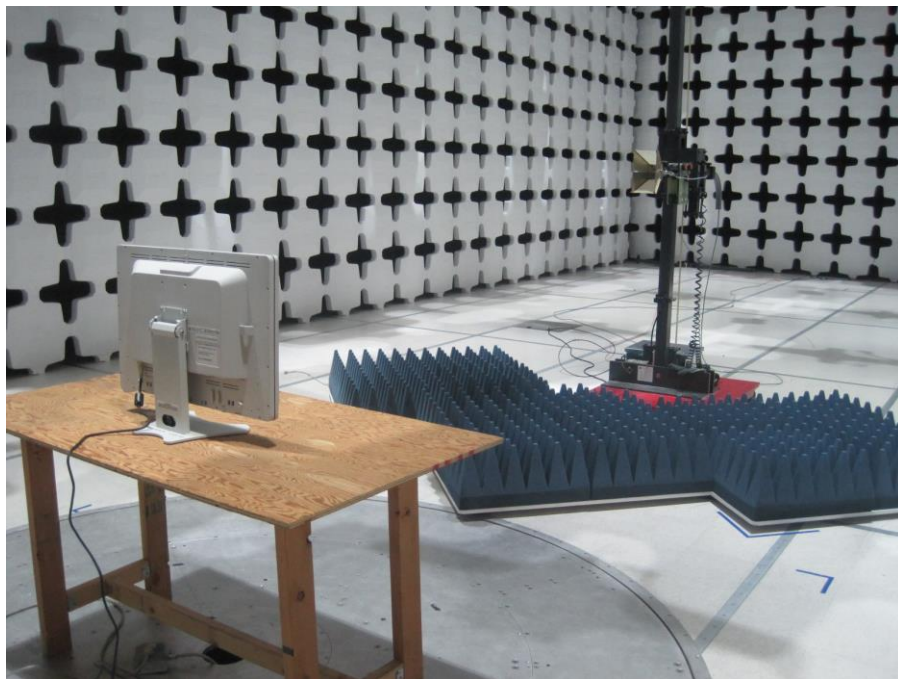
Radiated emissions above than 1 GHz setup (With host: wireless LED display) - Back view
