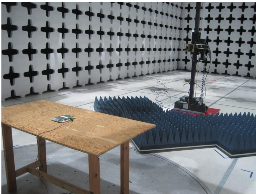
Radiated emissions above than 1 GHz setup (Receiver module) - Back view
