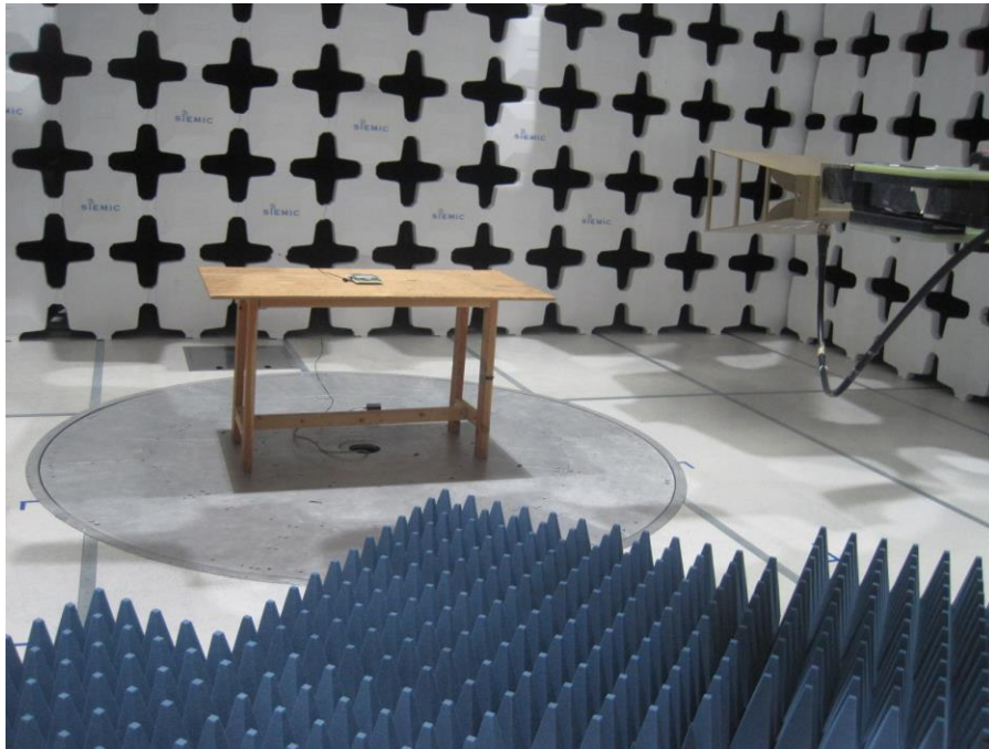
Radiated emissions above than 1 GHz setup (Receiver module) - Front view
