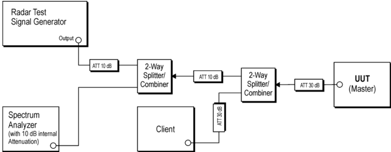
Test Setup Block Diagram
