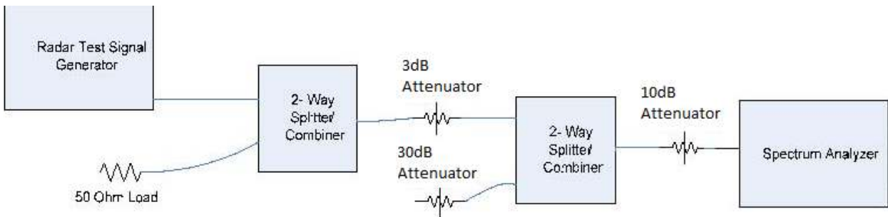
Conducted Calibration Setup
