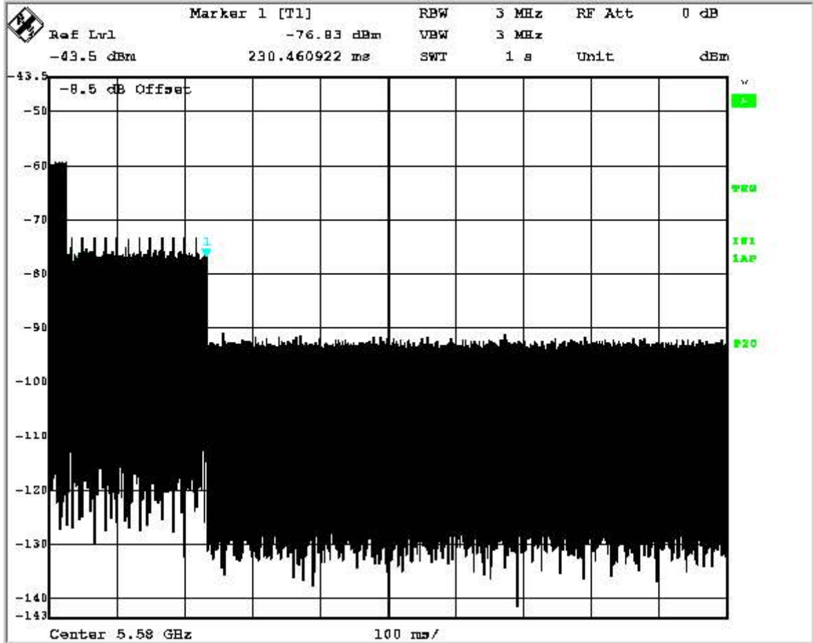
LabiView-Timing Measurement Plot
