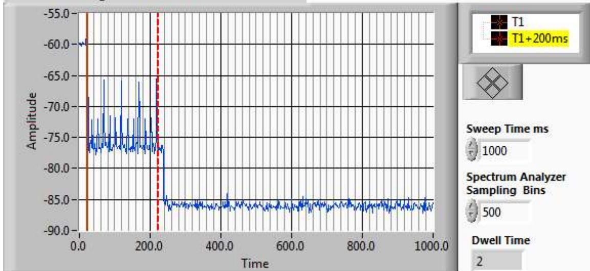
Channel Closing Transmission Time (ms)
