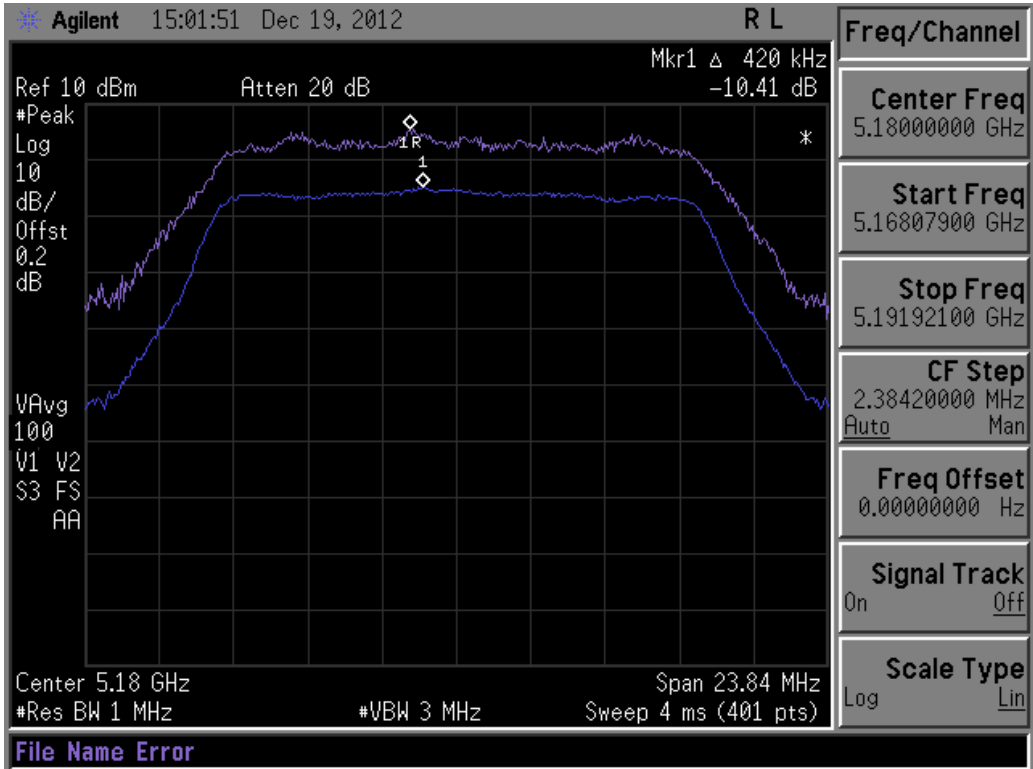
Peak Excursion Ratio TX-Low-Port1-5180
