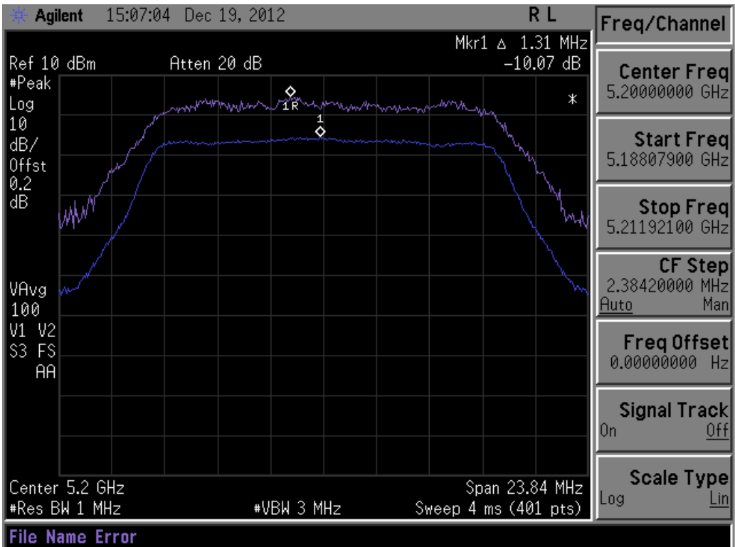
Peak Excursion Ratio TX-Mid-Port1-5200
