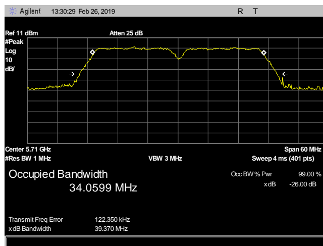
Plot 6. 26 dB Occupied Bandwidth, UNII 2C, 40 MHz, 5710 MHz, J2
