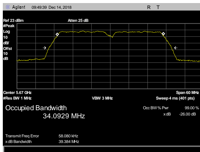
Plot 5. 26 dB Occupied Bandwidth, UNII 2C, 40 MHz, 5670 MHz, J2
