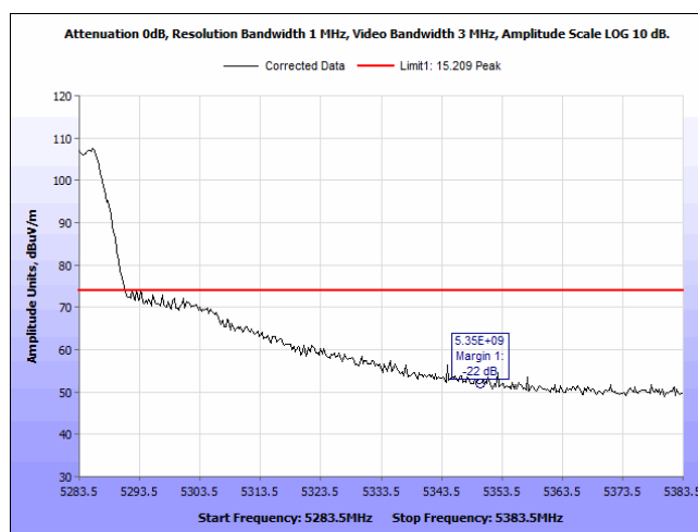
Plot 117. Radiated Band Edge, UNII 2A, Peak, 5350 MHz, BW 40, CF 5270 MHz, rx 11 dBi
