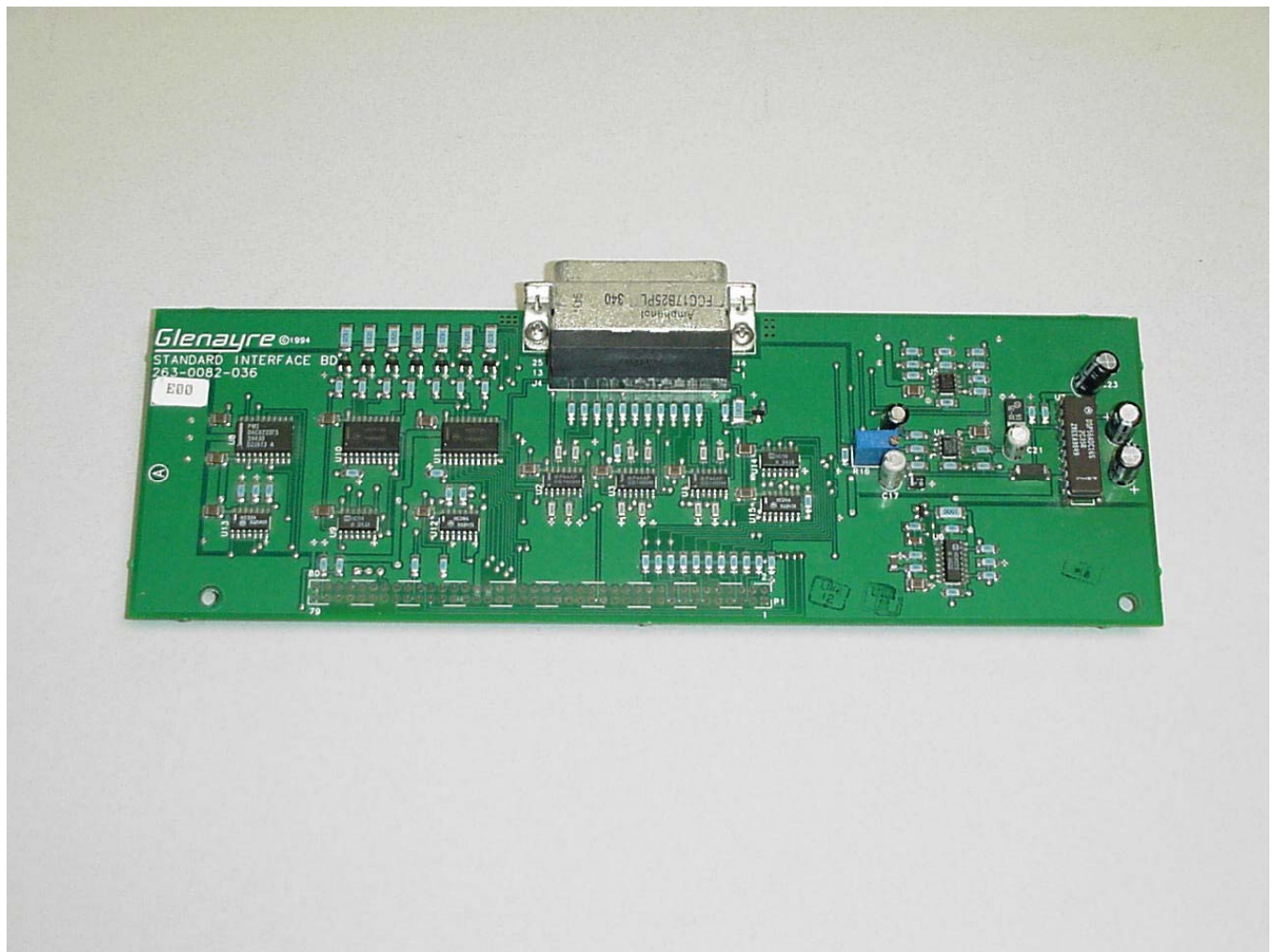
2630082036 Exciter Standard Interface Board (component side)
