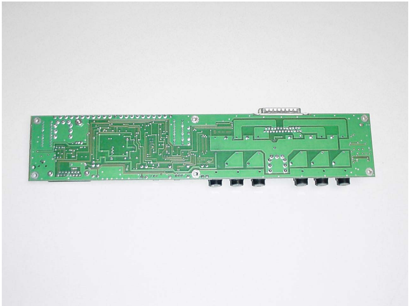
2000.02154 Metering Board (bottom view)
