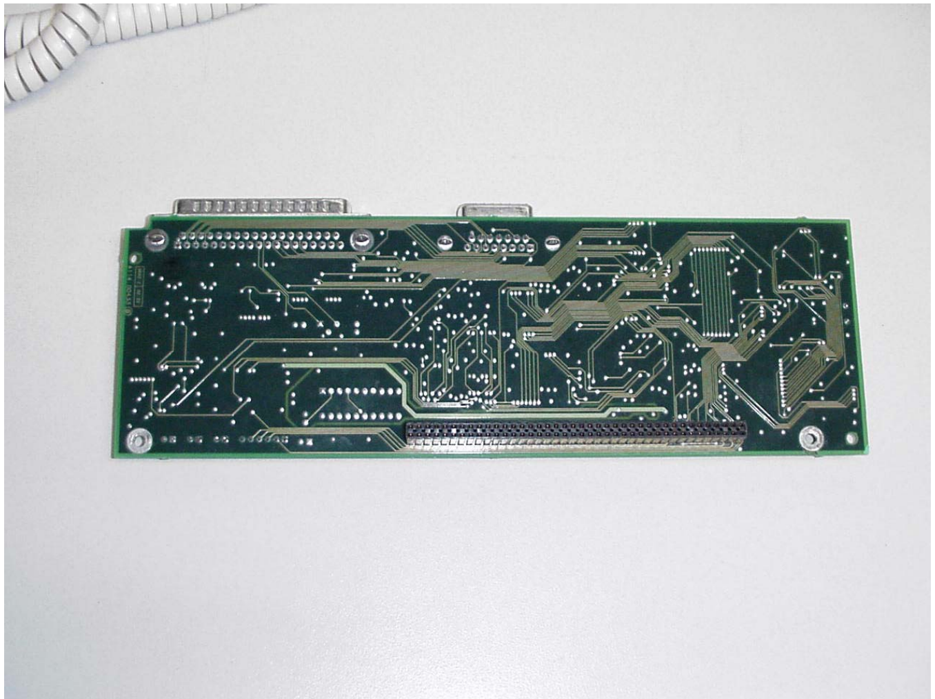
2000.00436 Exciter I20 Interface Board (bottom view)
