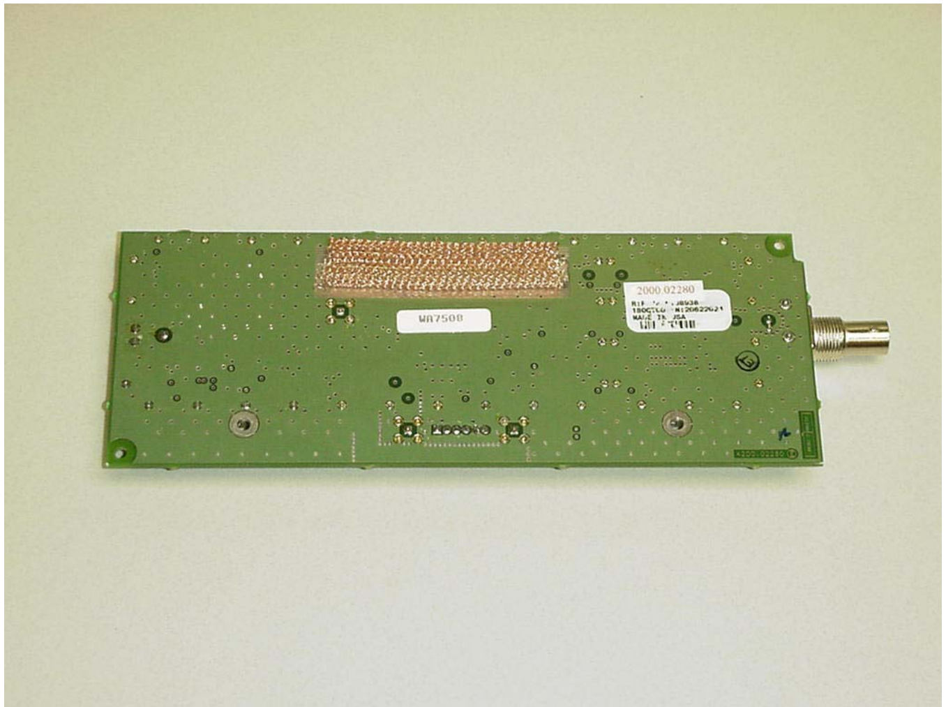
2000.00189 Exciter VCO/RF Amp Board (bottom view)
