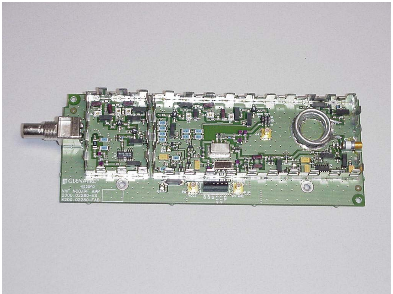
2000.02280 Exciter VCO/RF Amp Board (covers removed)
