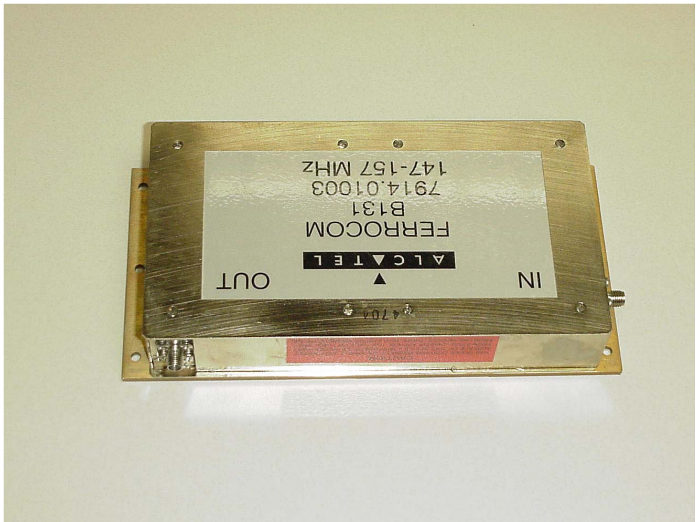
7914.01003 Dual Isolator (far view)
