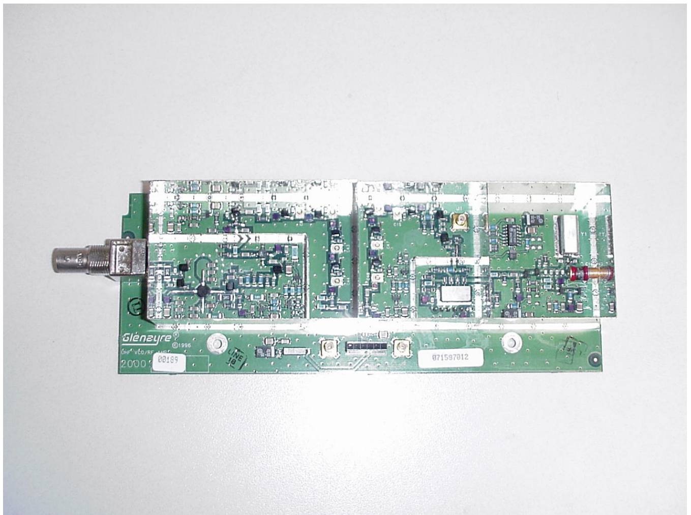
2000.00189 Exciter VCO/RF Amp Board (covers removed)
