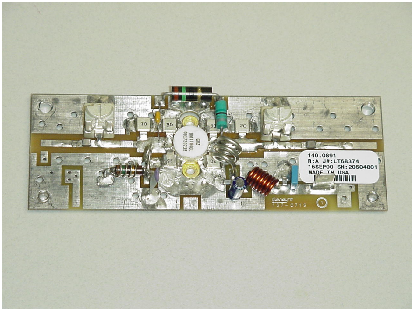
140.0891 RF Final Amplifier Assembly
