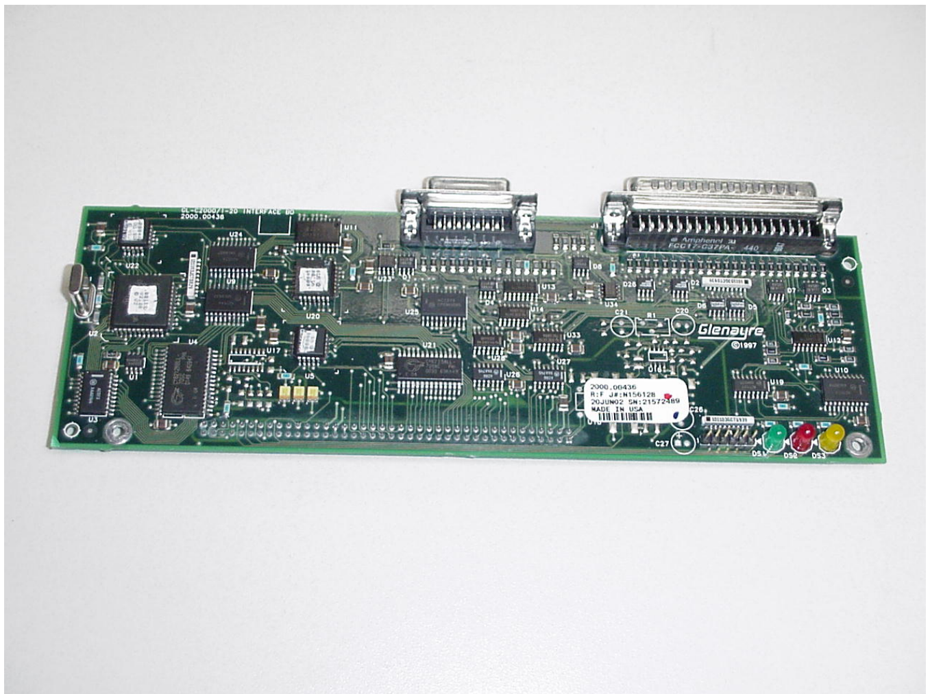
2000.00436 Exciter I20 Interface Board
