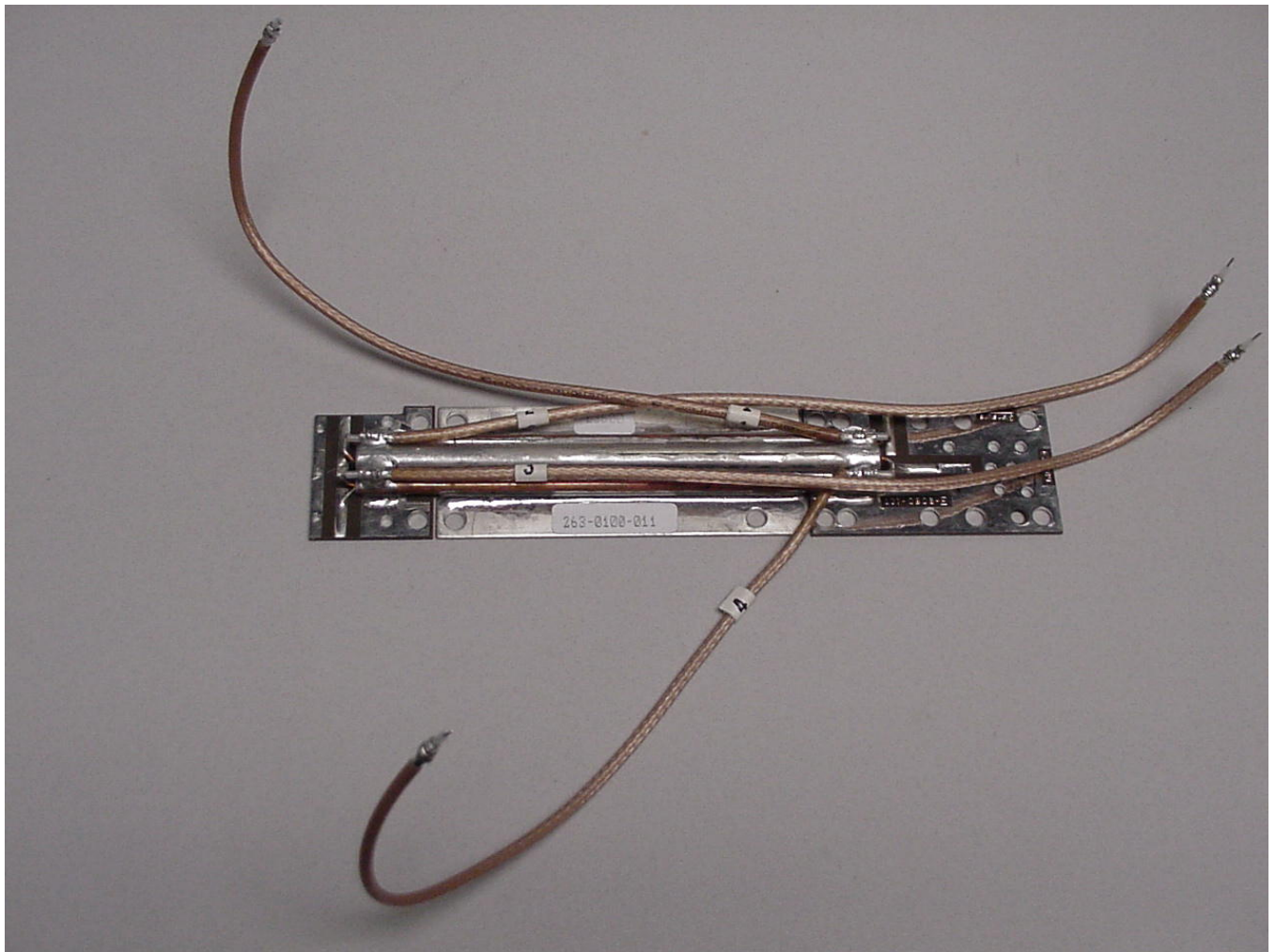
2630100011 Quad RF Combiner Assembly (less chassis mounted resistors)
