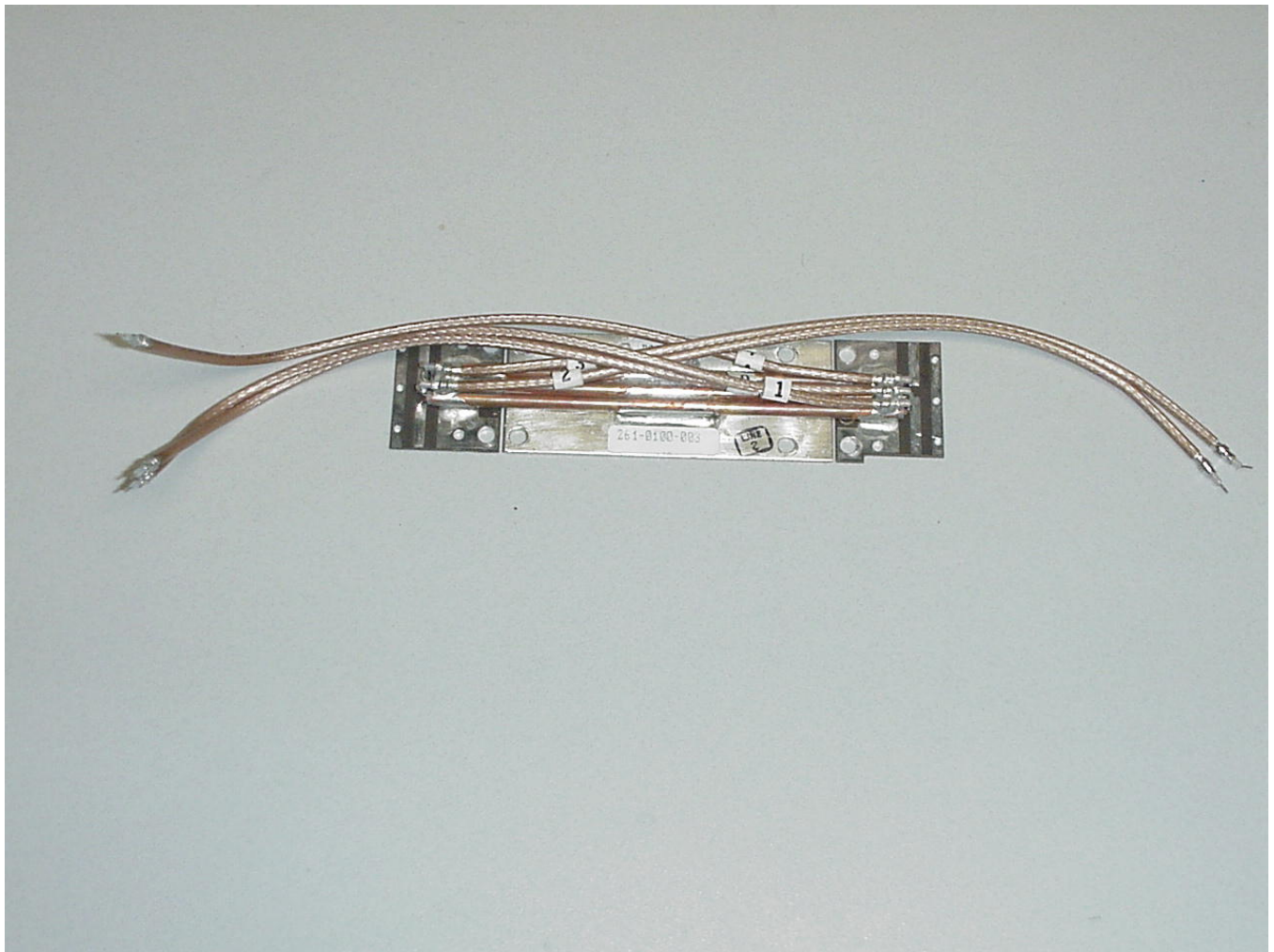
2610100003 Quad RF Splitter Assembly (less chassis mounted resistors)
