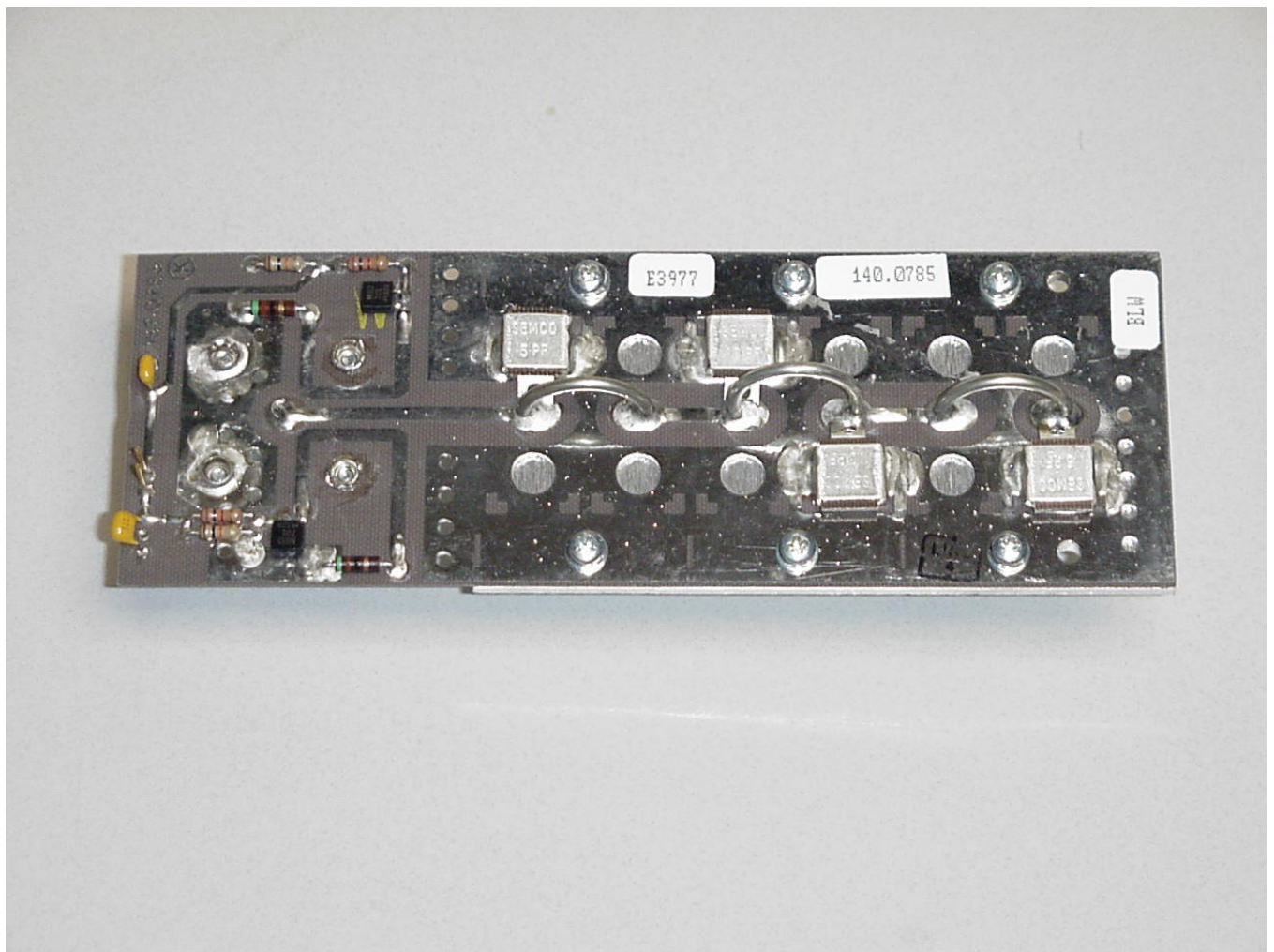
140.0785 Low Pass Filter/Directional Coupler Assembly
