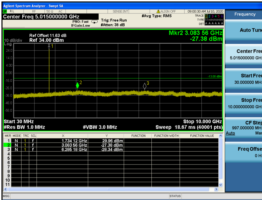
LTE Band 4 / 3MHz / 16QAM - RB Size/Offset (1/14) – Mid Channel
