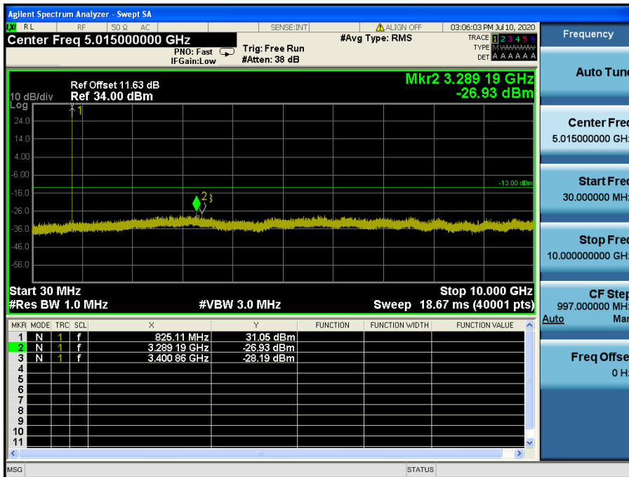
LTE Band 5 / 1.4 MHz / 16QAM - RB Size/Offset (3/3) – Low Channel
