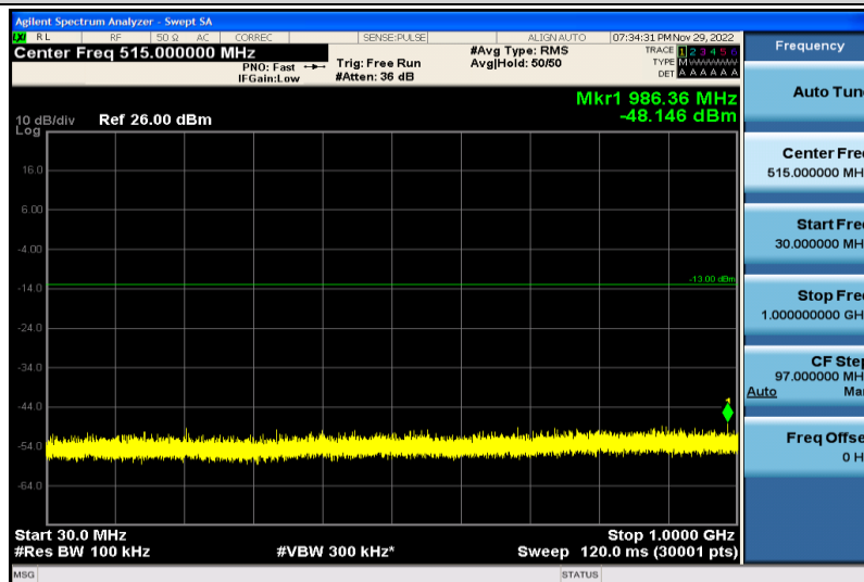
Band66-10MHz-64QAM-132022-1RB#0-30~1000MHz
