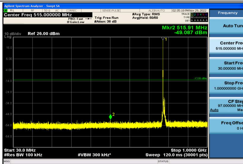
Band13-10MHz-QPSK-23230-1RB#0-30~1000MHz
