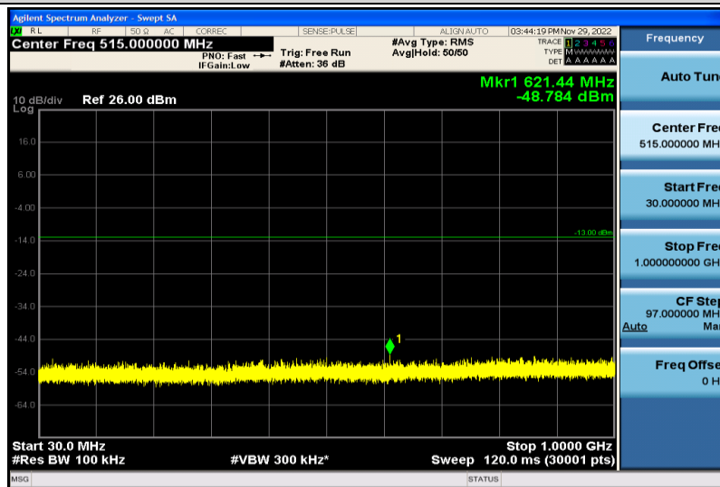
Band66-5MHz-QPSK-131997-1RB#0-30~1000MHz
