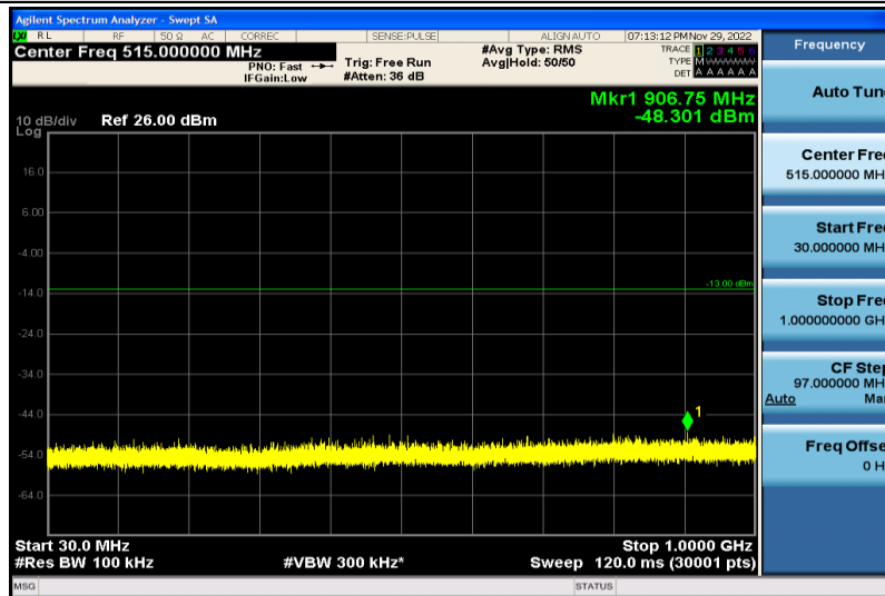
Band66-3MHz-64QAM-131987-1RB#0-30~1000MHz
