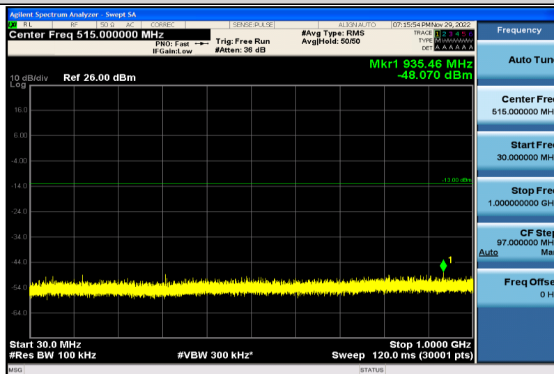
Band66-3MHz-64QAM-132657-1RB#0-30~1000MHz
