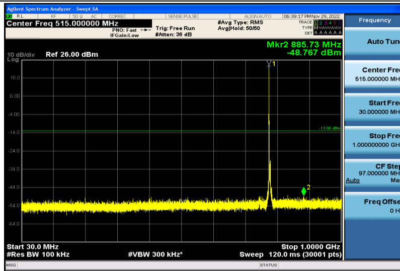
Band13-5MHz-64QAM-23230-1RB#0-30~1000MHz
