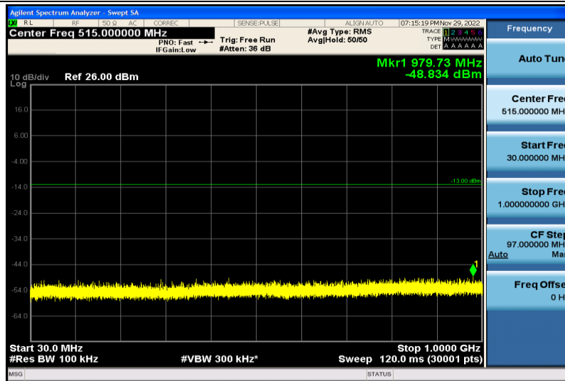
Band66-3MHz-64QAM-132322-1RB#0-30~1000MHz
