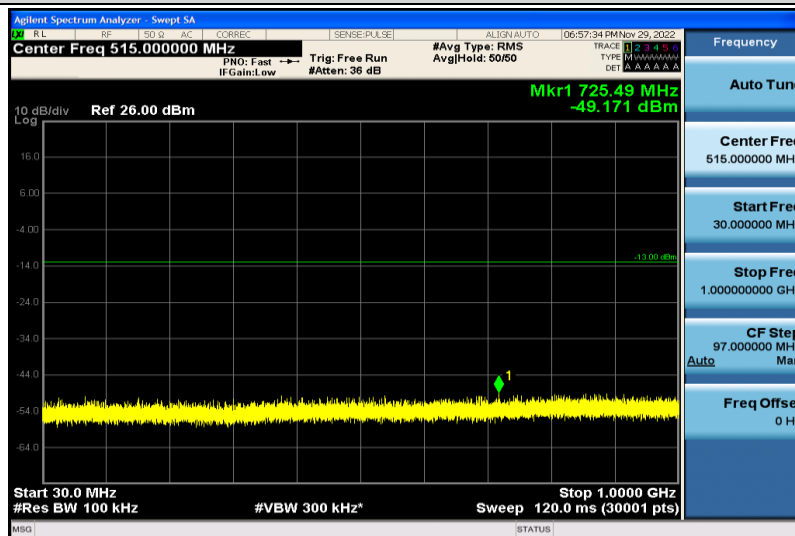
Band66-1.4MHz-64QAM-131979-1RB#0-30~1000MHz
