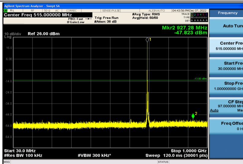
Band12-5MHz-64QAM-23035-1RB#0-30~1000MHz
