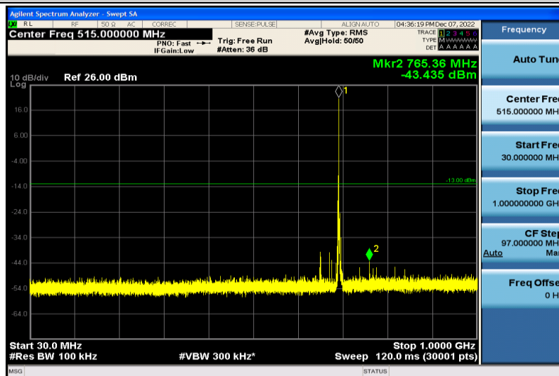
Band12-3MHz-64QAM-23025-1RB#0-30~1000MHz
