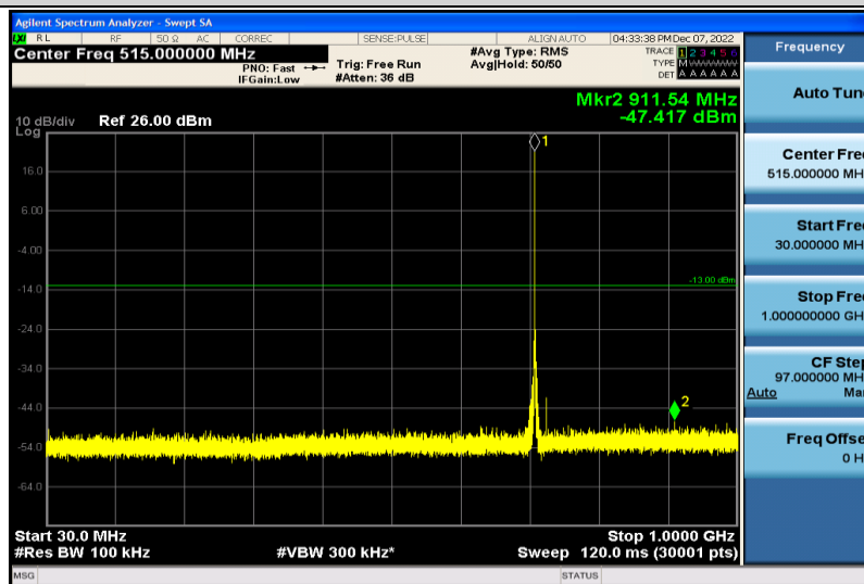
Band12-1.4MHz-64QAM-23173-1RB#0-30~1000MHz
