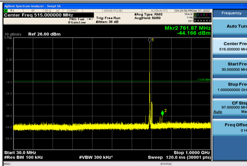
Band12-1.4MHz-64QAM-23017-1RB#0-30~1000MHz
