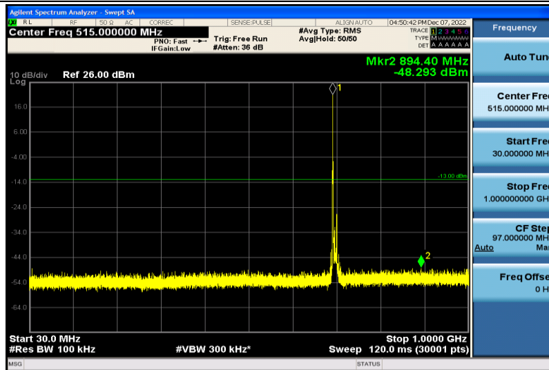
Band12-10MHz-64QAM-23060-1RB#0-30~1000MHz
