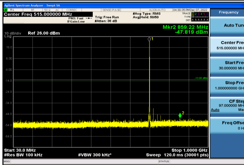
Band12-1.4MHz-QPSK-23095-1RB#0-30~1000MHz
