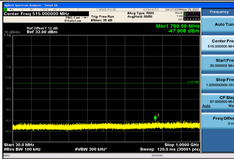
Band4-10MHz-64QAM-20175-1RB#0-30~1000MHz
