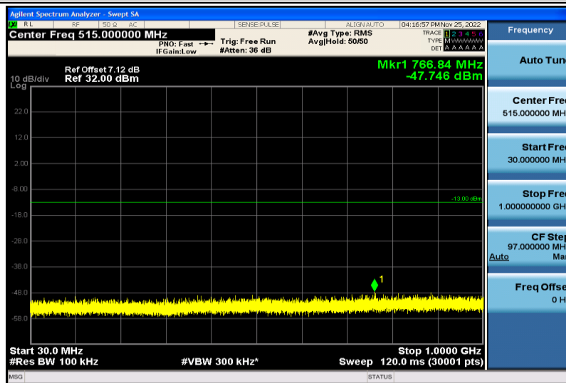
Band4-10MHz-64QAM-20000-1RB#0-30~1000MHz
