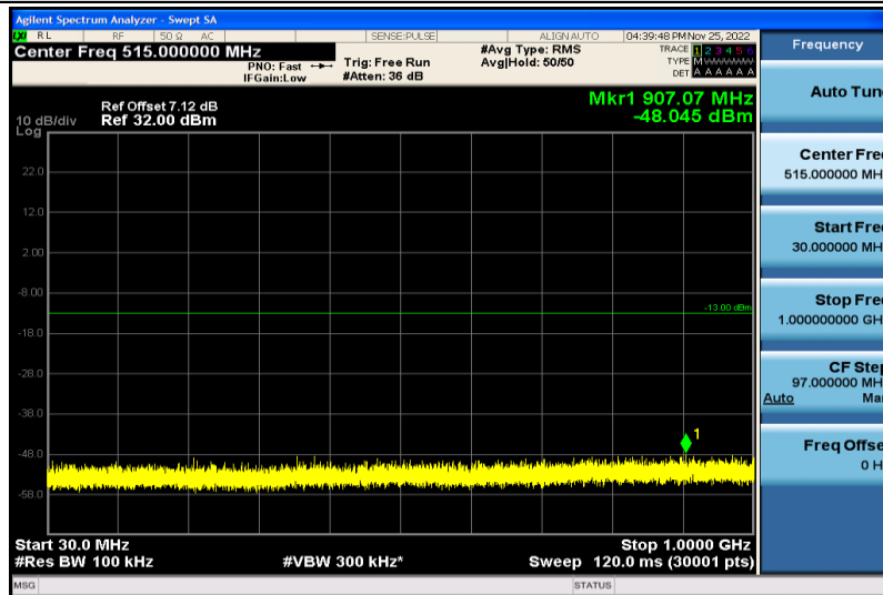
Band4-20MHz-64QAM-20050-1RB#0-30~1000MHz
