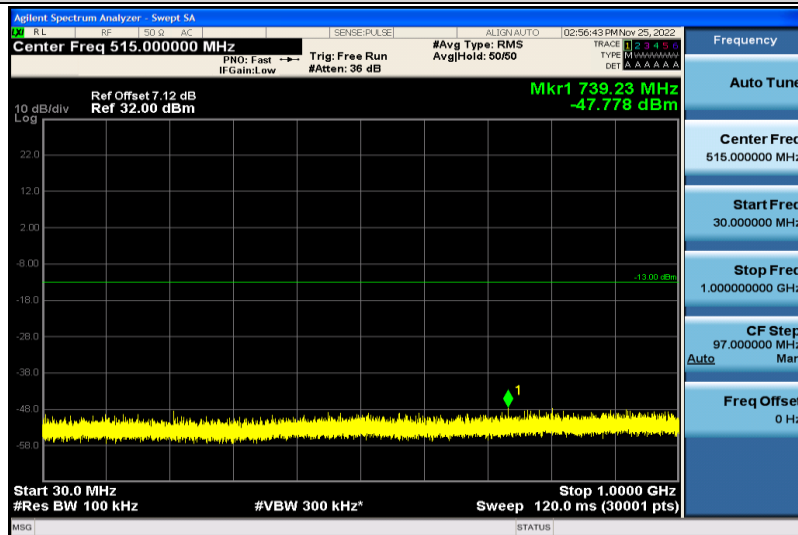
Band2-15MHz-64QAM-19125-1RB#0-30~1000MHz
