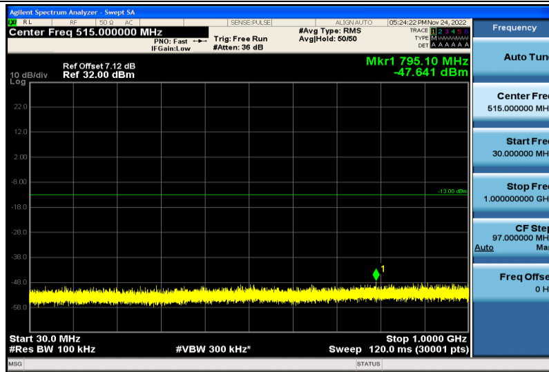
Band4-5MHz-QPSK-20175-1RB#0-30~1000MHz
