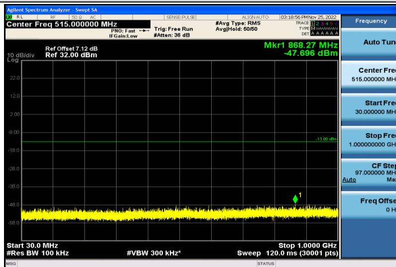
Band4-1.4MHz-64QAM-19957-1RB#0-30~1000MHz
