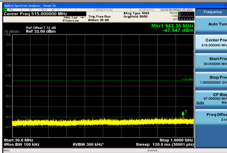
Band4-3MHz-64QAM-19965-1RB#0-30~1000MHz
