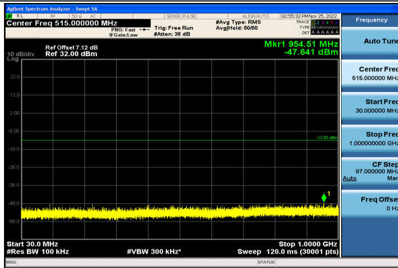
Band2-15MHz-64QAM-18675-1RB#0-30~1000MHz
