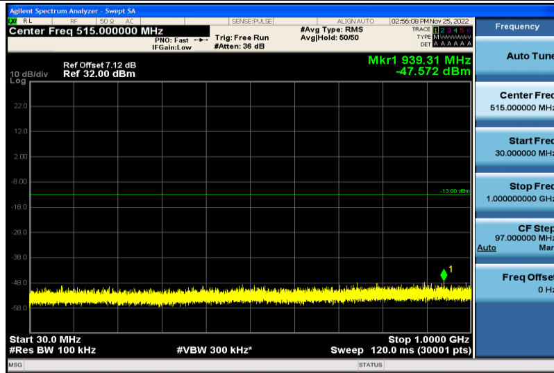
Band2-15MHz-64QAM-18900-1RB#0-30~1000MHz
