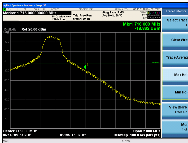
Band12-5MHz-16QAM-23155-1RB#24
