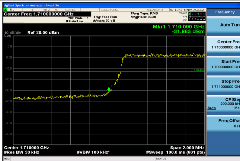
Band66-3MHz-64QAM-131987-15RB#0
