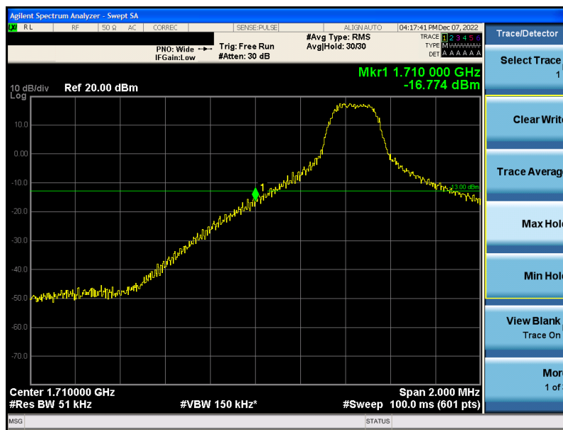
Band66-5MHz-64QAM-131997-1RB#0
