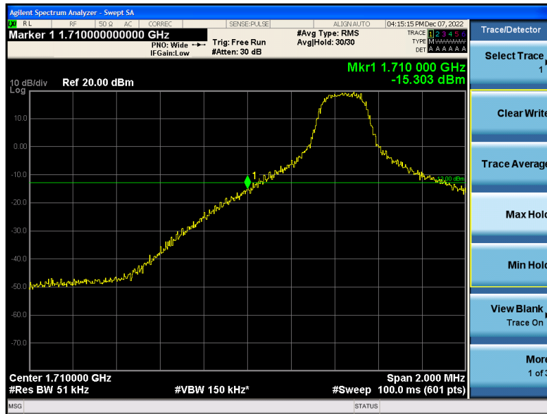
Band66-5MHz-QPSK-131997-1RB#0
