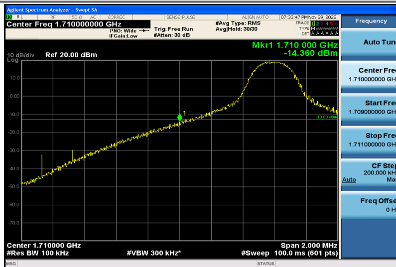
Band66-10MHz-64QAM-132022-1RB#0
