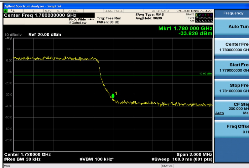
Band66-3MHz-64QAM-132657-15RB#0
