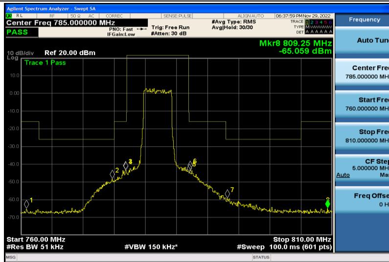
Band13-5MHz-64QAM-23230-25RB#0
