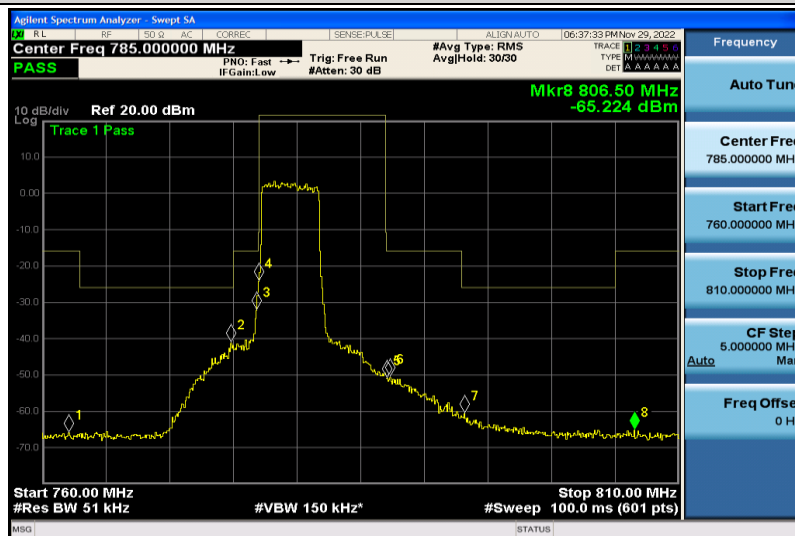
Band13-5MHz-64QAM-23205-25RB#0
