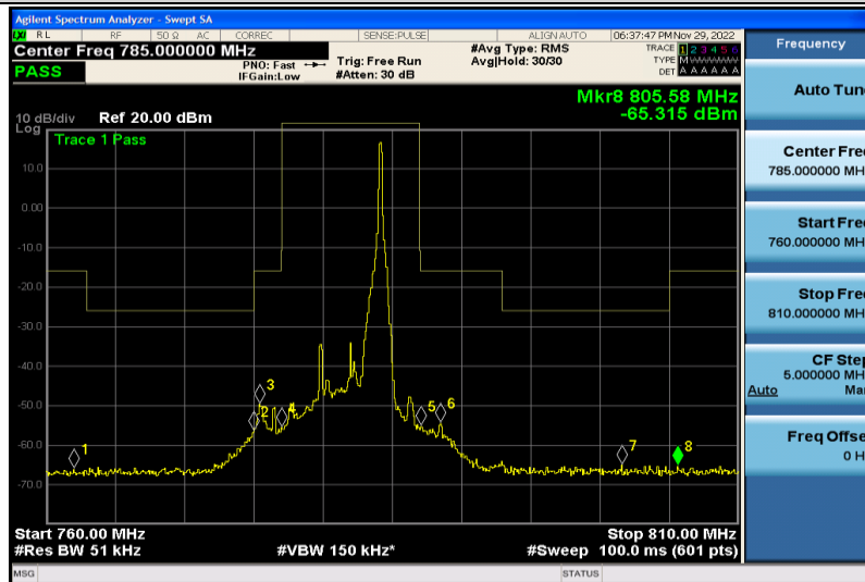
Band13-5MHz-64QAM-23230-1RB#24
