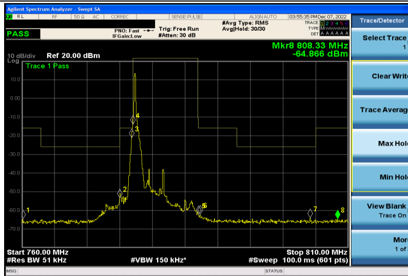
Band13-5MHz-64QAM-23205-1RB#0
