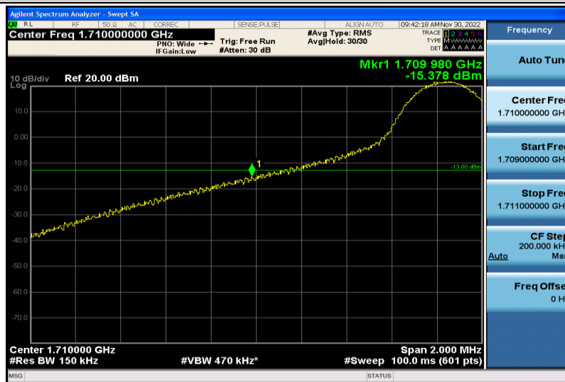
Band66-15MHz-64QAM-132047-1RB#0
