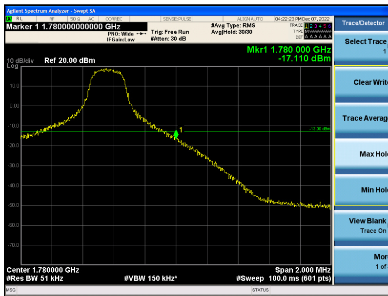
Band66-5MHz-16QAM-132647-1RB#24
