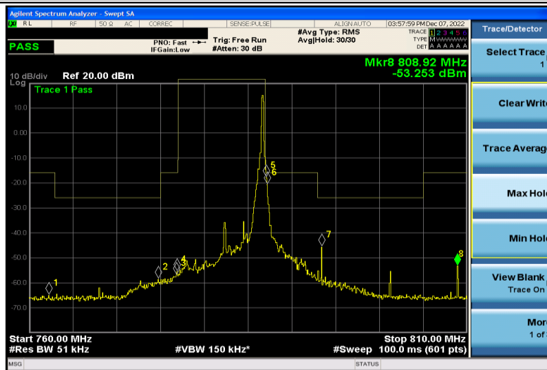
Band13-5MHz-QPSK-23255-1RB#24
