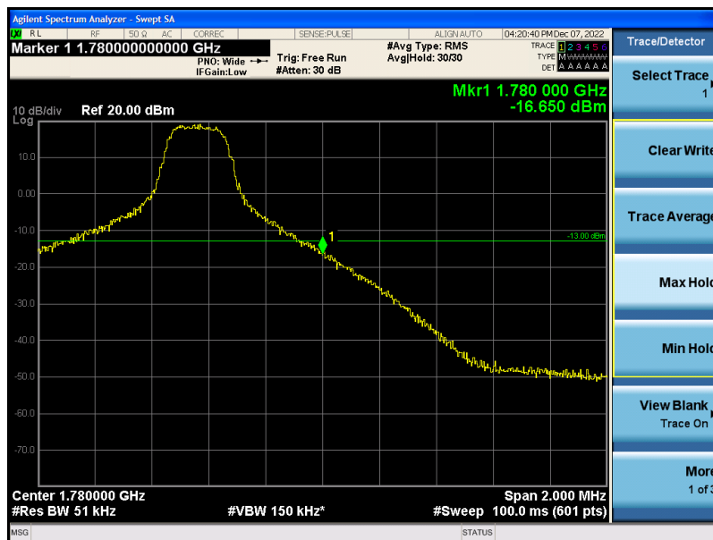
Band66-5MHz-QPSK-132647-1RB#24
