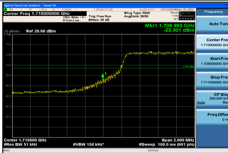
Band66-5MHz-64QAM-131997-25RB#0
