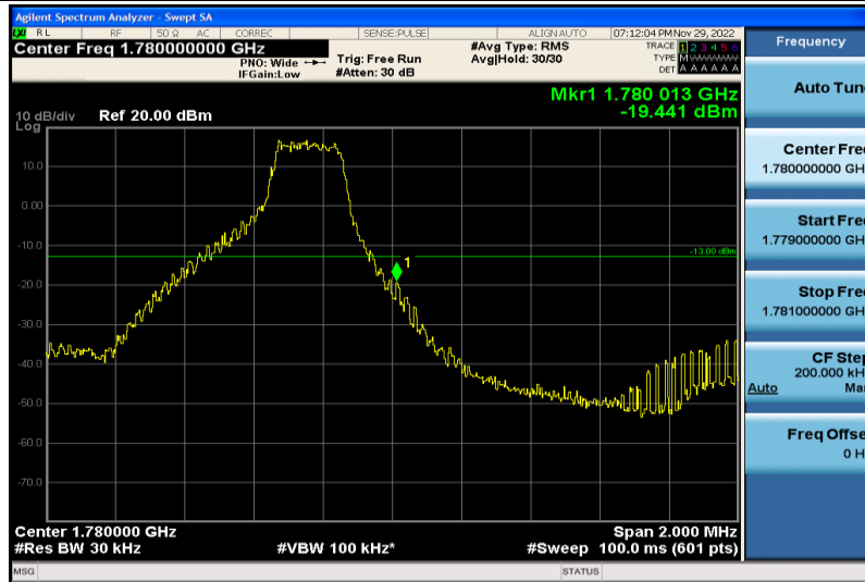
Band66-3MHz-64QAM-132657-1RB#14
