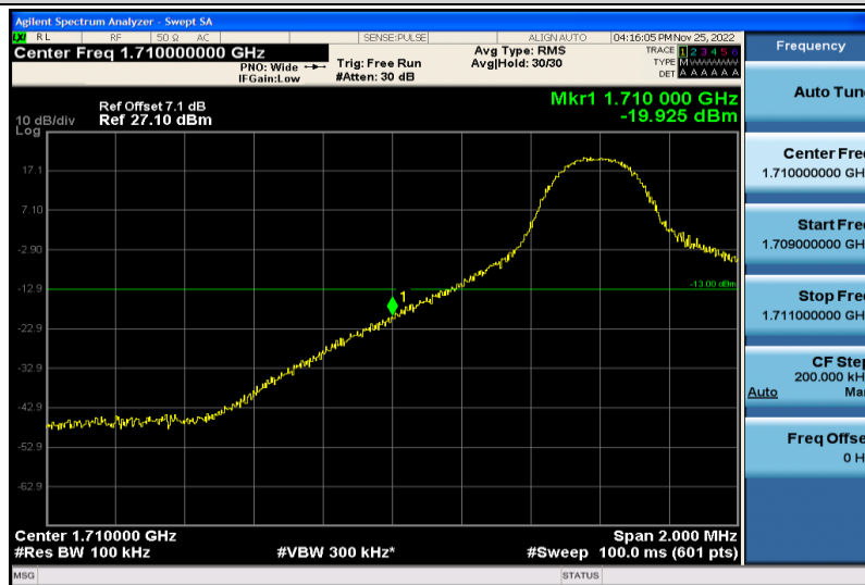
Band4-10MHz-64QAM-20000-1RB#0
