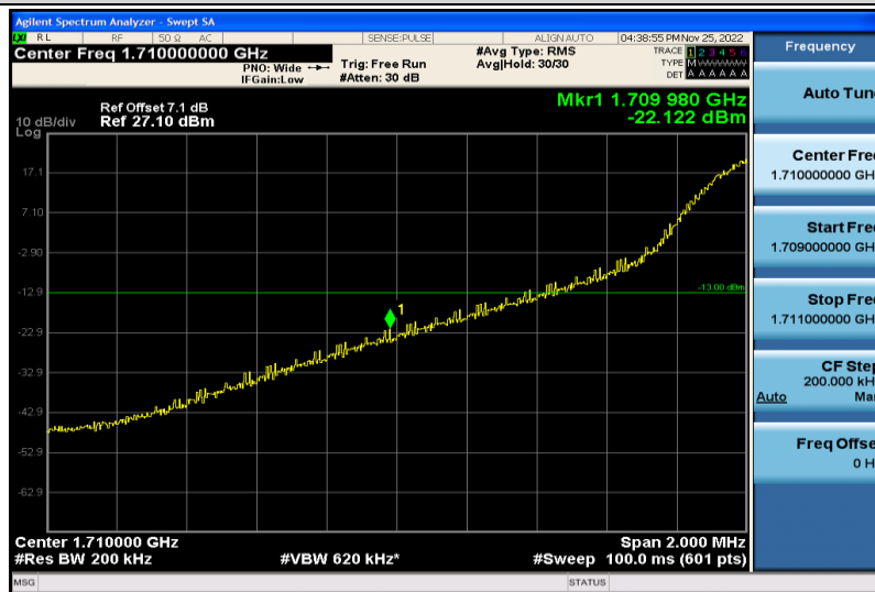
Band4-20MHz-64QAM-20050-1RB#0
