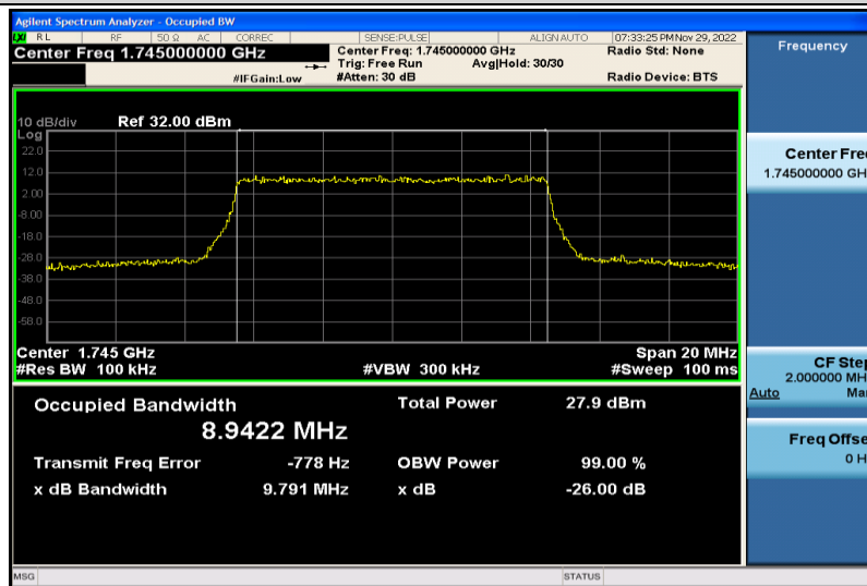
Band66-10MHz-64QAM-132322-50RB#0-8.9422
