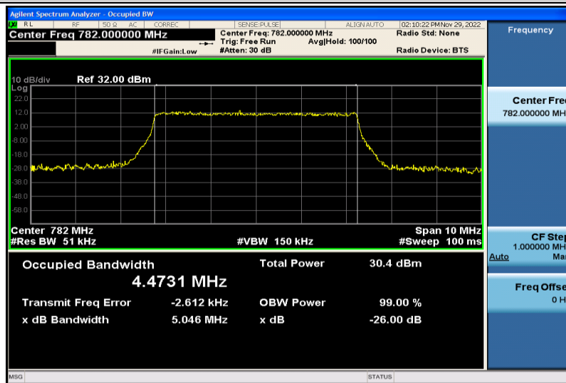
Band13-5MHz-QPSK-23230-25RB#0-4.4731
