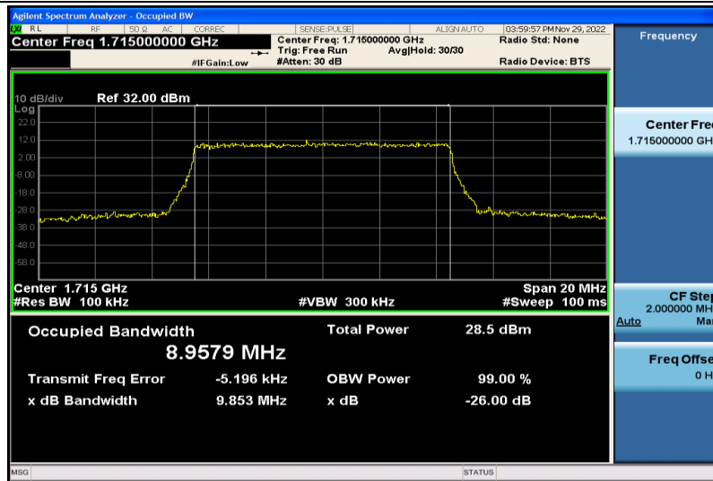
Band66-10MHz-16QAM-132022-50RB#0-8.9579
