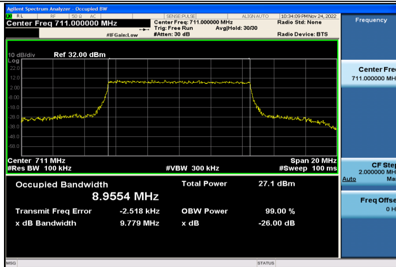
Band12-10MHz-16QAM-23130-50RB#0-8.9554
