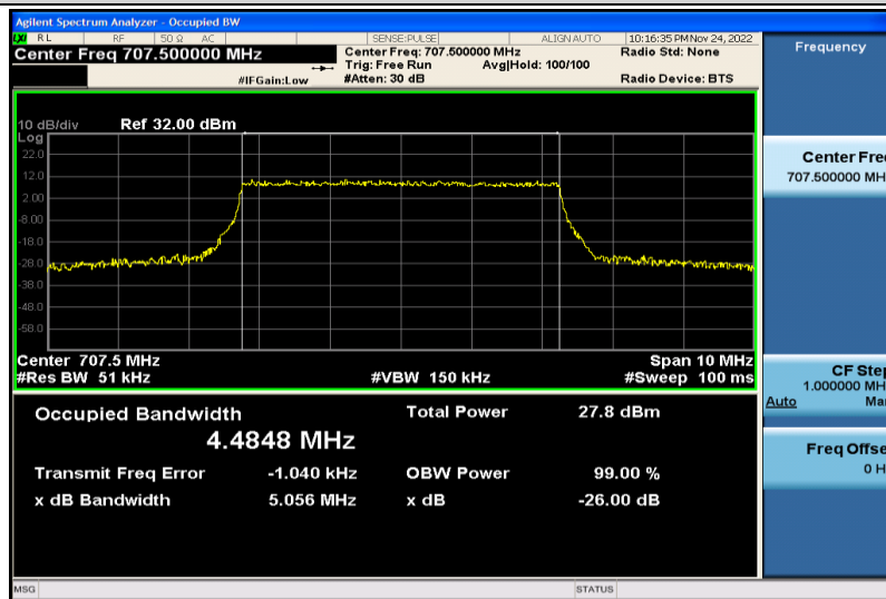
Band12-5MHz-QPSK-23095-25RB#0-4.4848
