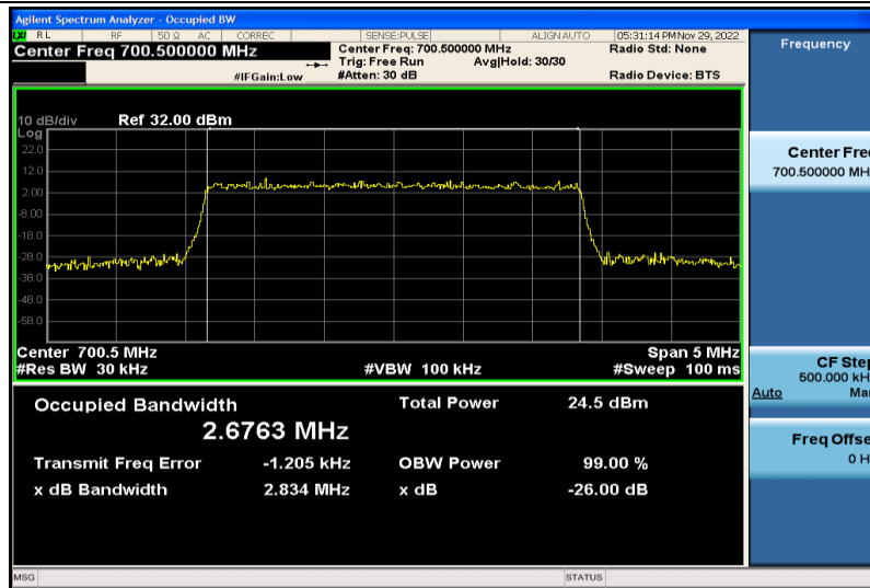
Band12-3MHz-64QAM-23025-15RB#0-2.6763
