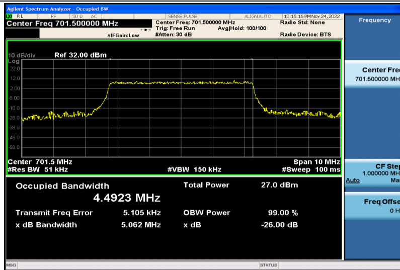
Band12-5MHz-16QAM-23035-25RB#0-4.4923
