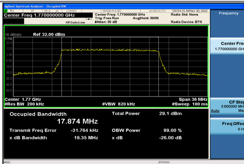
Band66-20MHz-64QAM-132572-100RB#0-17.874
