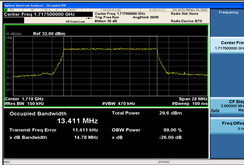
Band66-15MHz-QPSK-132047-75RB#0-13.411
