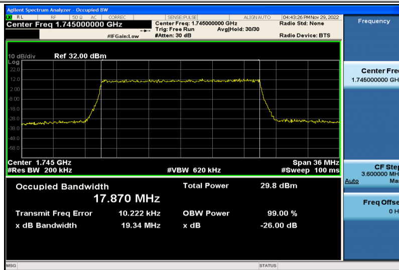
Band66-20MHz-QPSK-132322-100RB#0-17.870
