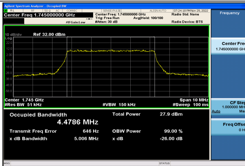
Band66-5MHz-64QAM-132322-25RB#0-4.4786
