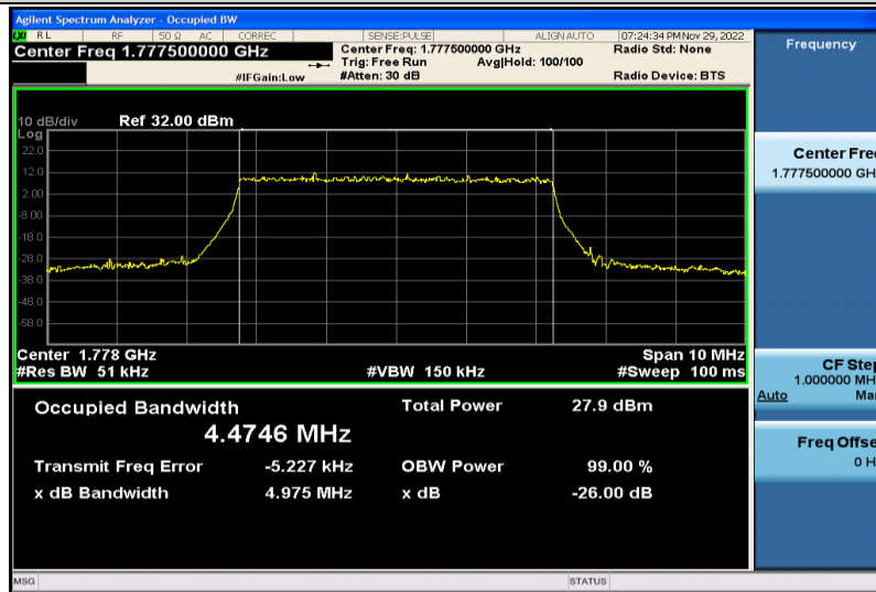
Band66-5MHz-64QAM-132647-25RB#0-4.4746
