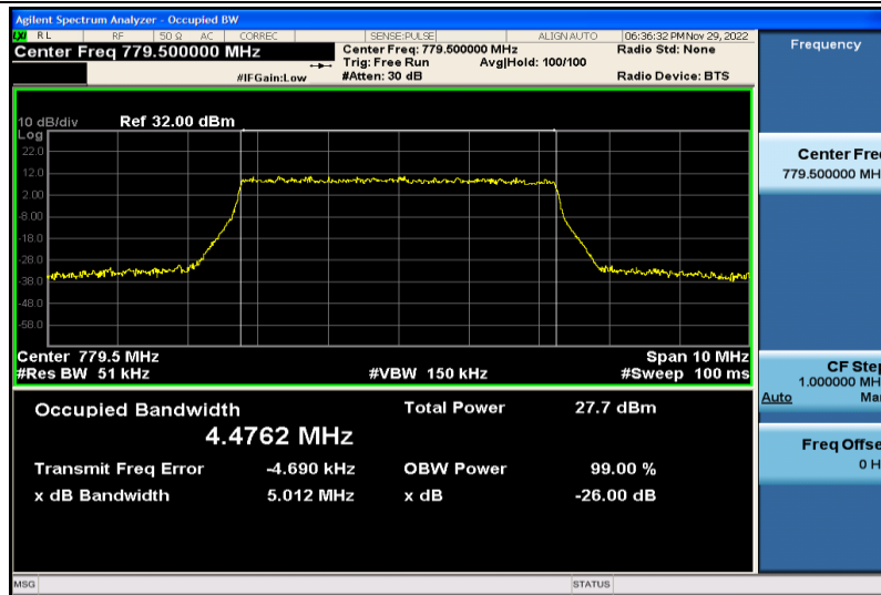
Band13-5MHz-64QAM-23205-25RB#0-4.4762
