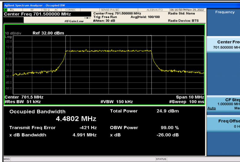
Band12-5MHz-64QAM-23035-25RB#0-4.4802
