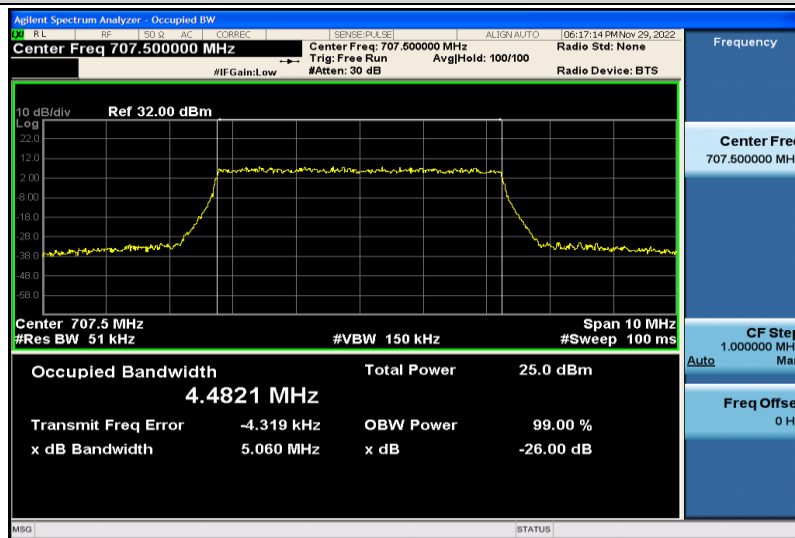
Band12-5MHz-64QAM-23095-25RB#0-4.4821
