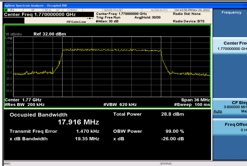
Band66-20MHz-16QAM-132572-100RB#0-17.916
