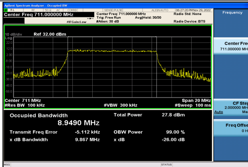
Band12-10MHz-64QAM-23130-50RB#0-8.9490
