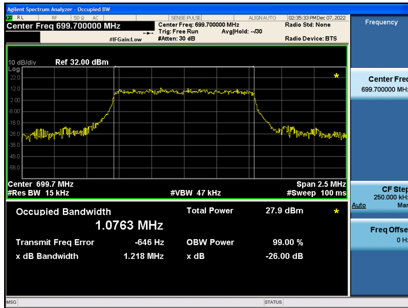
Band12-1.4MHz-64QAM-23017-6RB#0-1.0763
