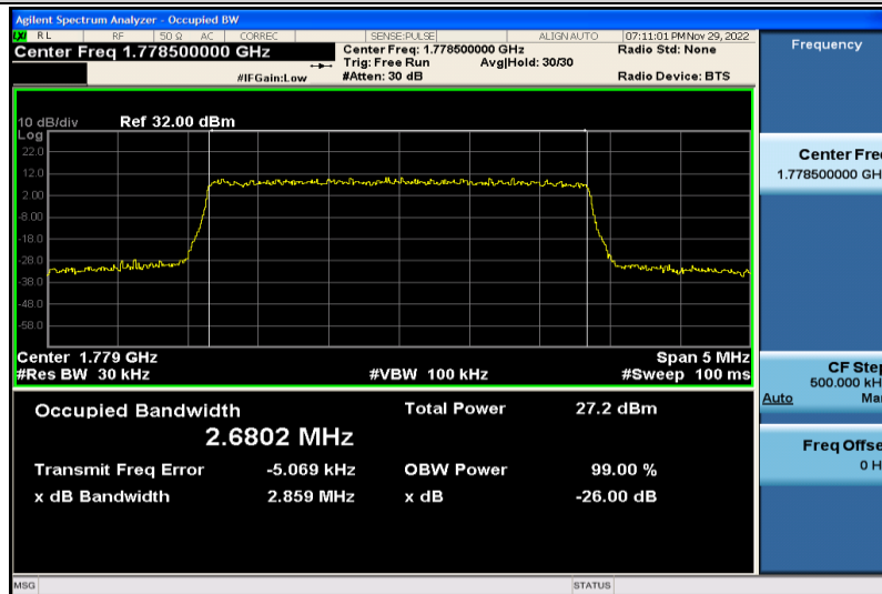
Band66-3MHz-64QAM-132657-15RB#0-2.6802
