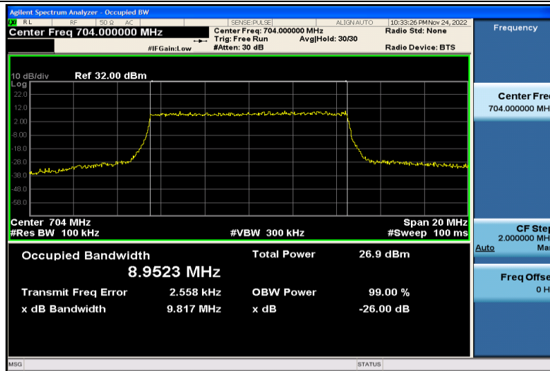
Band12-10MHz-16QAM-23060-50RB#0-8.9523
