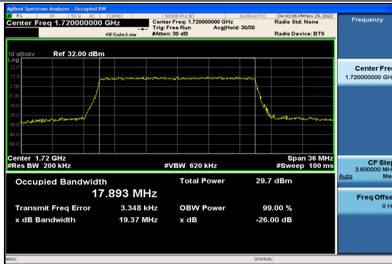
Band66-20MHz-QPSK-132072-100RB#0-17.893
