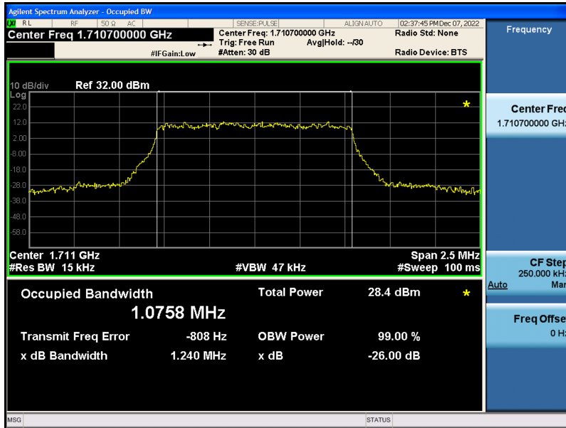
Band66-1.4MHz-64QAM-131979-6RB#0-1.0758
