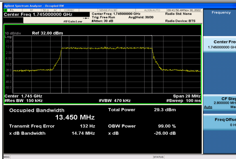
Band66-15MHz-64QAM-132322-75RB#0-13.450
