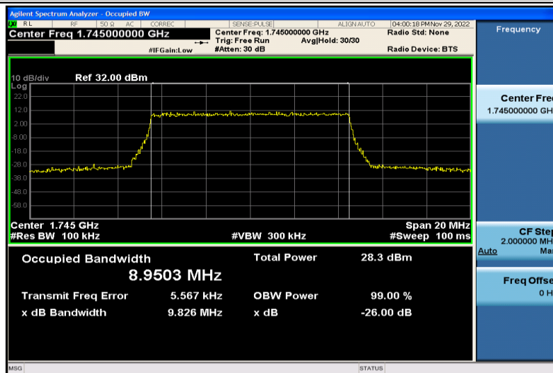
Band66-10MHz-16QAM-132322-50RB#0-8.9503
