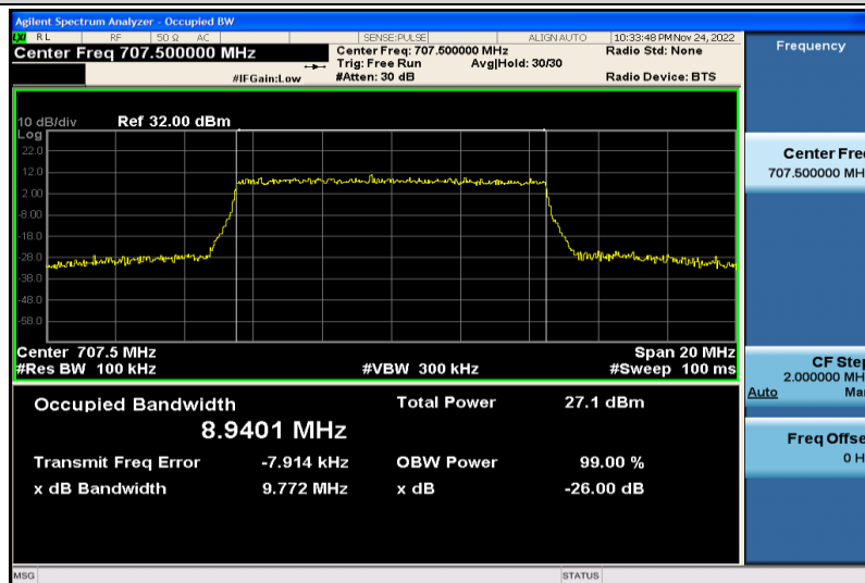
Band12-10MHz-16QAM-23095-50RB#0-8.9401
