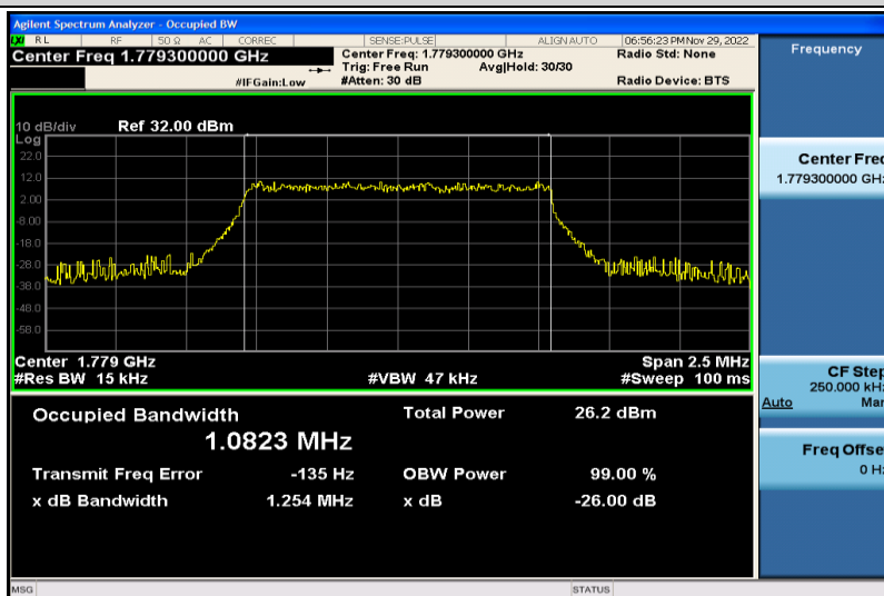
Band66-1.4MHz-64QAM-132665-6RB#0-1.0823
