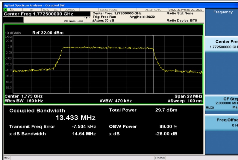
Band66-15MHz-QPSK-132597-75RB#0-13.433
