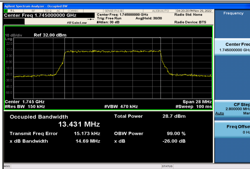
Band66-15MHz-16QAM-132322-75RB#0-13.431
