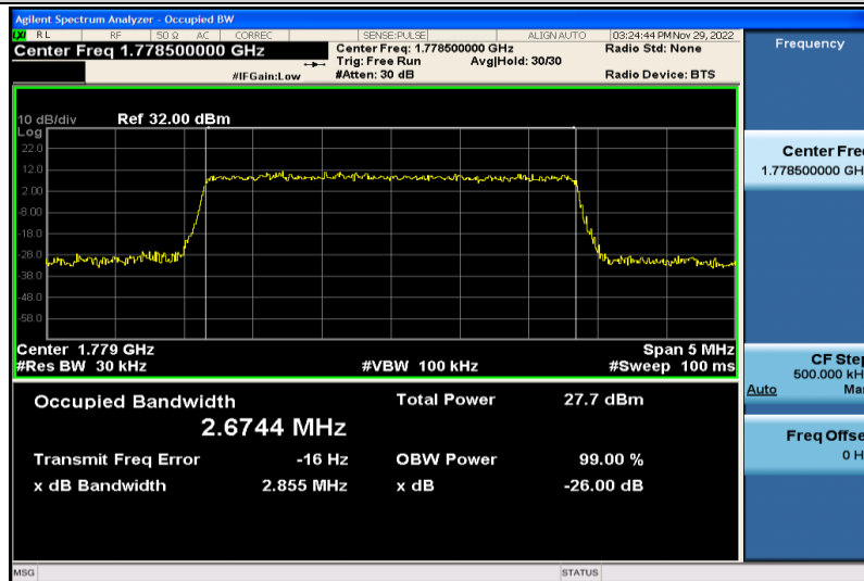
Band66-3MHz-16QAM-132657-15RB#0-2.6744
