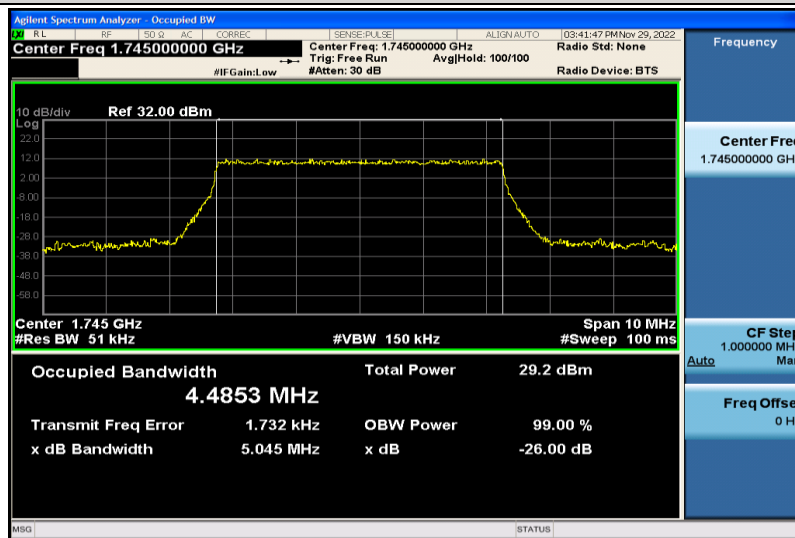
Band66-5MHz-QPSK-132322-25RB#0-4.4853
