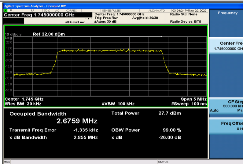
Band66-3MHz-16QAM-132322-15RB#0-2.6759
