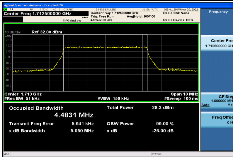
Band66-5MHz-16QAM-131997-25RB#0-4.4831
