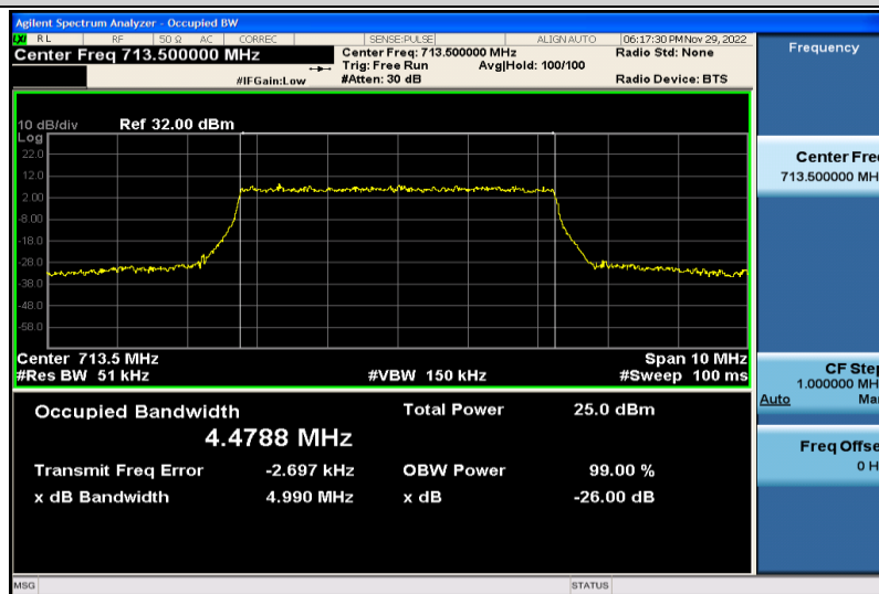
Band12-5MHz-64QAM-23155-25RB#0-4.4788
