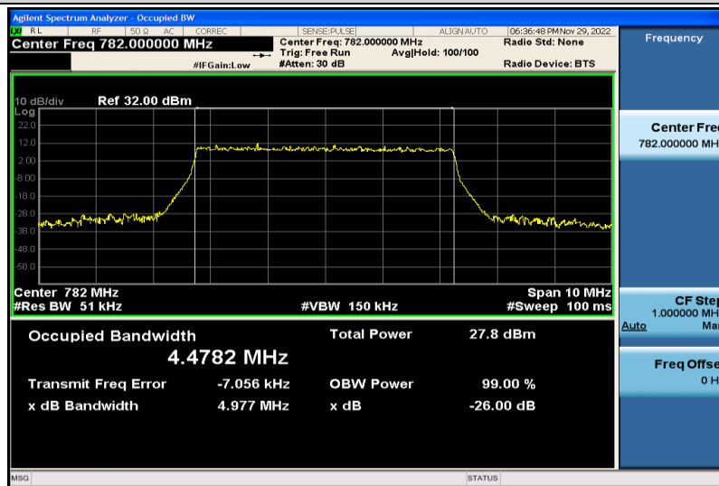
Band13-5MHz-64QAM-23230-25RB#0-4.4782
