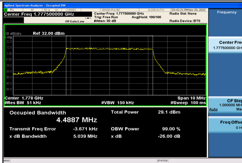
Band66-5MHz-QPSK-132647-25RB#0-4.4887
