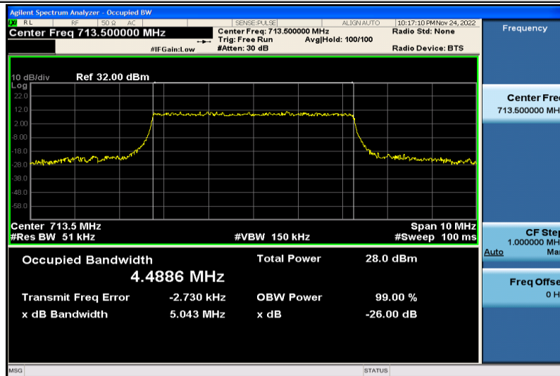
Band12-5MHz-QPSK-23155-25RB#0-4.4886
