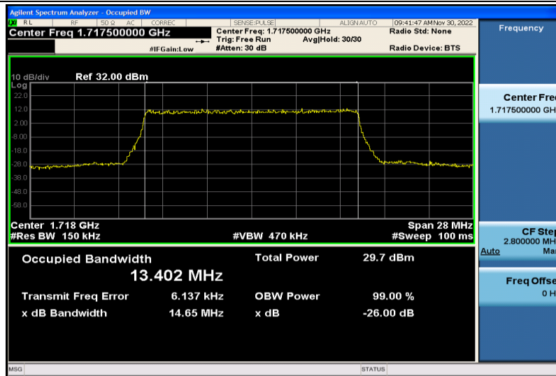
Band66-15MHz-64QAM-132047-75RB#0-13.402
