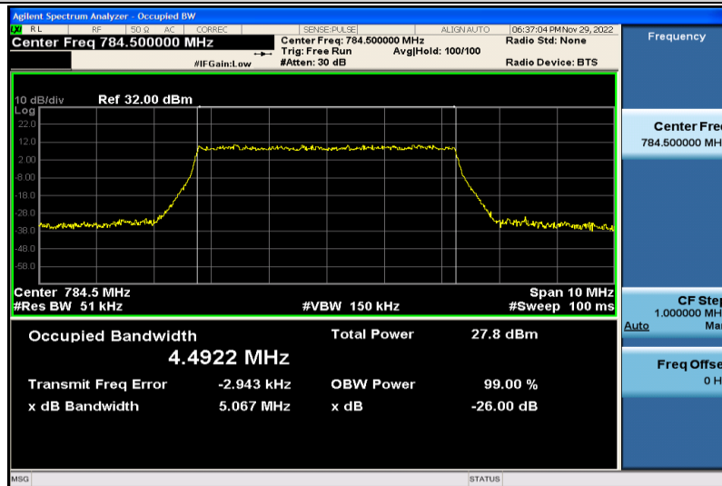
Band13-5MHz-64QAM-23255-25RB#0-4.4922
