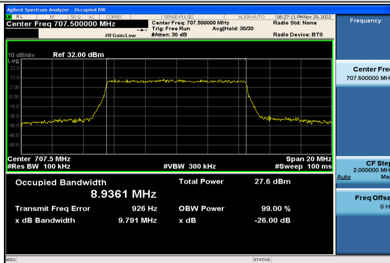
Band12-10MHz-64QAM-23095-50RB#0-8.9361
