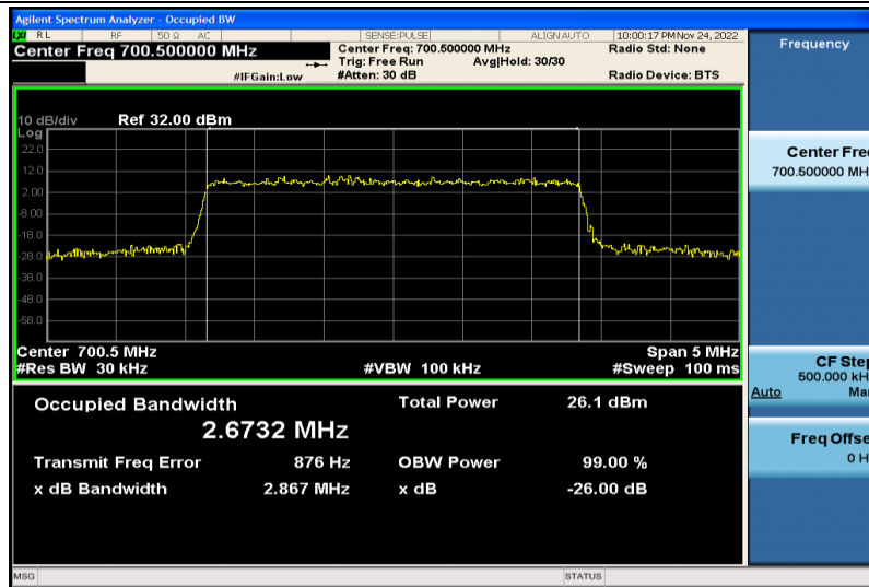
Band12-3MHz-16QAM-23025-15RB#0-2.6732
