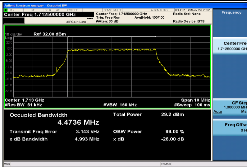
Band66-5MHz-QPSK-131997-25RB#0-4.4736
