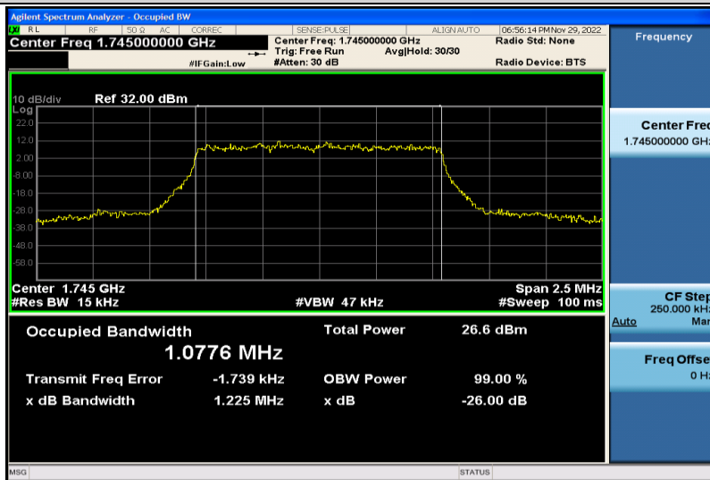
Band66-1.4MHz-64QAM-132322-6RB#0-1.0776
