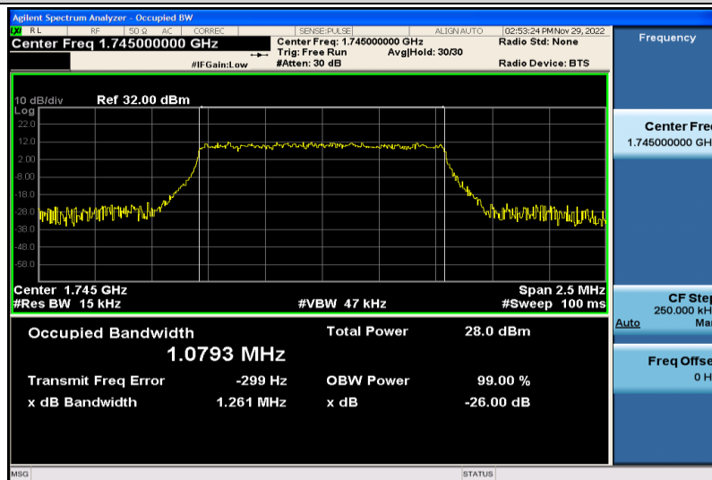
Band66-1.4MHz-QPSK-132322-6RB#0-1.0793
