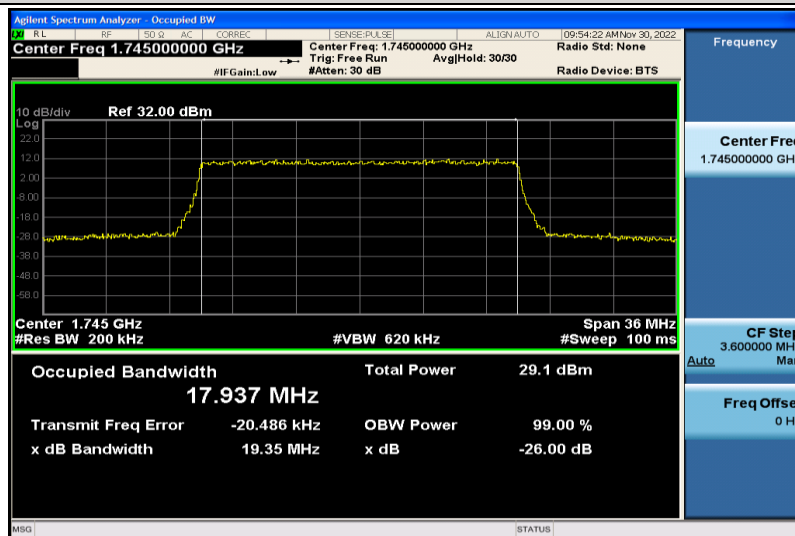
Band66-20MHz-64QAM-132322-100RB#0-17.937
