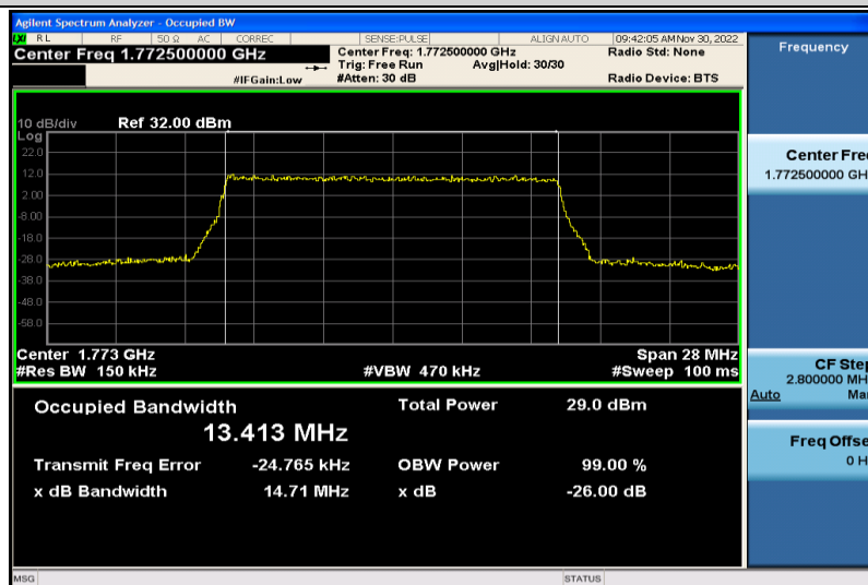
Band66-15MHz-64QAM-132597-75RB#0-13.413
