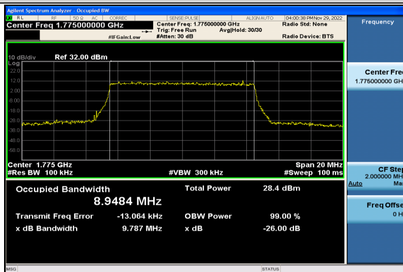
Band66-10MHz-16QAM-132622-50RB#0-8.9484
