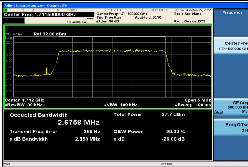
Band66-3MHz-16QAM-131987-15RB#0-2.6758
