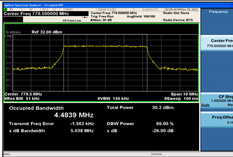
Band13-5MHz-QPSK-23205-25RB#0-4.4839
