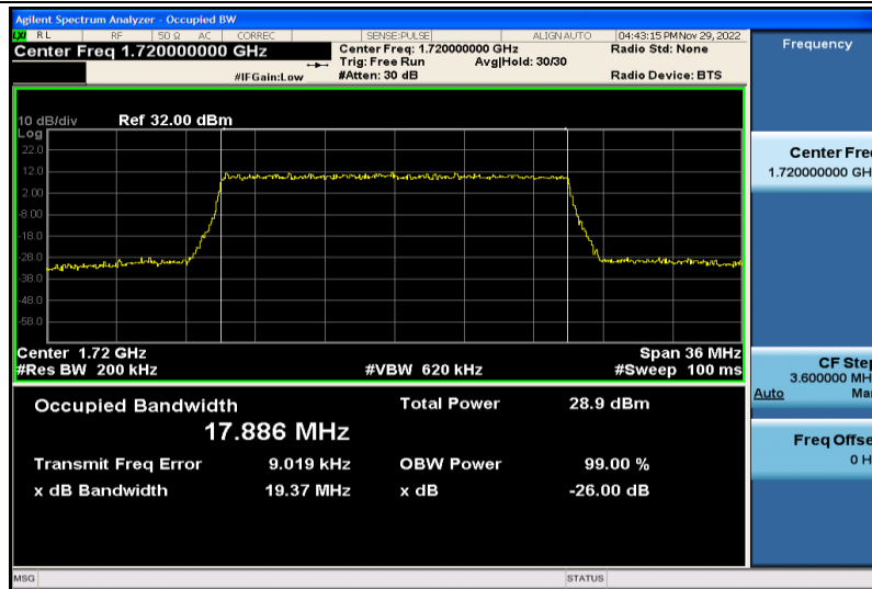
Band66-20MHz-16QAM-132072-100RB#0-17.886
