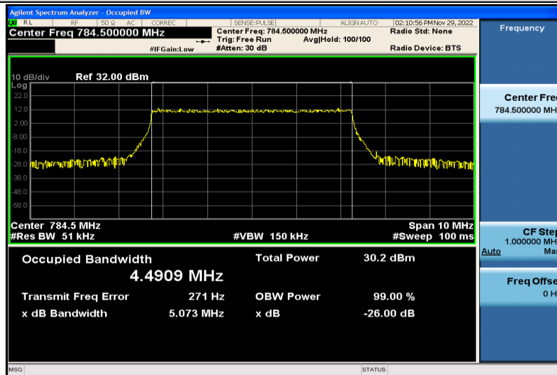
Band13-5MHz-QPSK-23255-25RB#0-4.4909
