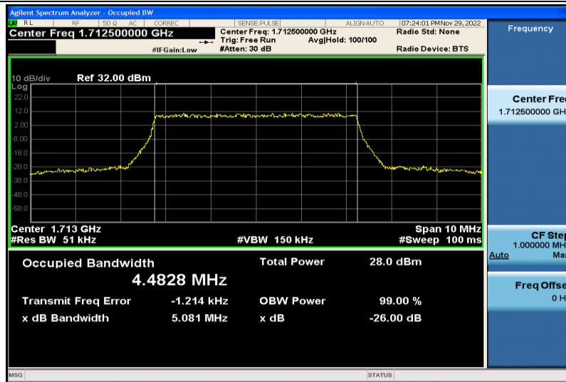
Band66-5MHz-64QAM-131997-25RB#0-4.4828
