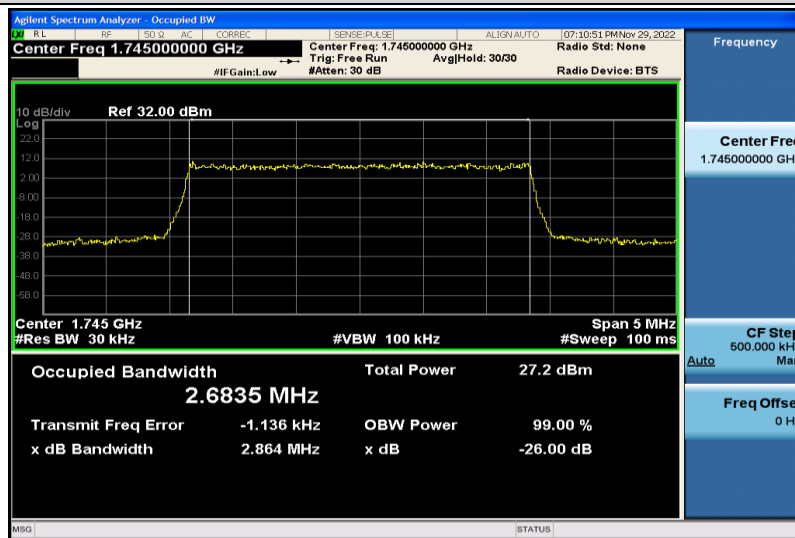
Band66-3MHz-64QAM-132322-15RB#0-2.6835
