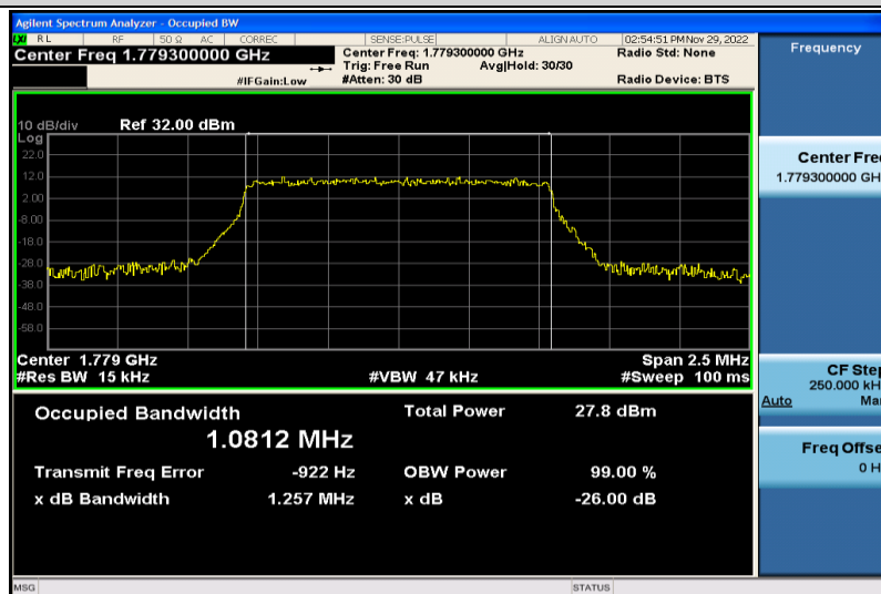
Band66-1.4MHz-QPSK-132665-6RB#0-1.0812
