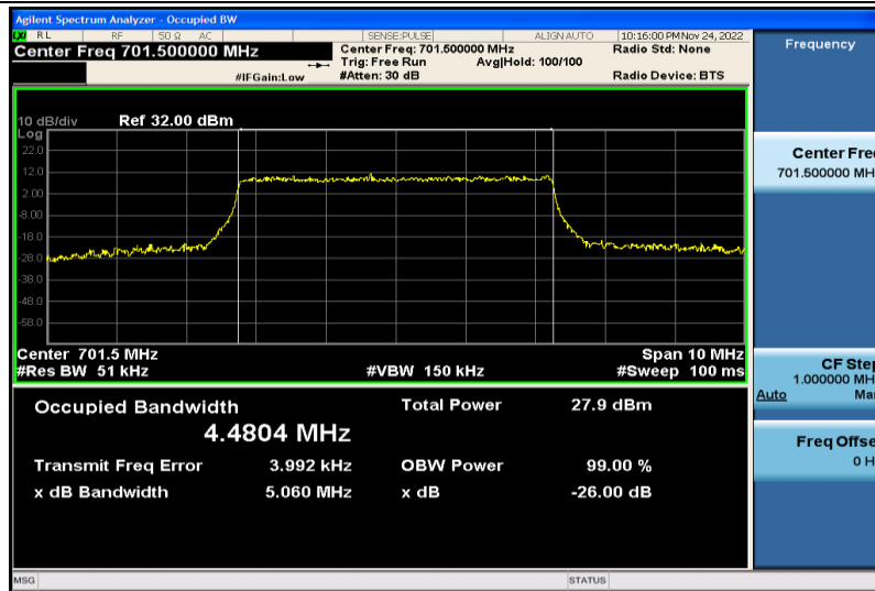
Band12-5MHz-QPSK-23035-25RB#0-4.4804
