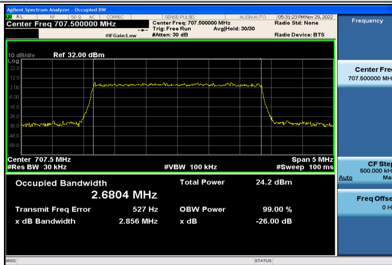
Band12-3MHz-64QAM-23095-15RB#0-2.6804
