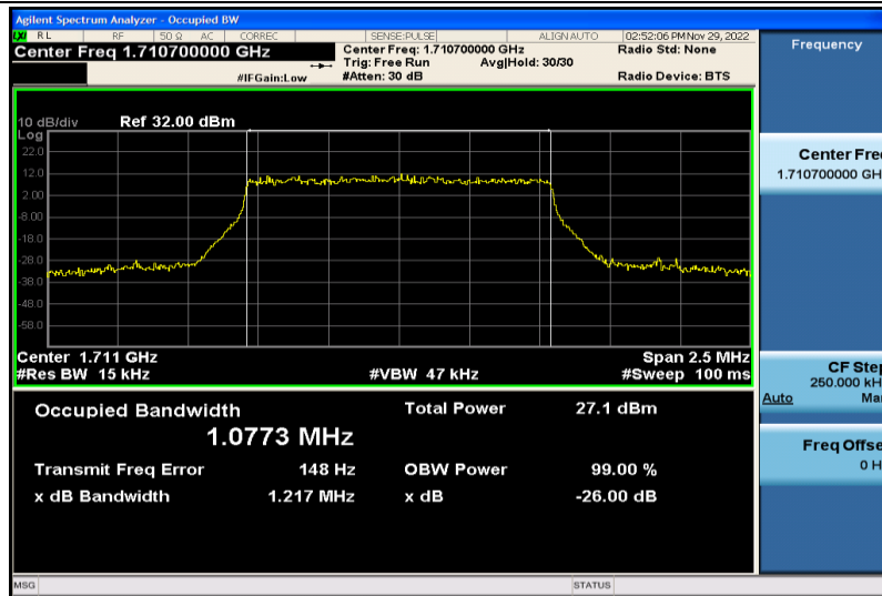
Band66-1.4MHz-16QAM-131979-6RB#0-1.0773
