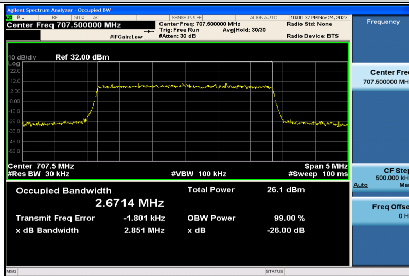
Band12-3MHz-16QAM-23095-15RB#0-2.6714
