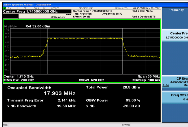
Band66-20MHz-16QAM-132322-100RB#0-17.903
