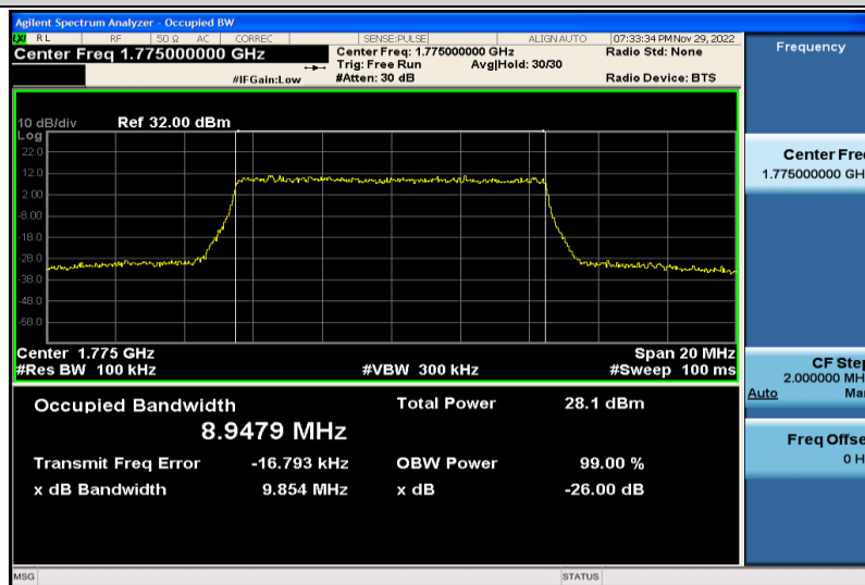
Band66-10MHz-64QAM-132622-50RB#0-8.9479
