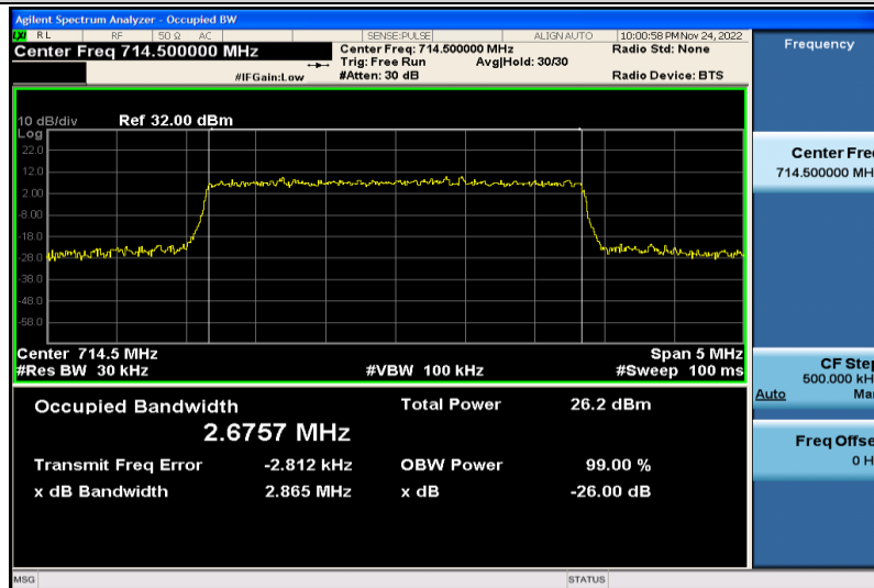
Band12-3MHz-16QAM-23165-15RB#0-2.6757
