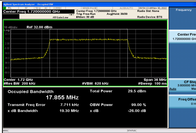
Band66-20MHz-64QAM-132072-100RB#0-17.855
