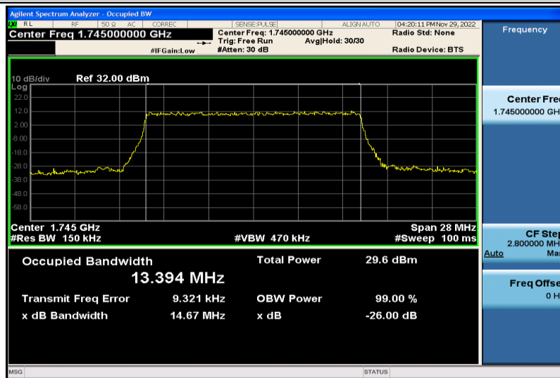
Band66-15MHz-QPSK-132322-75RB#0-13.394
