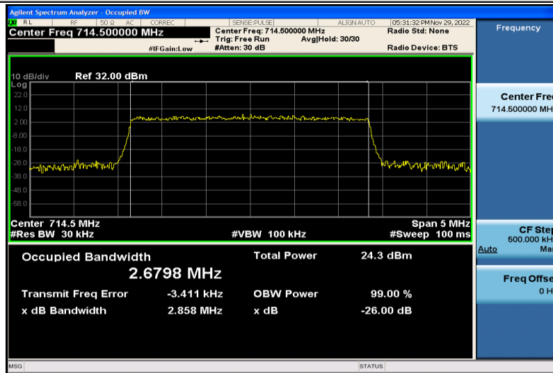
Band12-3MHz-64QAM-23165-15RB#0-2.6798
