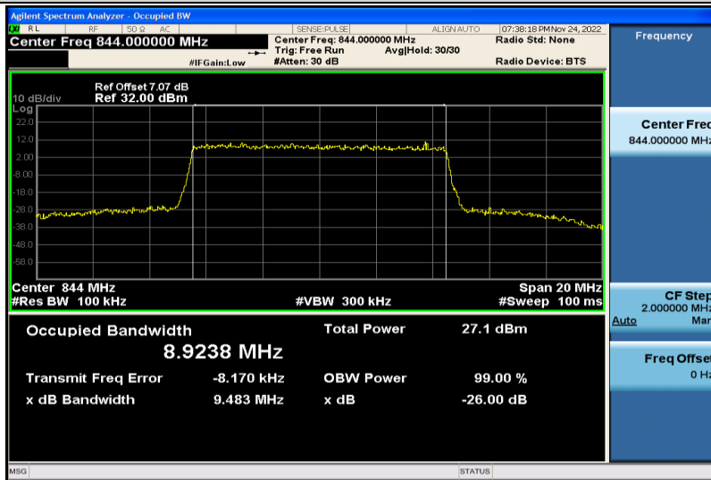
Band5-10MHz-16QAM-20600-50RB#0-8.9238
