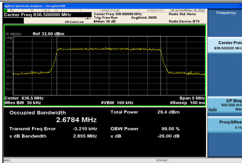
Band5-3MHz-64QAM-20525-15RB#0-2.6784
