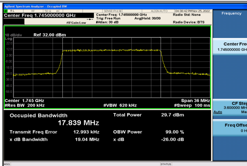
Band4-20MHz-64QAM-20300-100RB#0-17.839
