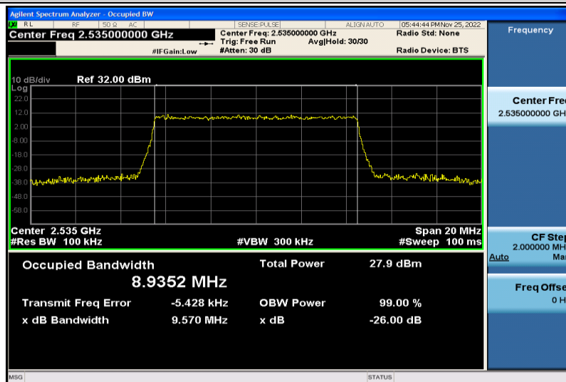
Band7-10MHz-64QAM-21100-50RB#0-8.9352
