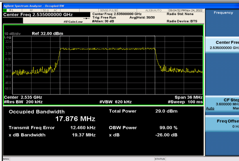
Band7-20MHz-QPSK-21100-100RB#0-17.876
