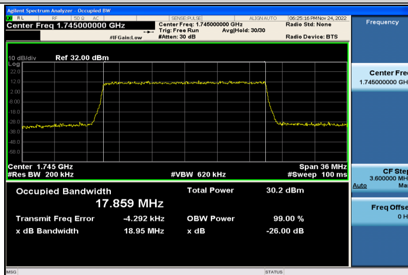
Band4-20MHz-QPSK-20300-100RB#0-17.859
