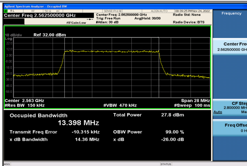
Band7-15MHz-16QAM-21375-75RB#0-13.398
