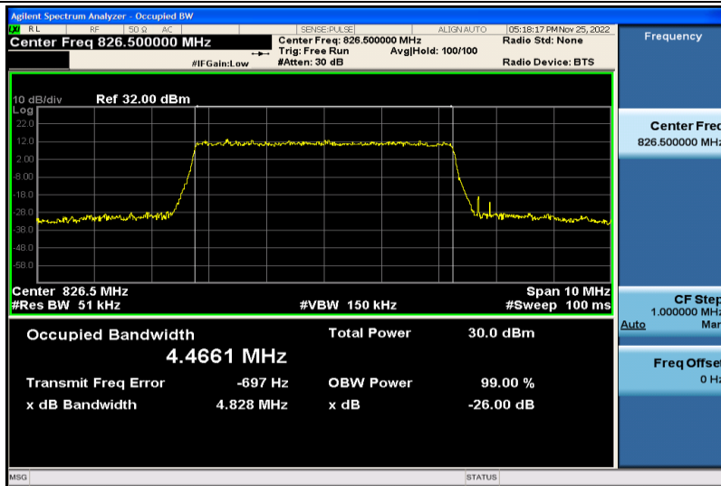
Band5-5MHz-64QAM-20425-25RB#0-4.4661
