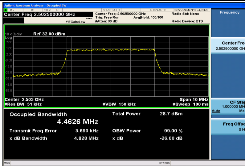
Band7-5MHz-QPSK-20775-25RB#0-4.4626
