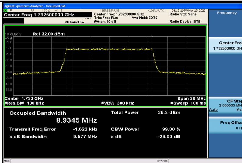
Band4-10MHz-64QAM-20175-50RB#0-8.9345
