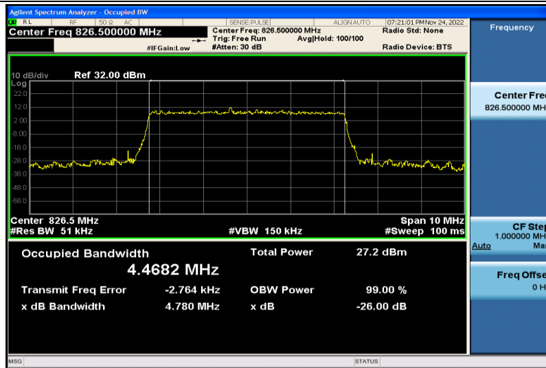
Band5-5MHz-16QAM-20425-25RB#0-4.4682
