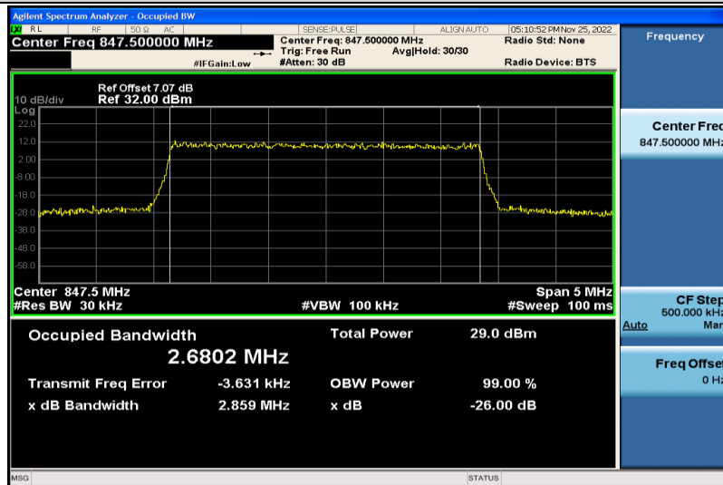
Band5-3MHz-64QAM-20635-15RB#0-2.6802
