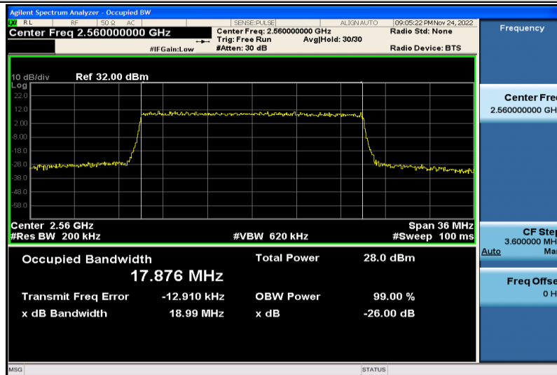
Band7-20MHz-16QAM-21350-100RB#0-17.876
