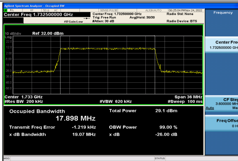
Band4-20MHz-16QAM-20175-100RB#0-17.898
