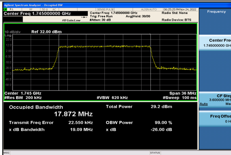
Band4-20MHz-16QAM-20300-100RB#0-17.872
