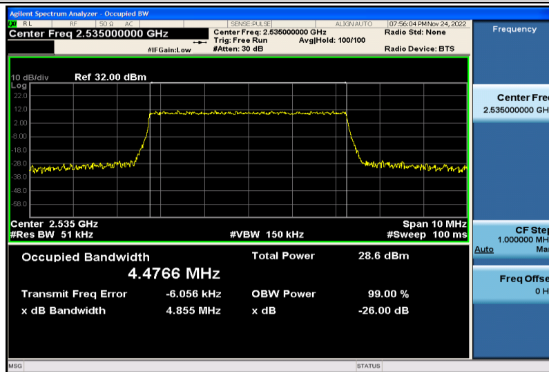
Band7-5MHz-QPSK-21100-25RB#0-4.4766
