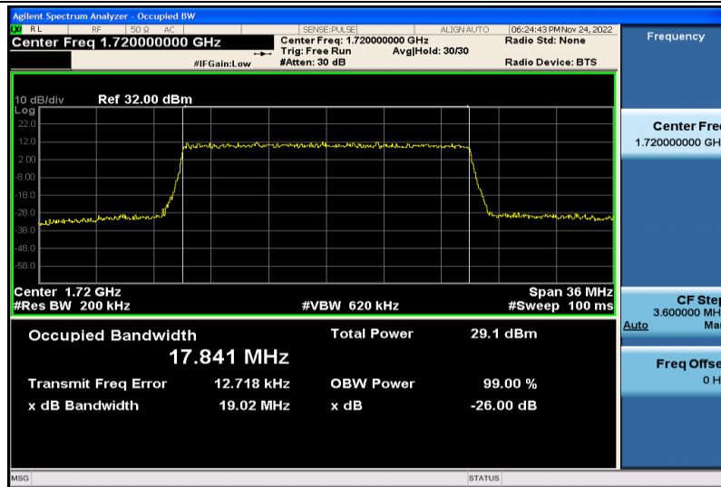
Band4-20MHz-16QAM-20050-100RB#0-17.841
