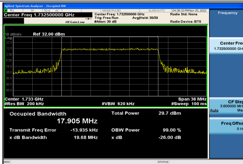
Band4-20MHz-64QAM-20175-100RB#0-17.905
