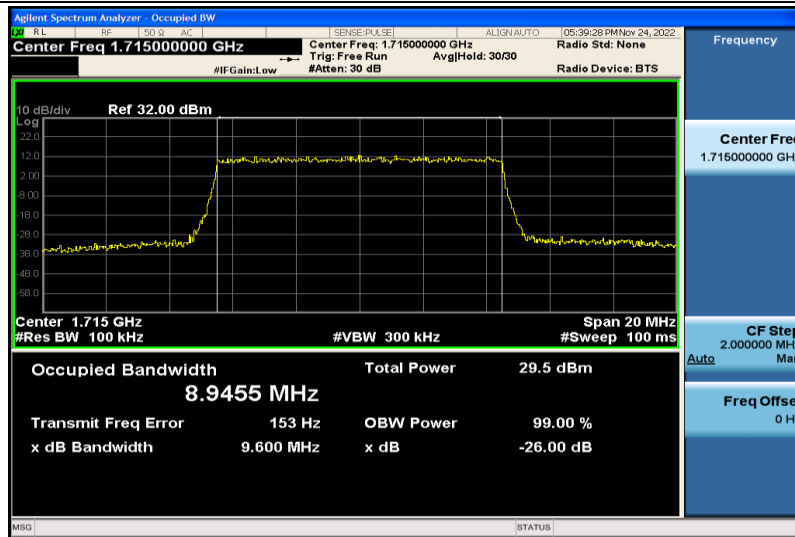
Band4-10MHz-QPSK-20000-50RB#0-8.9455
