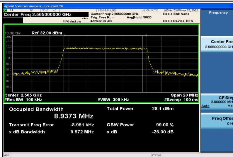
Band7-10MHz-64QAM-21400-50RB#0-8.9373
