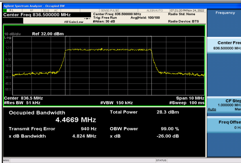
Band5-5MHz-QPSK-20525-25RB#0-4.4669
