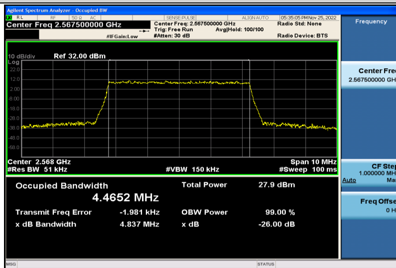
Band7-5MHz-64QAM-21425-25RB#0-4.4652
