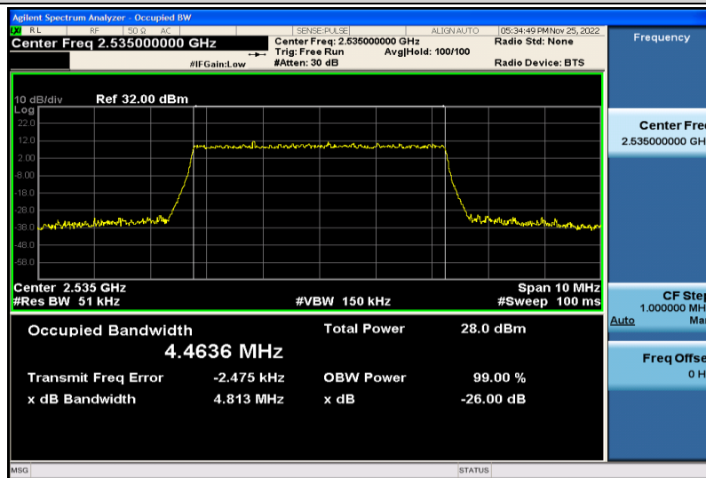
Band7-5MHz-64QAM-21100-25RB#0-4.4636
