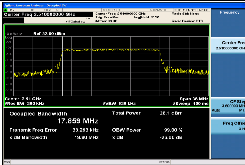
Band7-20MHz-16QAM-20850-100RB#0-17.859
