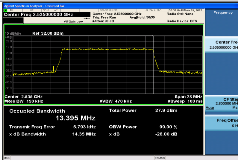
Band7-15MHz-16QAM-21100-75RB#0-13.395
