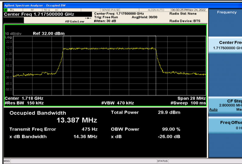
Band4-15MHz-QPSK-20025-75RB#0-13.387
