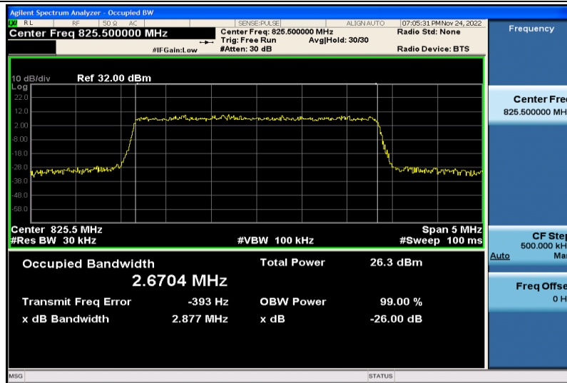
Band5-3MHz-16QAM-20415-15RB#0-2.6704
