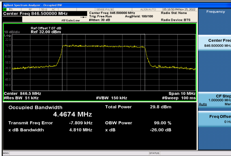
Band5-5MHz-64QAM-20625-25RB#0-4.4674
