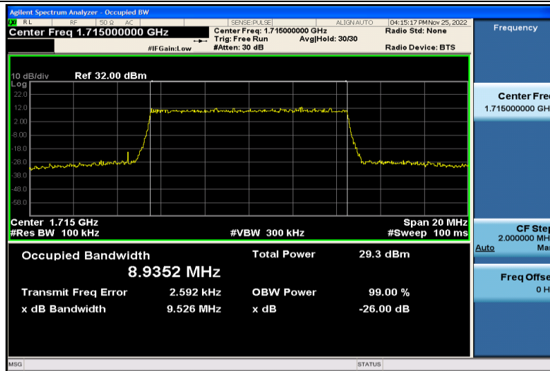
Band4-10MHz-64QAM-20000-50RB#0-8.9352
