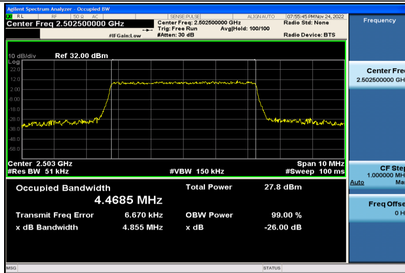
Band7-5MHz-16QAM-20775-25RB#0-4.4685
