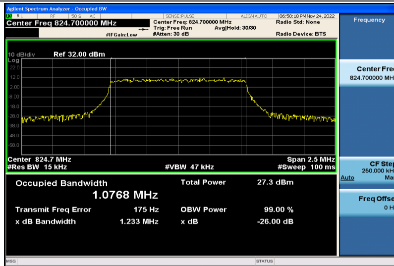
Band5-1.4MHz-QPSK-20407-6RB#0-1.0768
