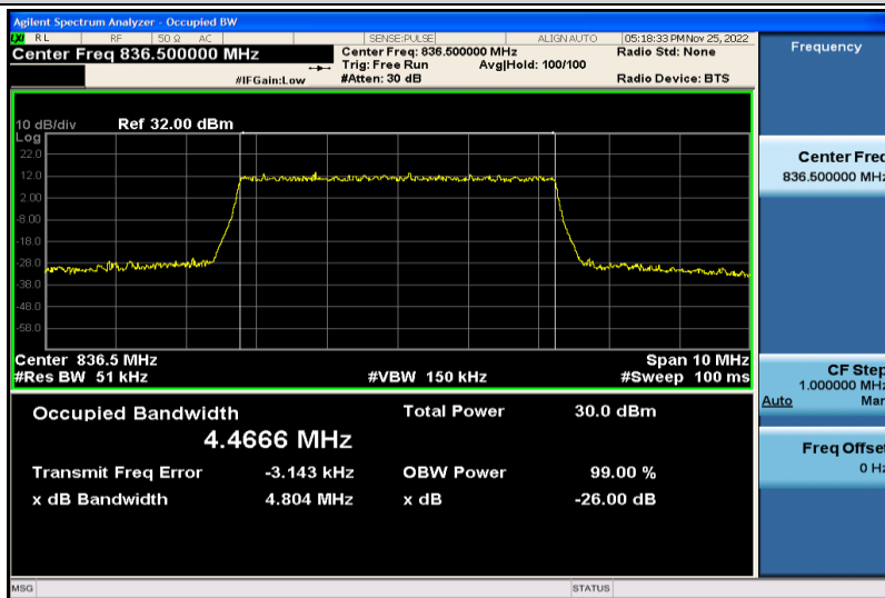
Band5-5MHz-64QAM-20525-25RB#0-4.4666
