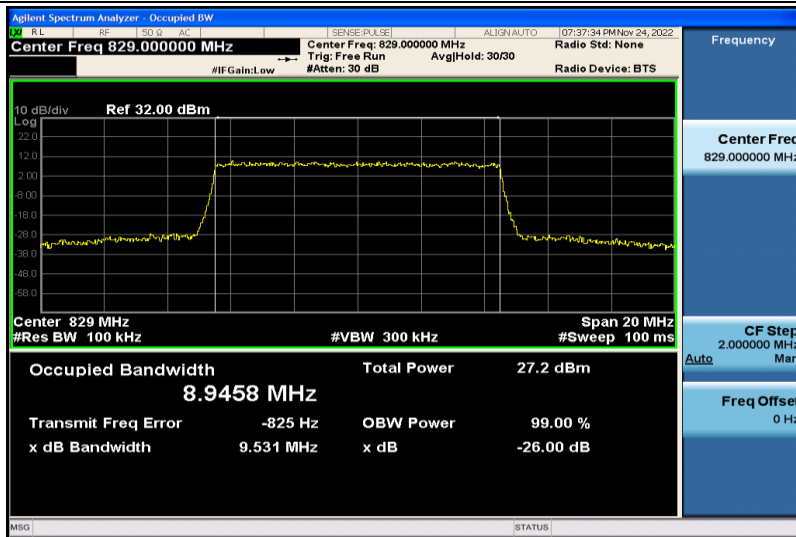
Band5-10MHz-16QAM-20450-50RB#0-8.9458
