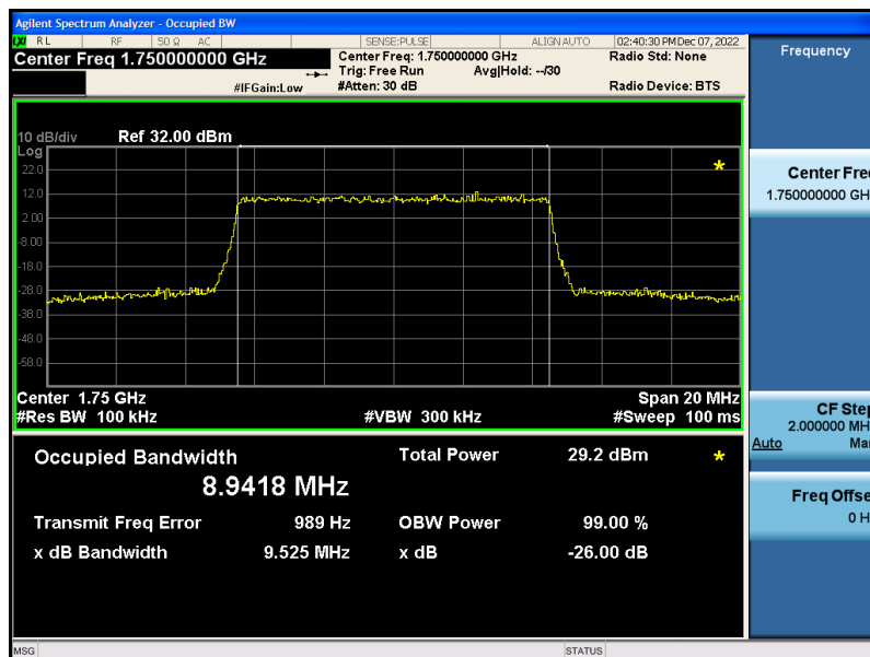
Band4-10MHz-64QAM-20350-50RB#0-8.9418
