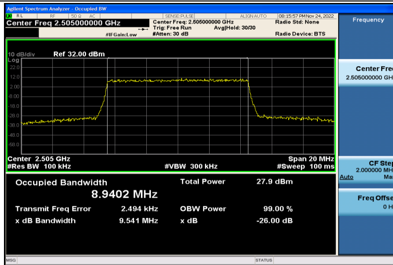
Band7-10MHz-16QAM-20800-50RB#0-8.9402
