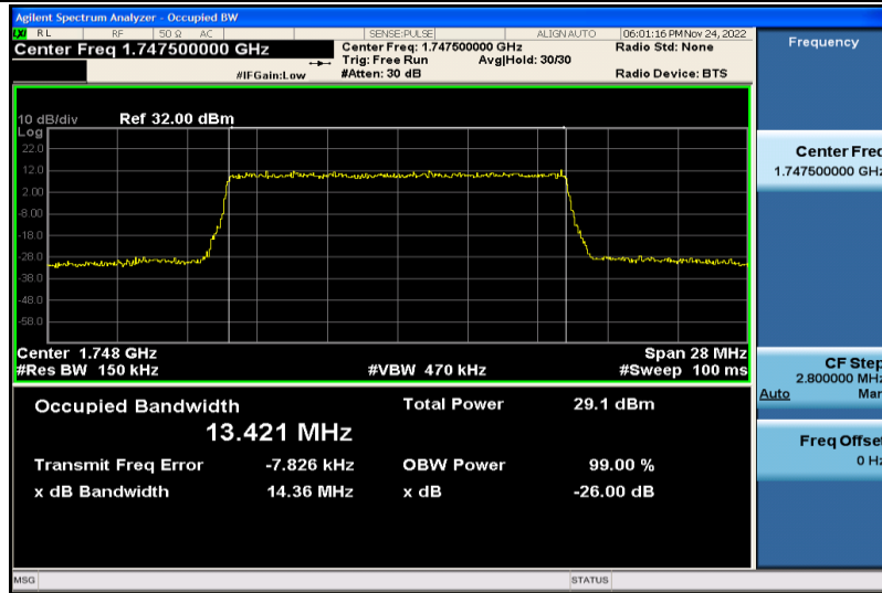
Band4-15MHz-16QAM-20325-75RB#0-13.421
