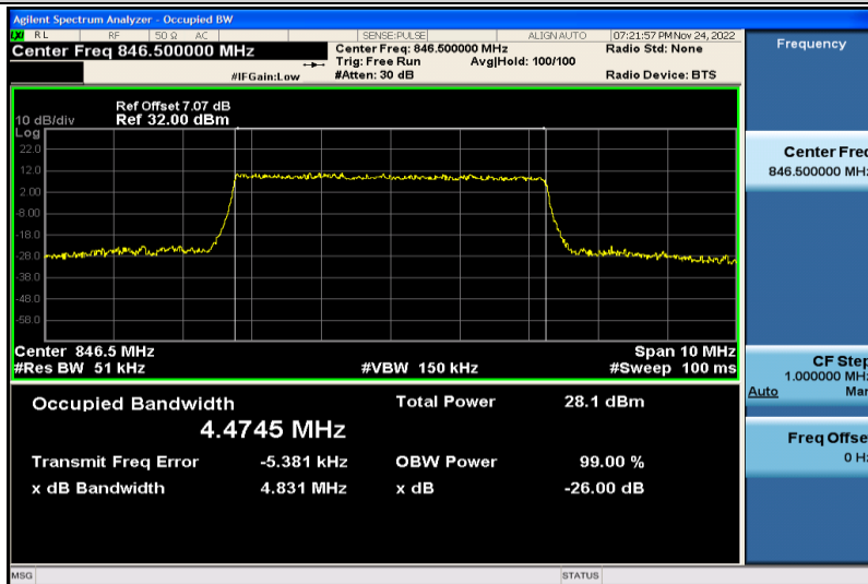
Band5-5MHz-QPSK-20625-25RB#0-4.4745
