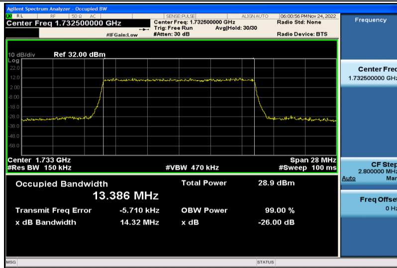
Band4-15MHz-16QAM-20175-75RB#0-13.386
