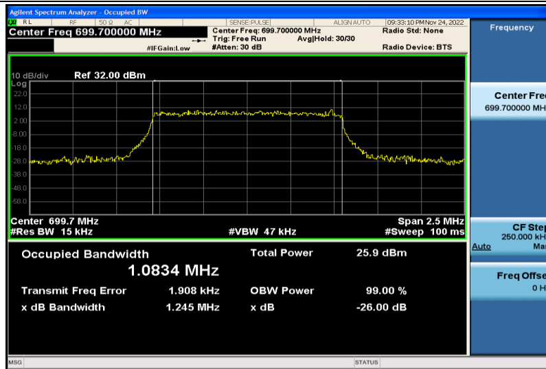
Band12-1.4MHz-QPSK-23017-6RB#0-1.0834
