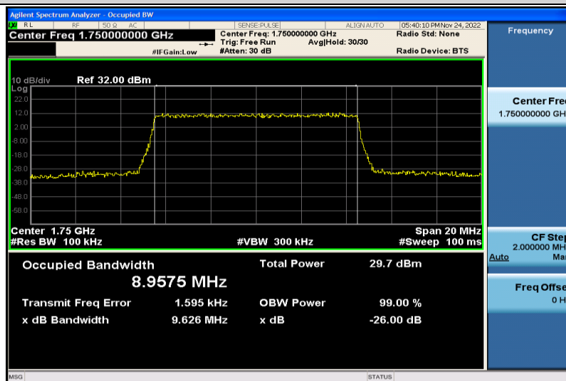
Band4-10MHz-QPSK-20350-50RB#0-8.9575
