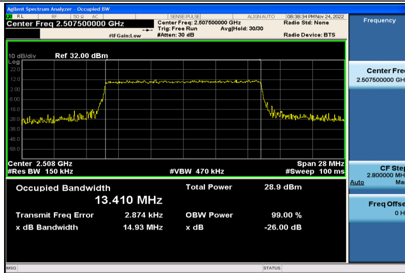
Band7-15MHz-QPSK-20825-75RB#0-13.410
