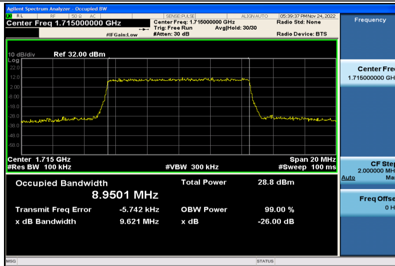
Band4-10MHz-16QAM-20000-50RB#0-8.9501
