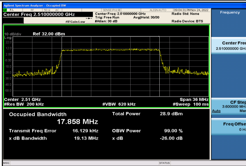
Band7-20MHz-QPSK-20850-100RB#0-17.858
