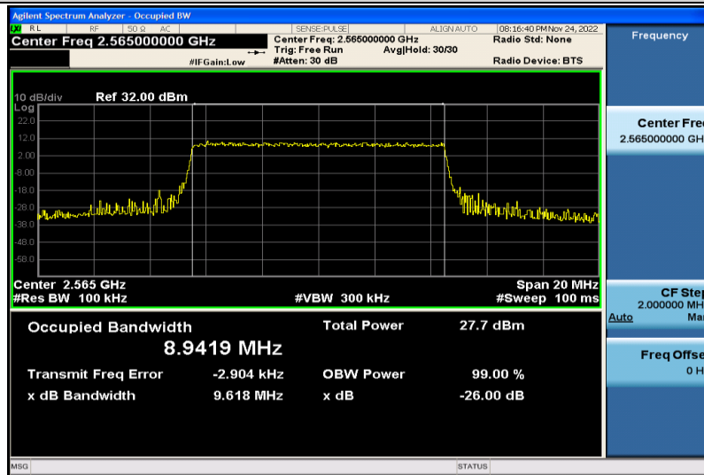
Band7-10MHz-16QAM-21400-50RB#0-8.9419
