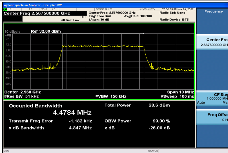
Band7-5MHz-QPSK-21425-25RB#0-4.4784
