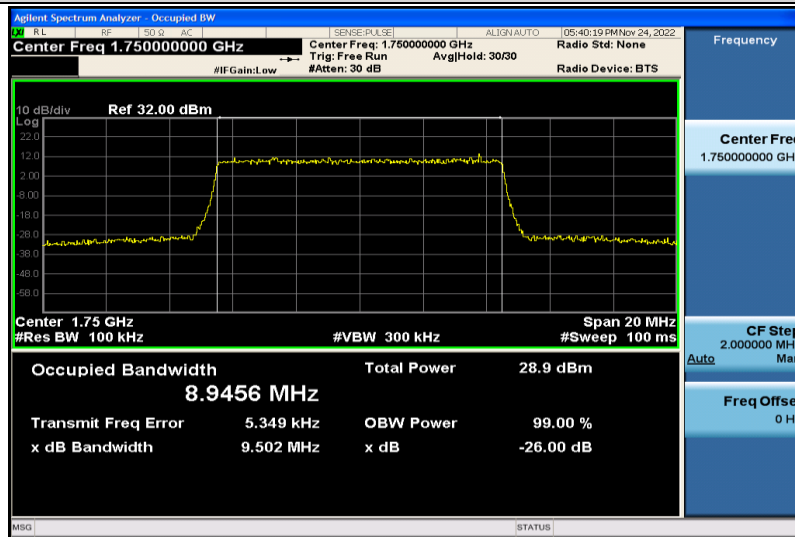
Band4-10MHz-16QAM-20350-50RB#0-8.9456
