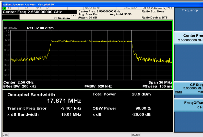
Band7-20MHz-QPSK-21350-100RB#0-17.871
