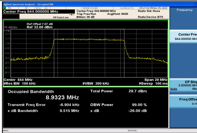
Band5-10MHz-64QAM-20600-50RB#0-8.9323
