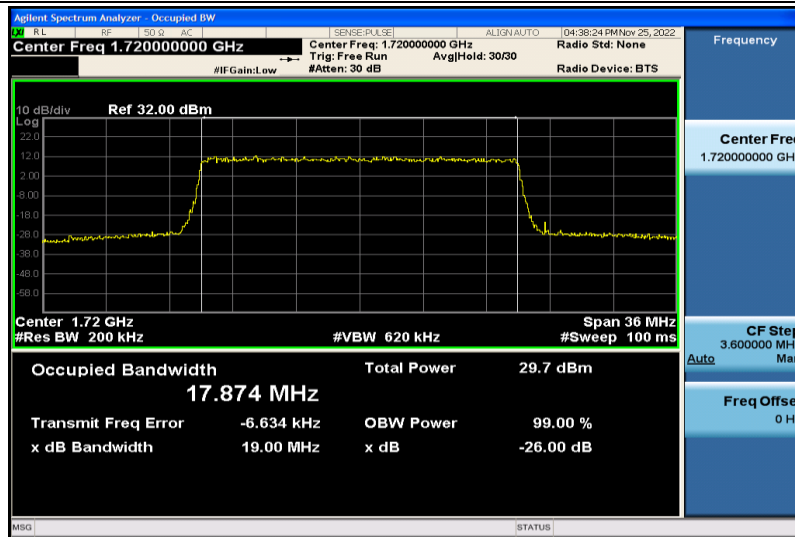
Band4-20MHz-64QAM-20050-100RB#0-17.874
