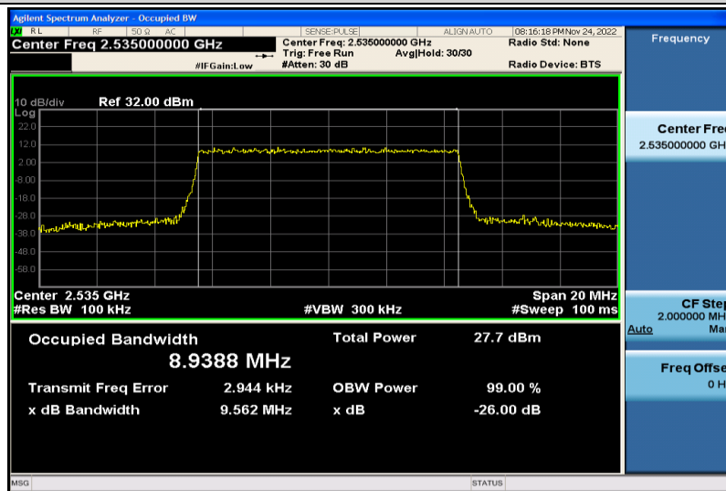
Band7-10MHz-16QAM-21100-50RB#0-8.9388
