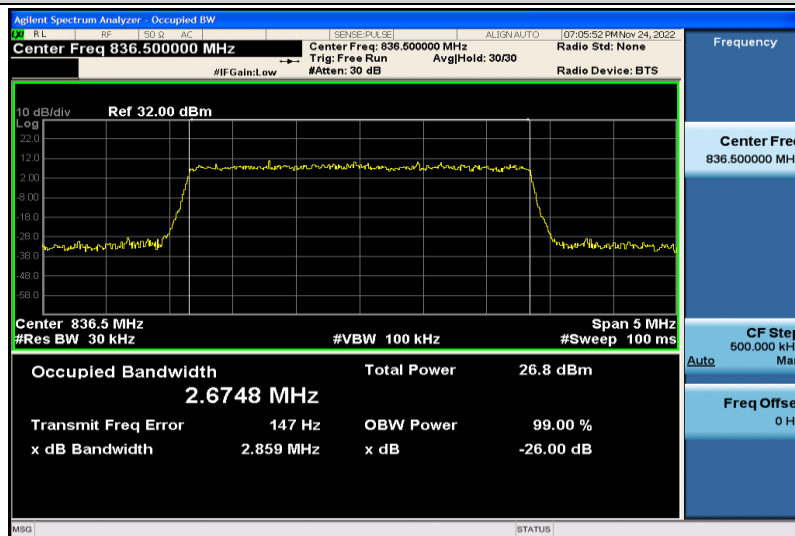
Band5-3MHz-16QAM-20525-15RB#0-2.6748
