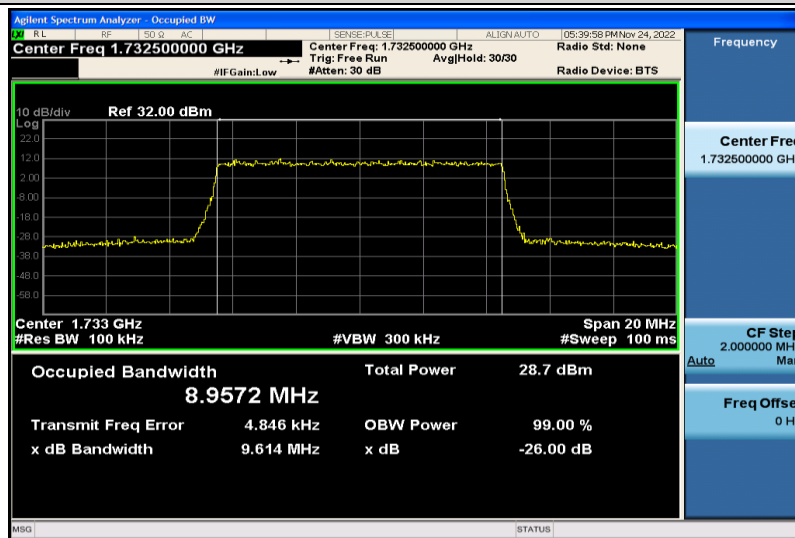
Band4-10MHz-16QAM-20175-50RB#0-8.9572
