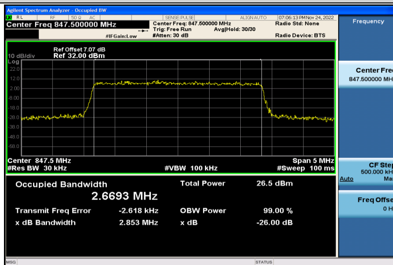
Band5-3MHz-16QAM-20635-15RB#0-2.6693
