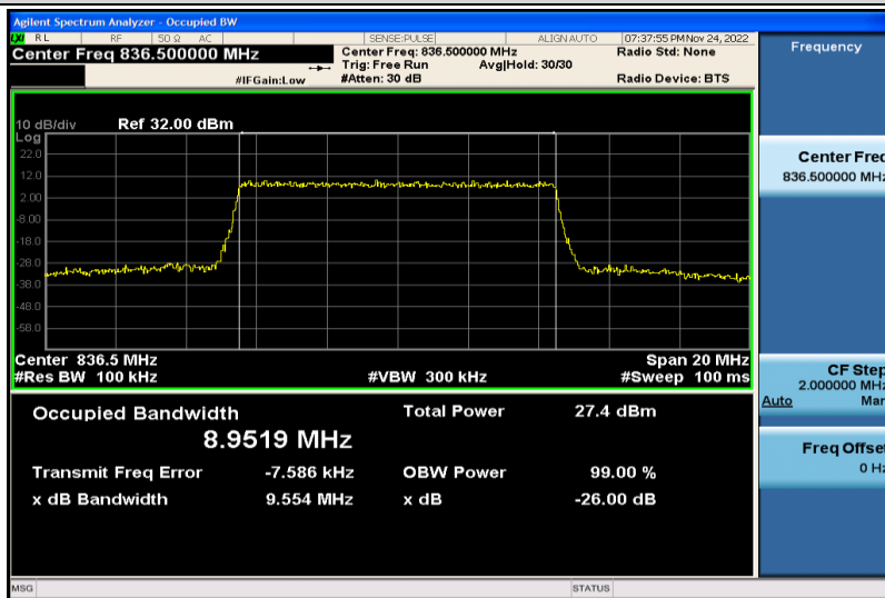
Band5-10MHz-16QAM-20525-50RB#0-8.9519
