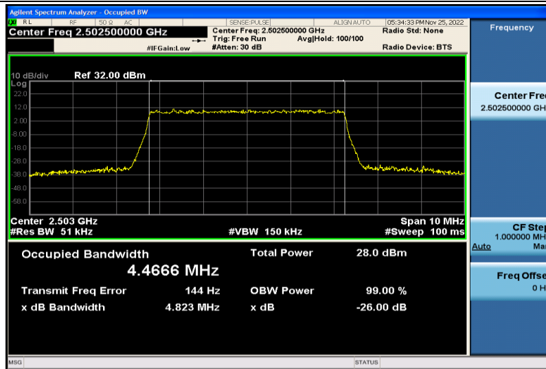
Band7-5MHz-64QAM-20775-25RB#0-4.4666
