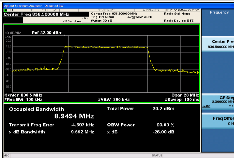
Band5-10MHz-64QAM-20525-50RB#0-8.9494
