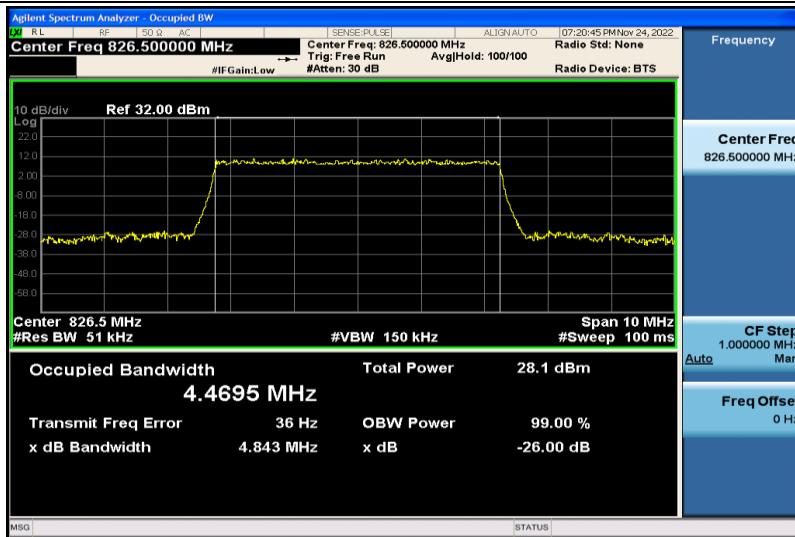
Band5-5MHz-QPSK-20425-25RB#0-4.4695
