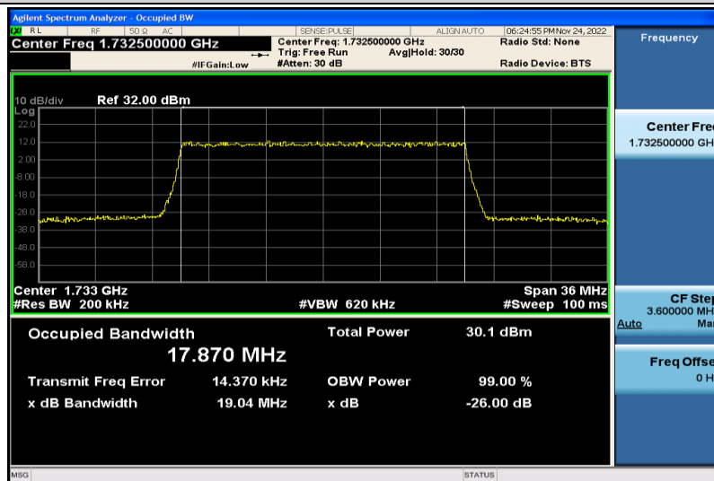
Band4-20MHz-QPSK-20175-100RB#0-17.870
