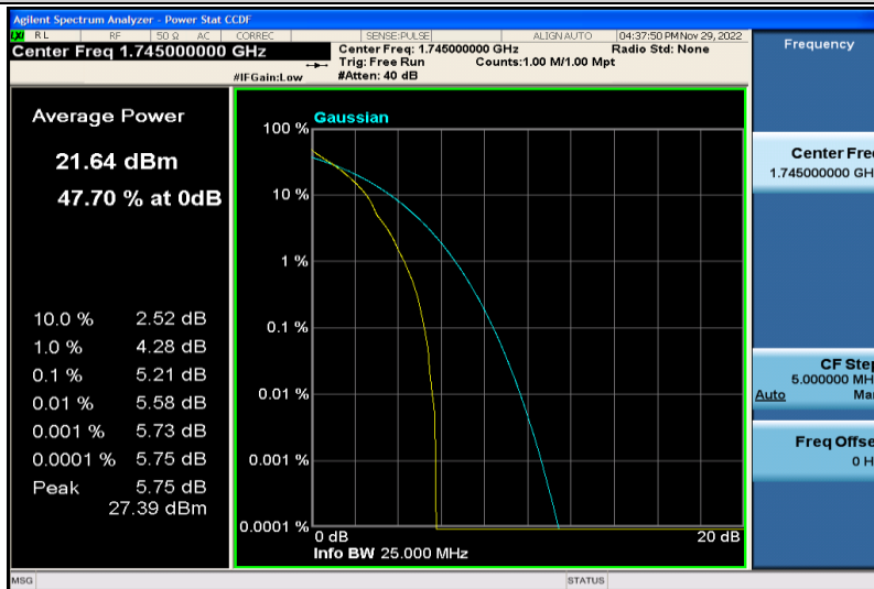
Band66-15MHz-QPSK-132322-1RB#0
