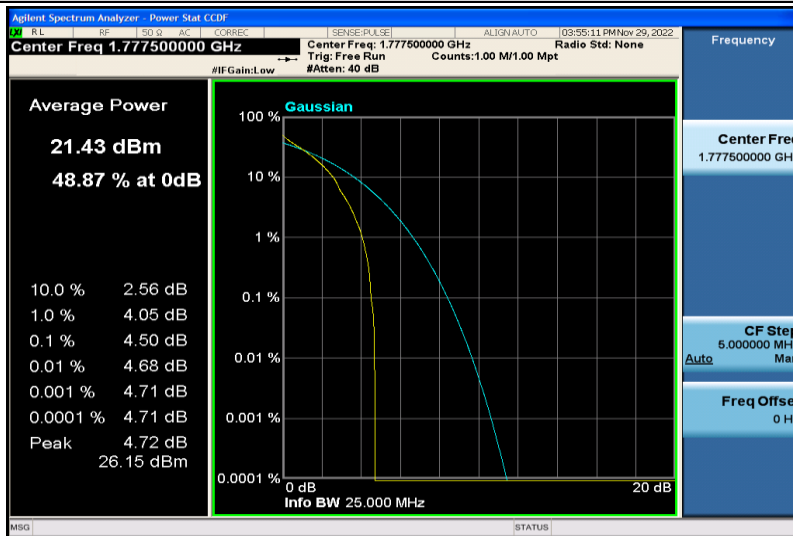
Band66-5MHz-QPSK-132647-1RB#0
