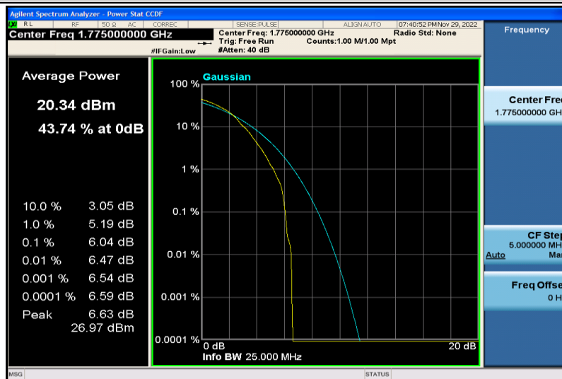
Band66-10MHz-64QAM-132622-1RB#0
