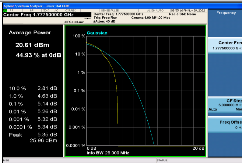
Band66-5MHz-16QAM-132647-1RB#0
