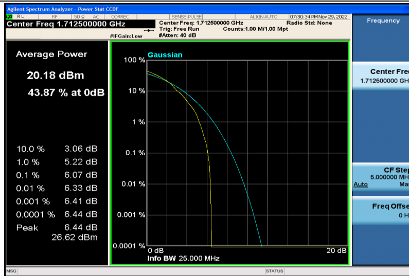
Band66-5MHz-64QAM-131997-1RB#0
