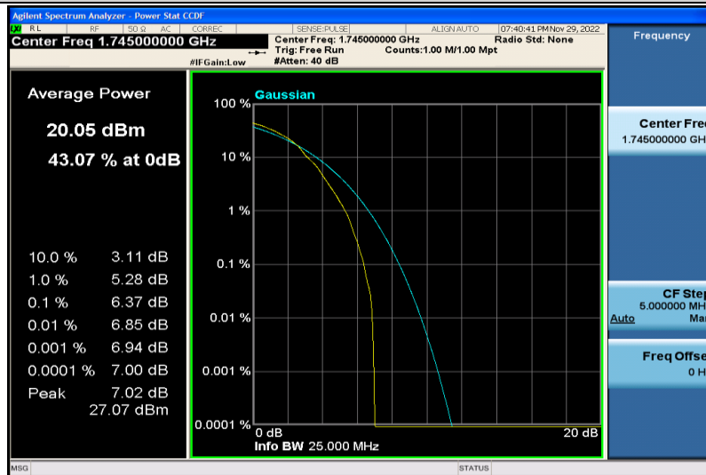
Band66-10MHz-64QAM-132322-1RB#0
