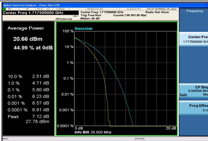
Band66-15MHz-QPSK-132047-75RB#0
