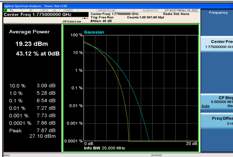
Band66-10MHz-64QAM-132622-50RB#0
