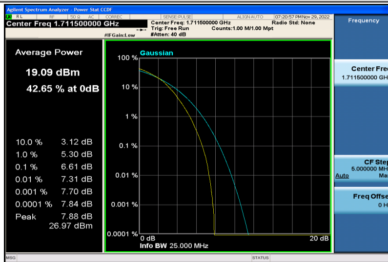
Band66-3MHz-64QAM-131987-15RB#0
