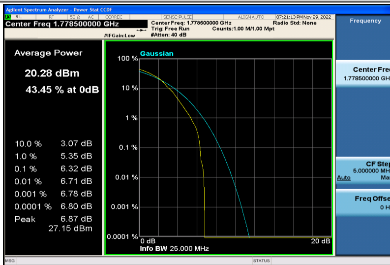
Band66-3MHz-64QAM-132657-1RB#0
