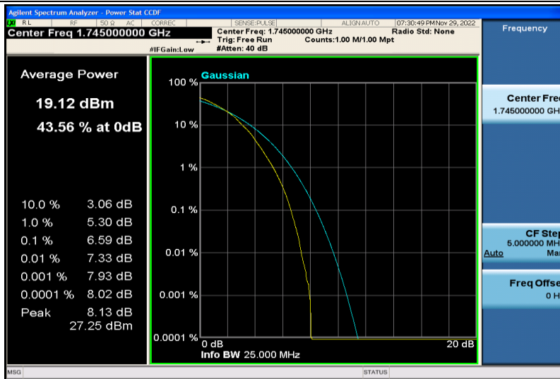
Band66-5MHz-64QAM-132322-25RB#0
