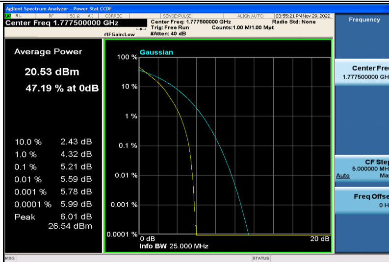
Band66-5MHz-QPSK-132647-25RB#0
