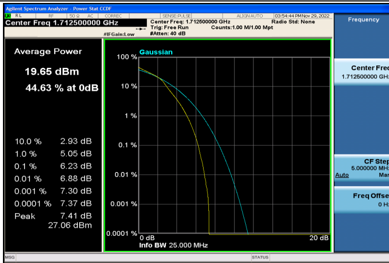
Band66-5MHz-16QAM-131997-25RB#0
