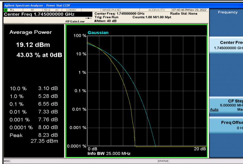
Band66-10MHz-64QAM-132322-50RB#0
