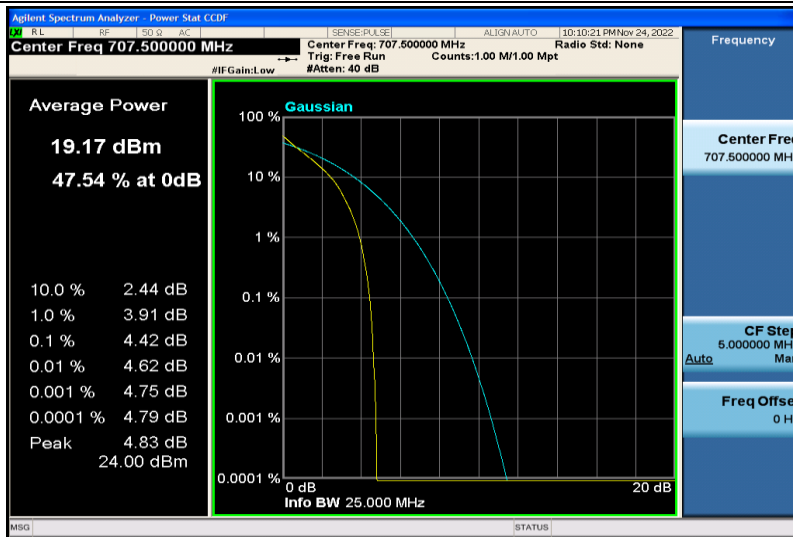
Band12-3MHz-QPSK-23095-15RB#0
