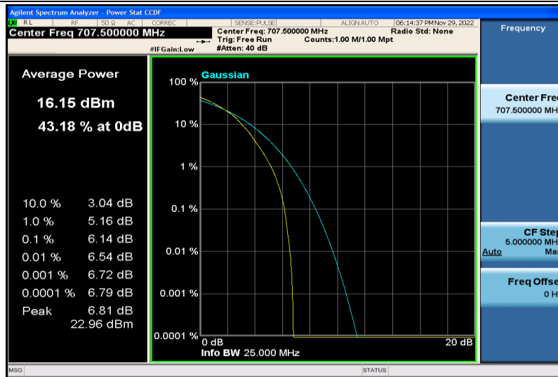
Band12-3MHz-64QAM-23095-15RB#0
