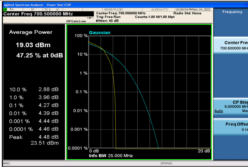
Band12-3MHz-16QAM-23025-1RB#0
