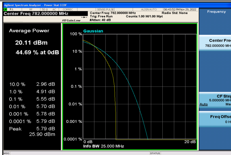
Band13-5MHz-64QAM-23230-1RB#0
