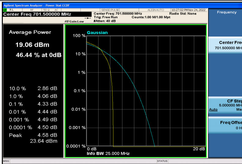
Band12-5MHz-16QAM-23035-1RB#0
