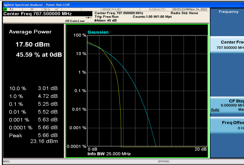
Band12-1.4MHz-16QAM-23095-6RB#0
