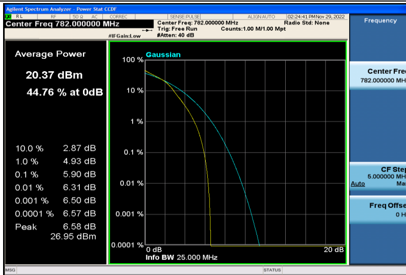
Band13-5MHz-16QAM-23230-25RB#0
