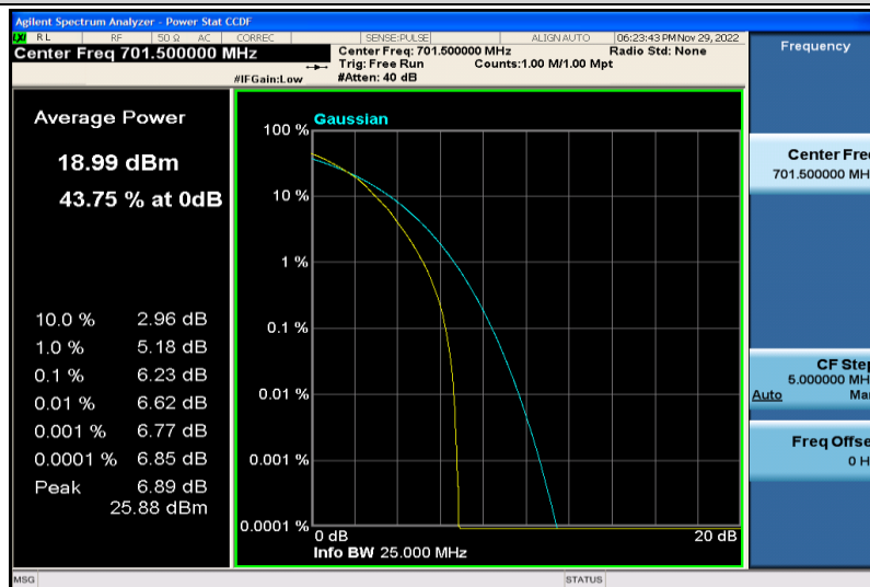
Band12-5MHz-64QAM-23035-25RB#0
