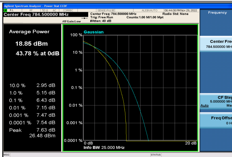
Band13-5MHz-64QAM-23255-25RB#0
