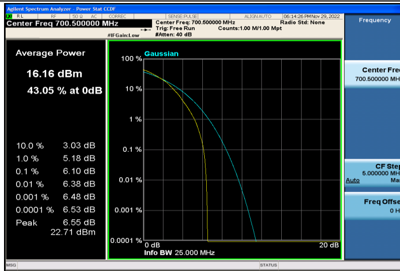
Band12-3MHz-64QAM-23025-15RB#0
