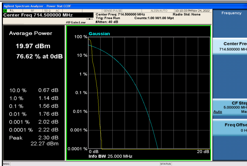
Band12-3MHz-QPSK-23165-1RB#0
