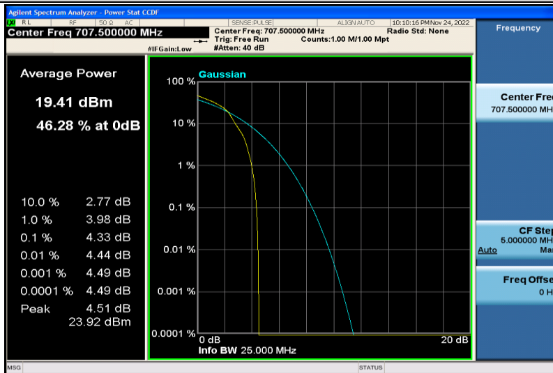
Band12-3MHz-16QAM-23095-1RB#0
