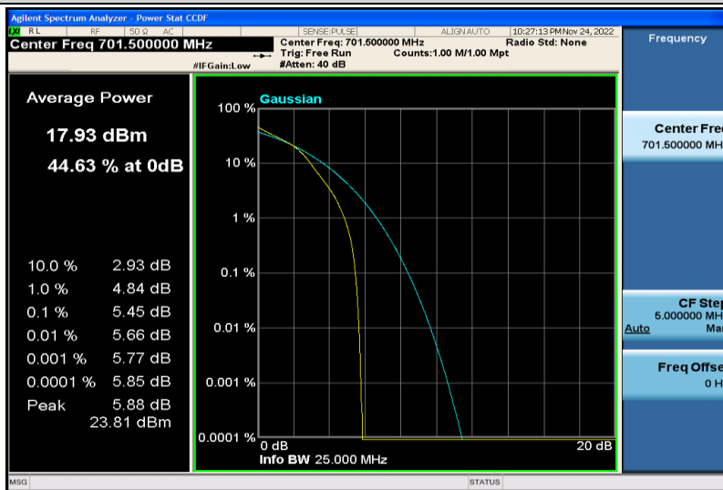
Band12-5MHz-16QAM-23035-25RB#0
