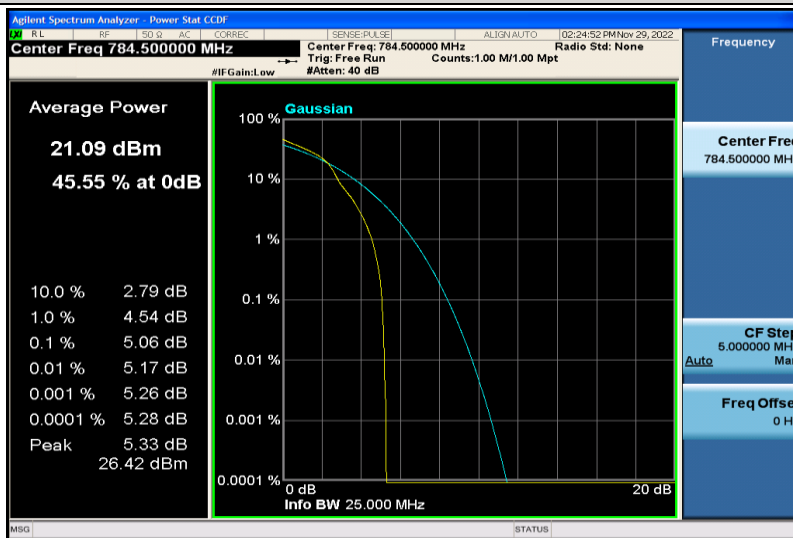
Band13-5MHz-16QAM-23255-1RB#0
