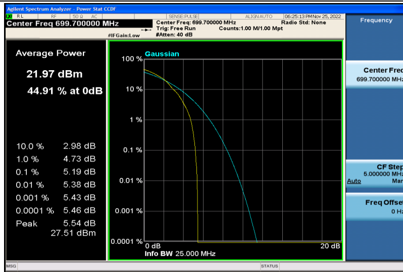
Band12-1.4MHz-64QAM-23017-1RB#0
