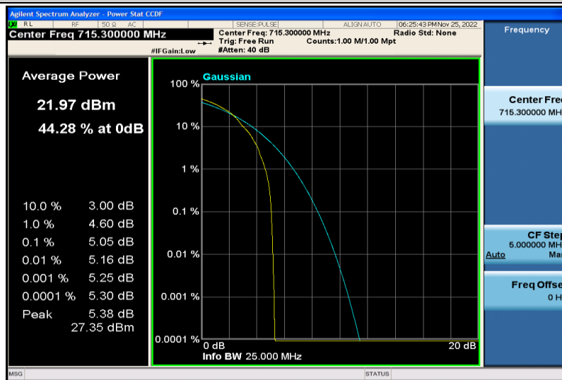
Band12-1.4MHz-64QAM-23173-1RB#0
