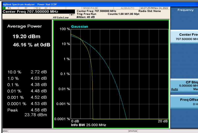
Band12-5MHz-16QAM-23095-1RB#0
