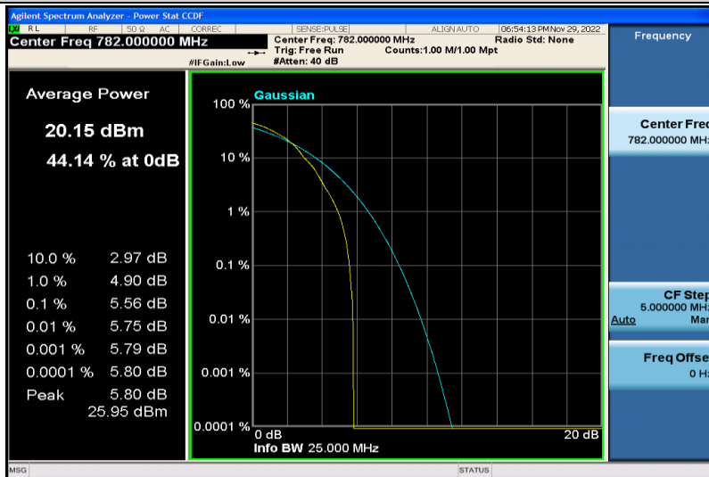
Band13-10MHz-64QAM-23230-1RB#0
