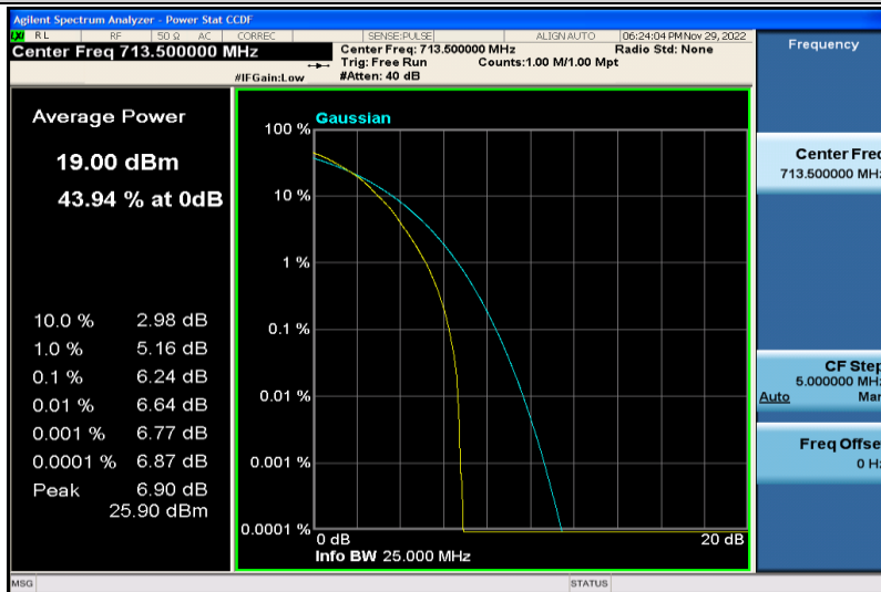
Band12-5MHz-64QAM-23155-25RB#0
