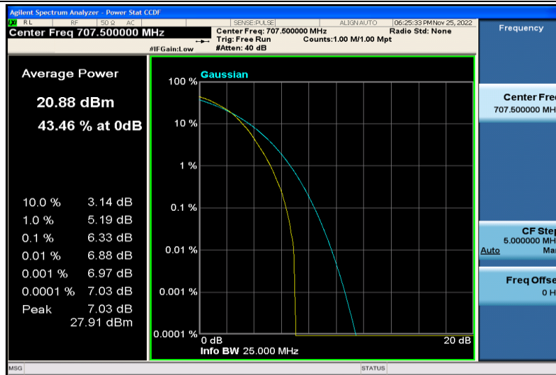
Band12-1.4MHz-64QAM-23095-6RB#0
