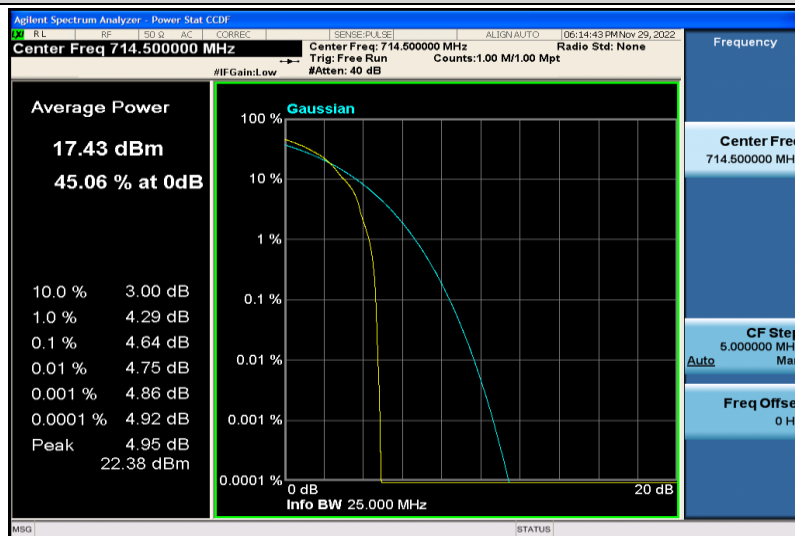
Band12-3MHz-64QAM-23165-1RB#0
