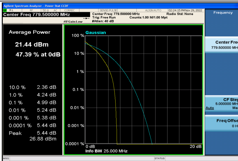
Band13-5MHz-QPSK-23205-25RB#0
