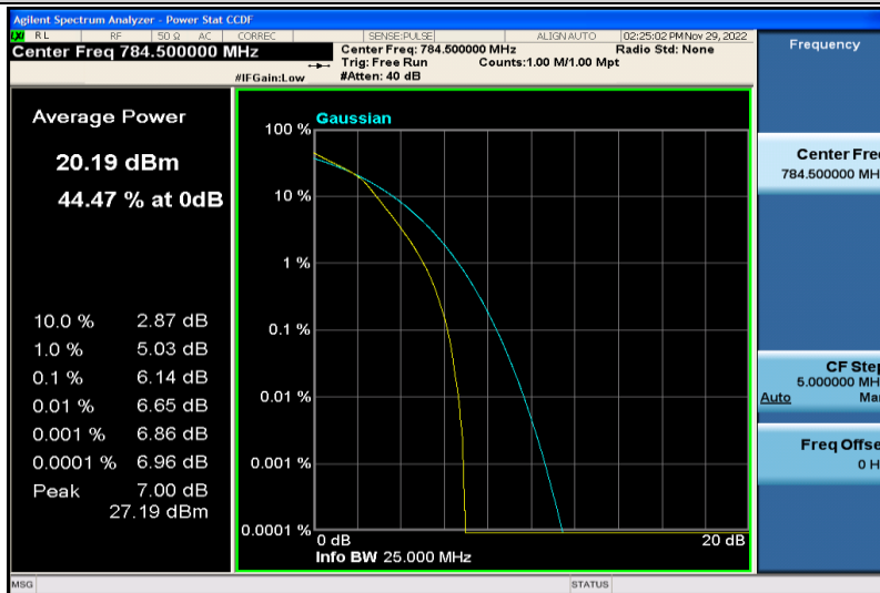
Band13-5MHz-16QAM-23255-25RB#0
