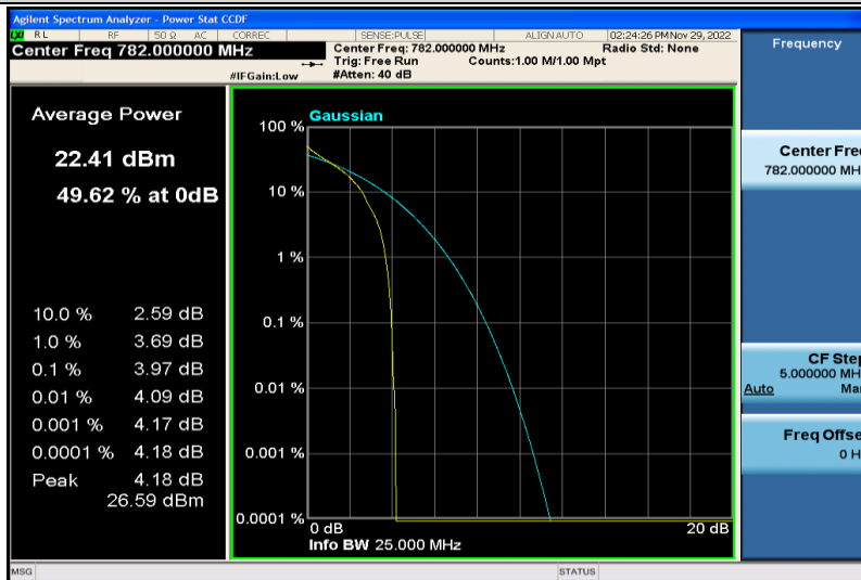
Band13-5MHz-QPSK-23230-1RB#0
