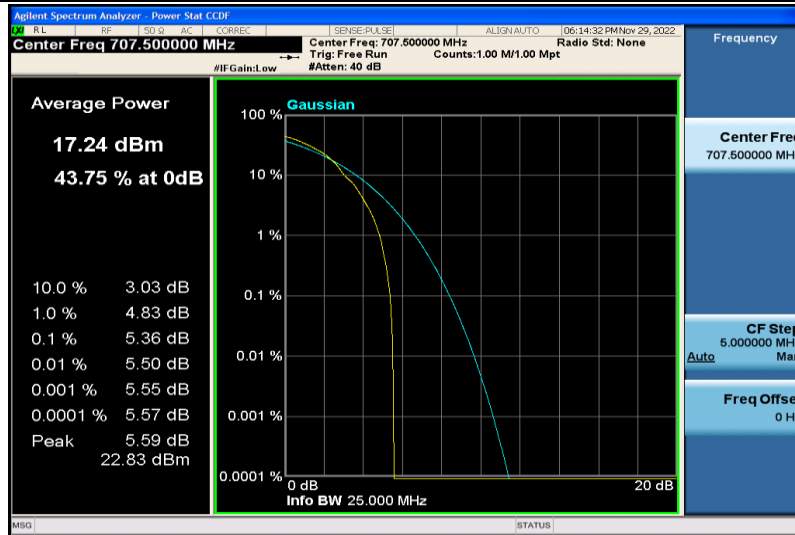
Band12-3MHz-64QAM-23095-1RB#0
