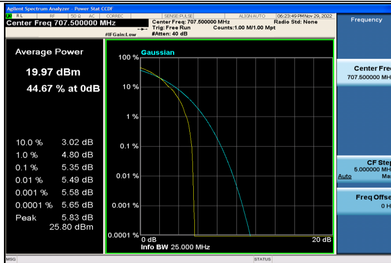
Band12-5MHz-64QAM-23095-1RB#0
