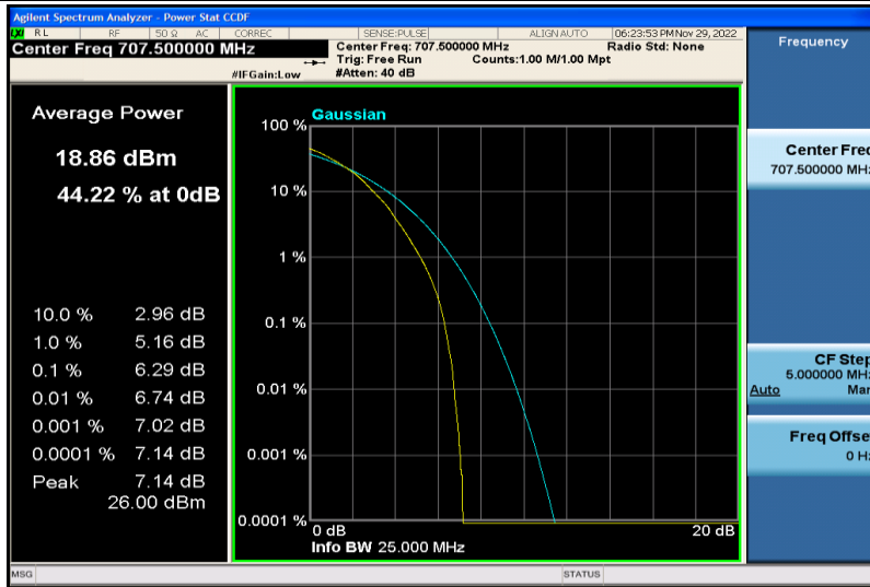
Band12-5MHz-64QAM-23095-25RB#0
