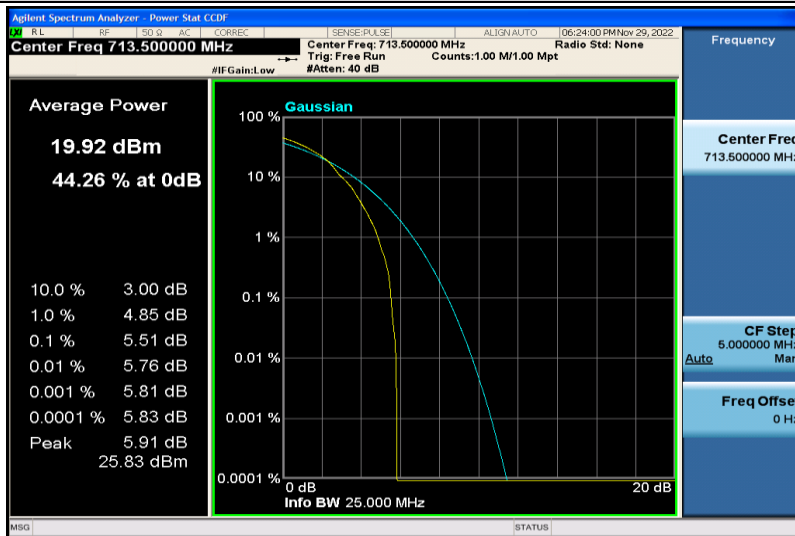
Band12-5MHz-64QAM-23155-1RB#0
