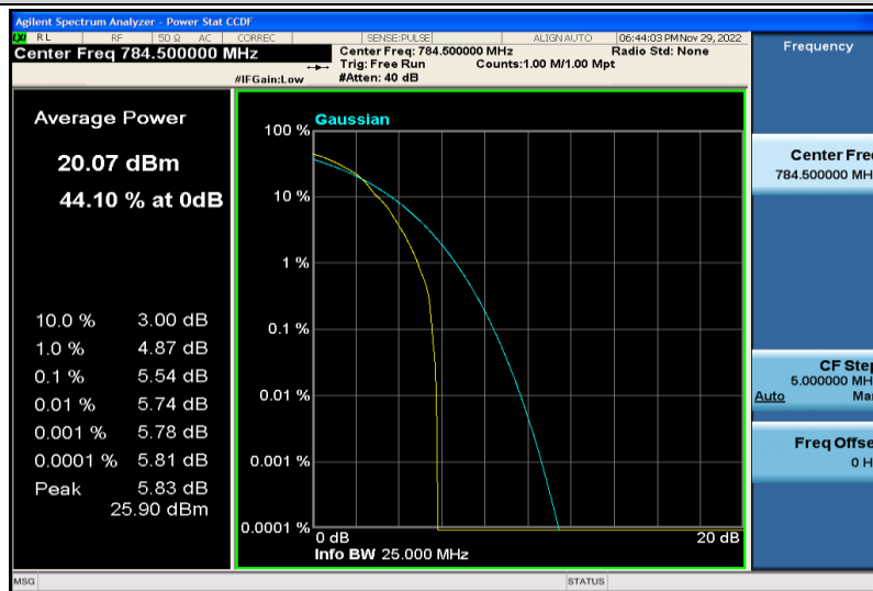
Band13-5MHz-64QAM-23255-1RB#0
