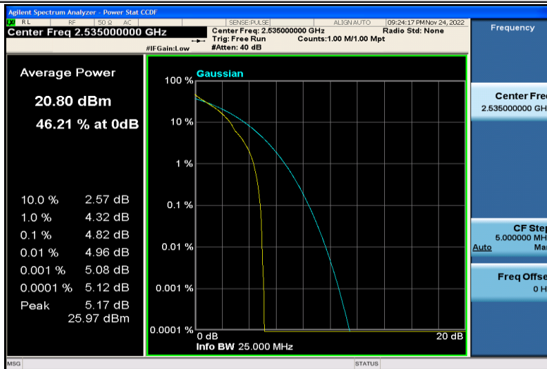
Band7-20MHz-QPSK-21100-1RB#0
