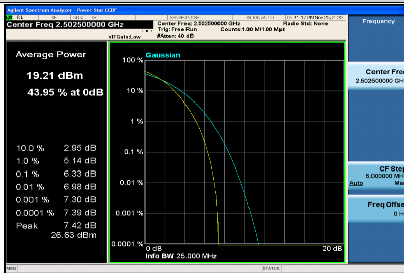
Band7-5MHz-64QAM-20775-25RB#0
