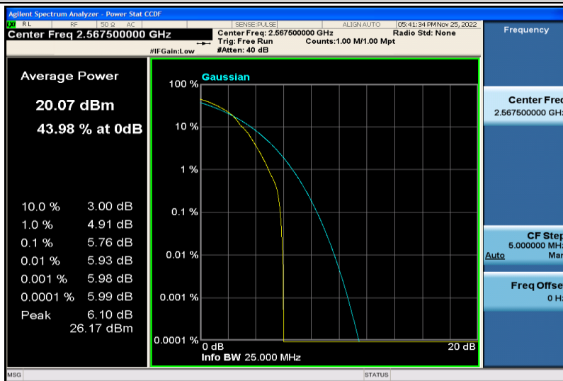
Band7-5MHz-64QAM-21425-1RB#0
