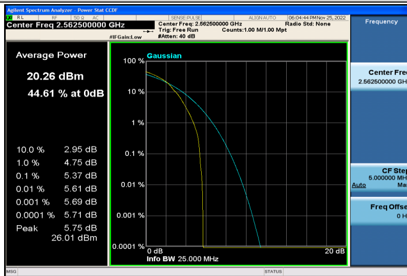
Band7-15MHz-64QAM-21375-1RB#0
