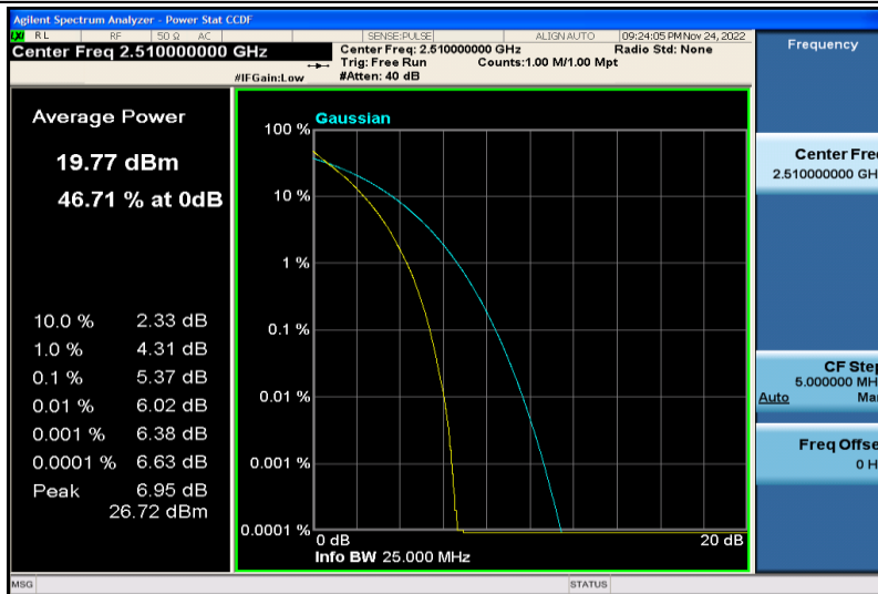
Band7-20MHz-QPSK-20850-100RB#0
