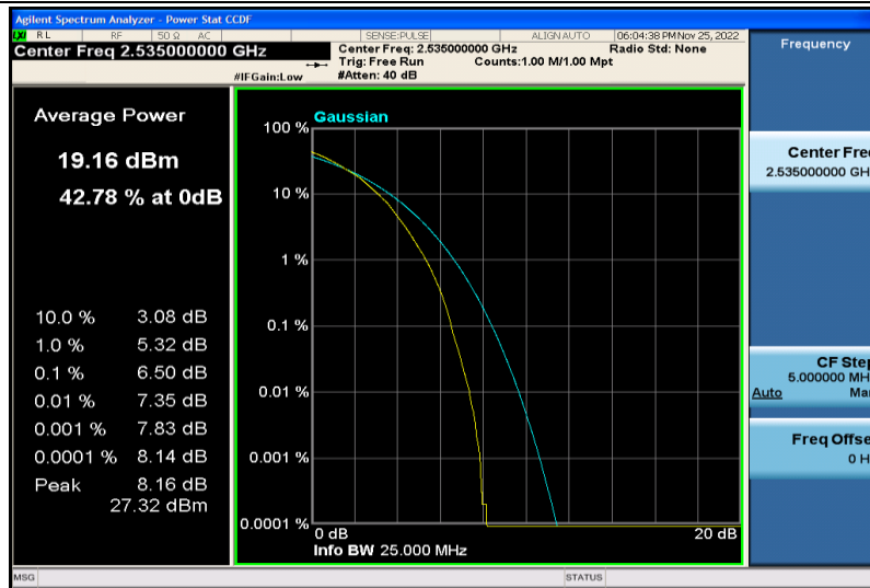
Band7-15MHz-64QAM-21100-75RB#0
