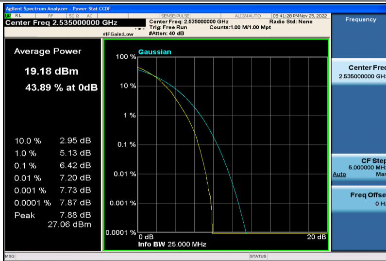
Band7-5MHz-64QAM-21100-25RB#0
