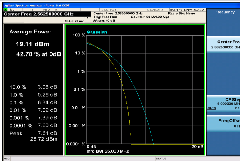
Band7-15MHz-64QAM-21375-75RB#0
