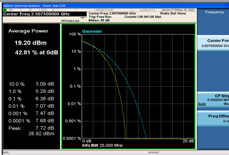
Band7-15MHz-64QAM-20825-75RB#0
