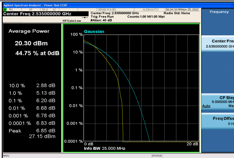
Band7-15MHz-64QAM-21100-1RB#0
