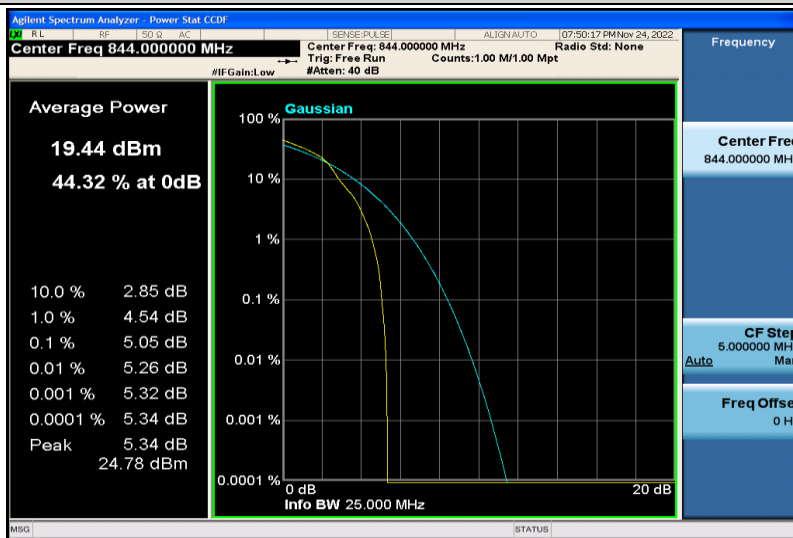
Band5-10MHz-16QAM-20600-1RB#0
