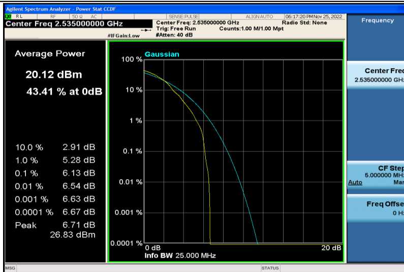
Band7-20MHz-64QAM-21100-1RB#0
