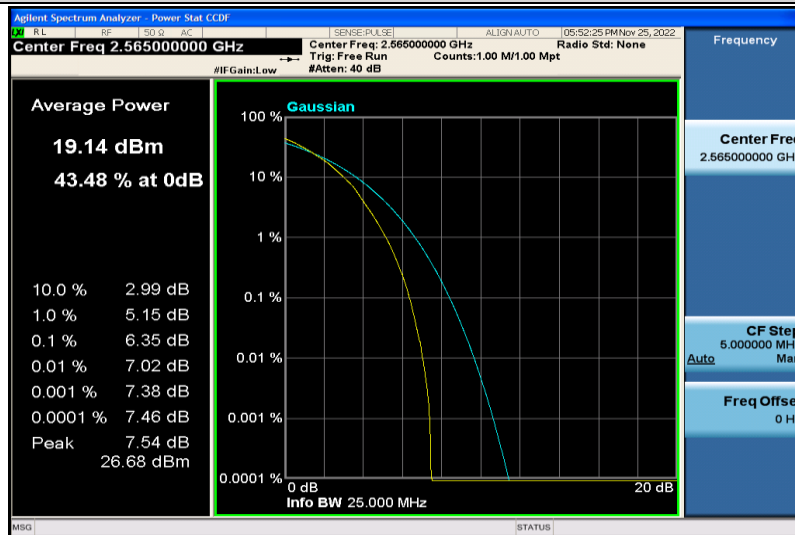
Band7-10MHz-64QAM-21400-50RB#0
