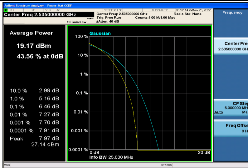
Band7-10MHz-64QAM-21100-50RB#0
