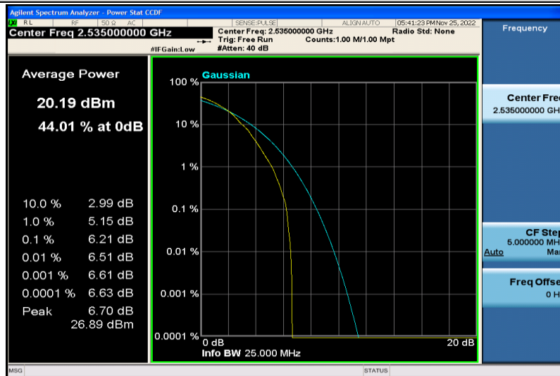
Band7-5MHz-64QAM-21100-1RB#0
