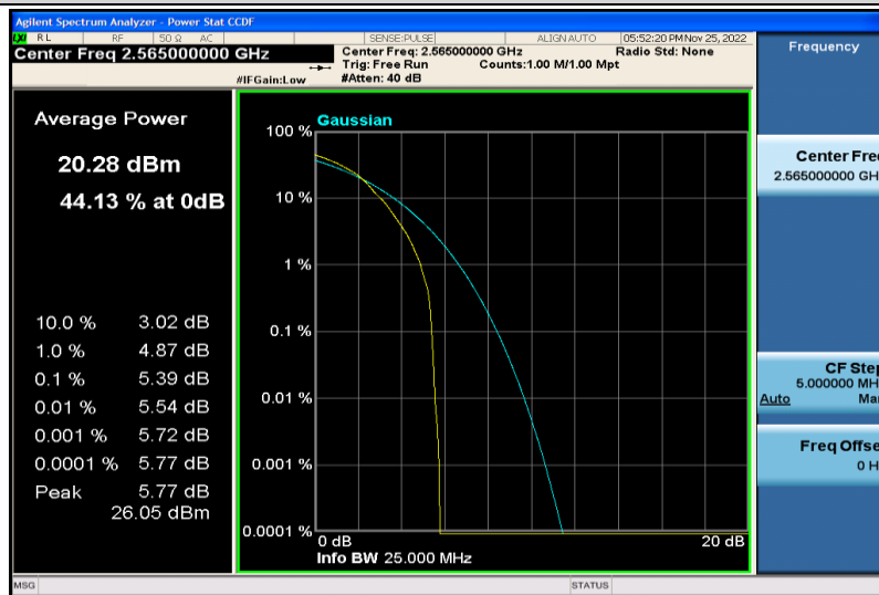
Band7-10MHz-64QAM-21400-1RB#0
