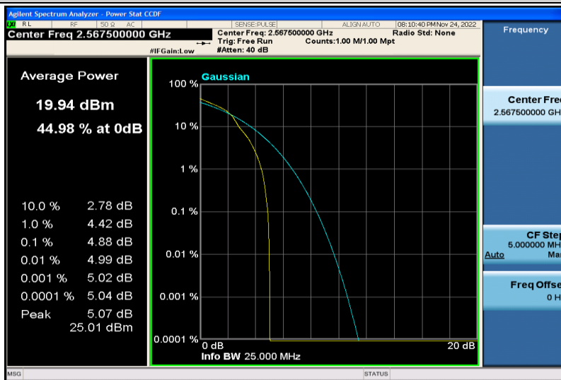
Band7-5MHz-16QAM-21425-1RB#0
