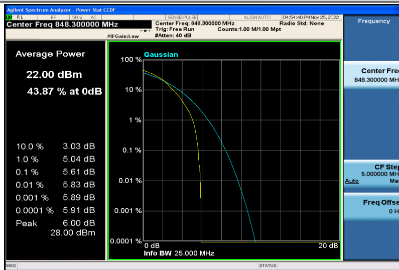
Band5-1.4MHz-64QAM-20643-1RB#0
