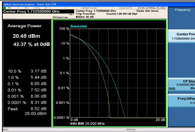
Band4-15MHz-64QAM-20175-75RB#0
