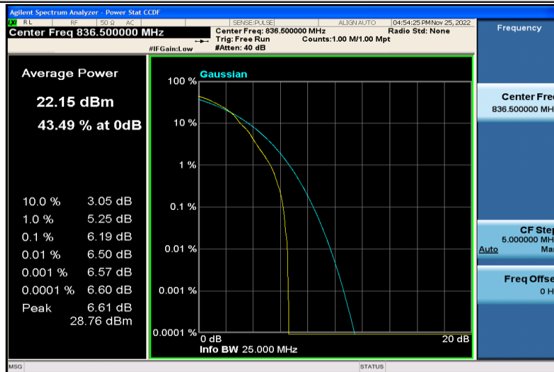
Band5-1.4MHz-64QAM-20525-1RB#0
