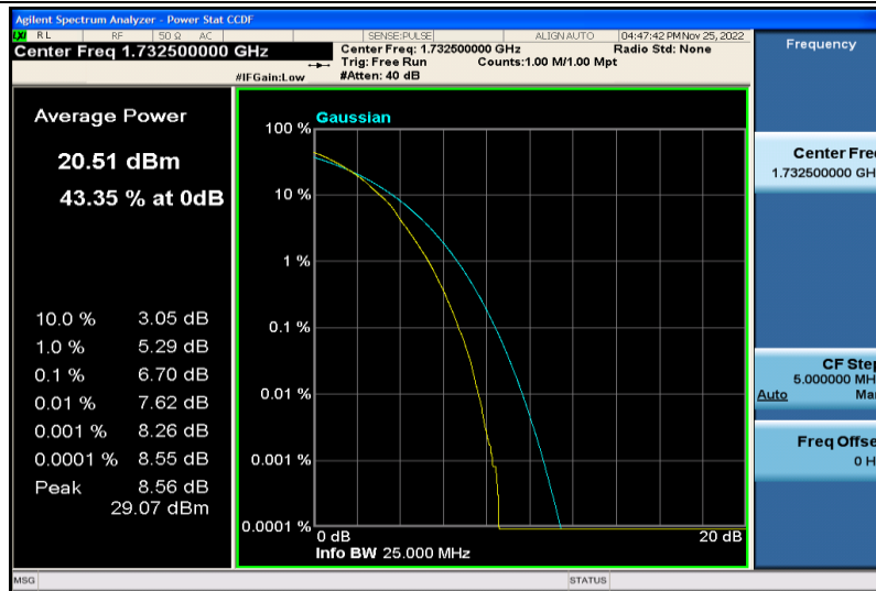
Band4-20MHz-64QAM-20175-100RB#0
