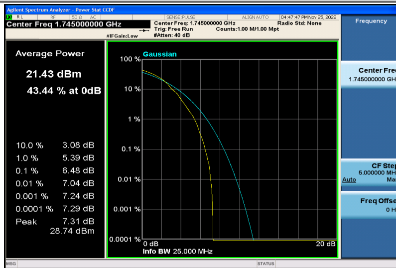
Band4-20MHz-64QAM-20300-1RB#0
