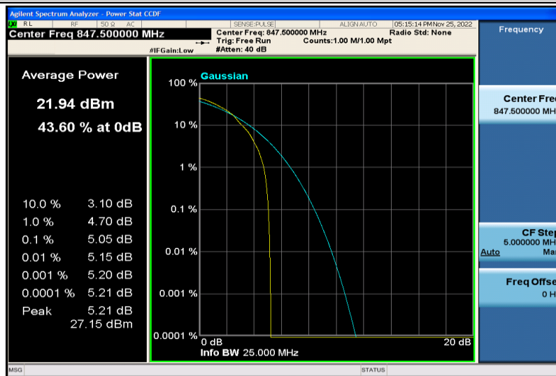
Band5-3MHz-64QAM-20635-1RB#0
