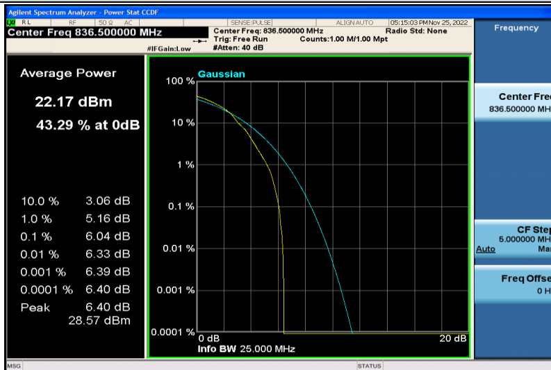
Band5-3MHz-64QAM-20525-1RB#0
