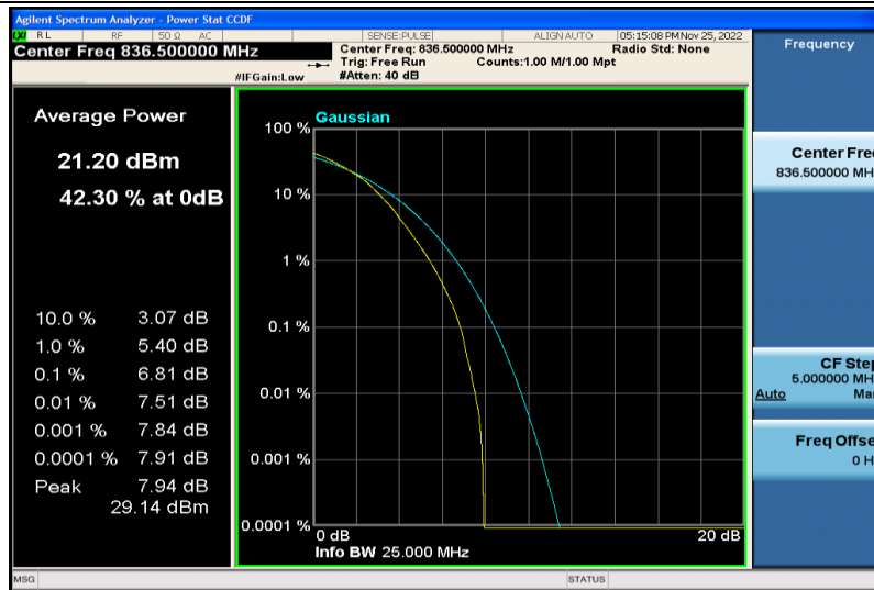
Band5-3MHz-64QAM-20525-15RB#0
