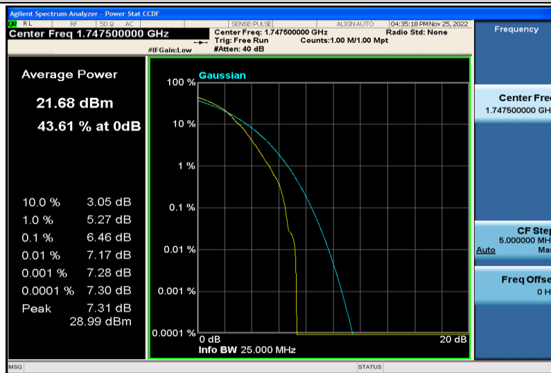
Band4-15MHz-64QAM-20325-1RB#0
