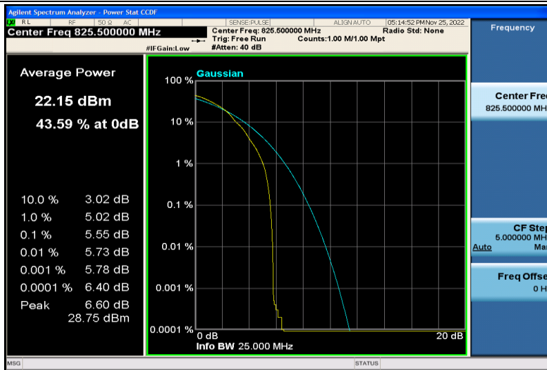
Band5-3MHz-64QAM-20415-1RB#0
