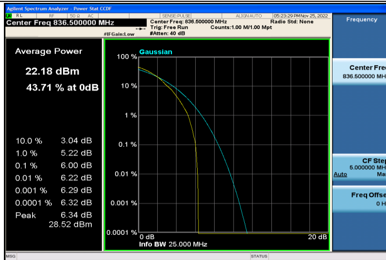
Band5-5MHz-64QAM-20525-1RB#0
