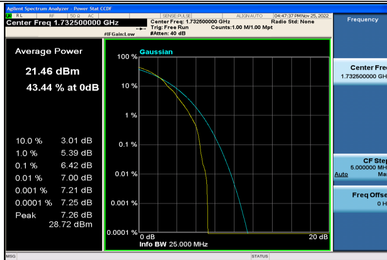
Band4-20MHz-64QAM-20175-1RB#0
