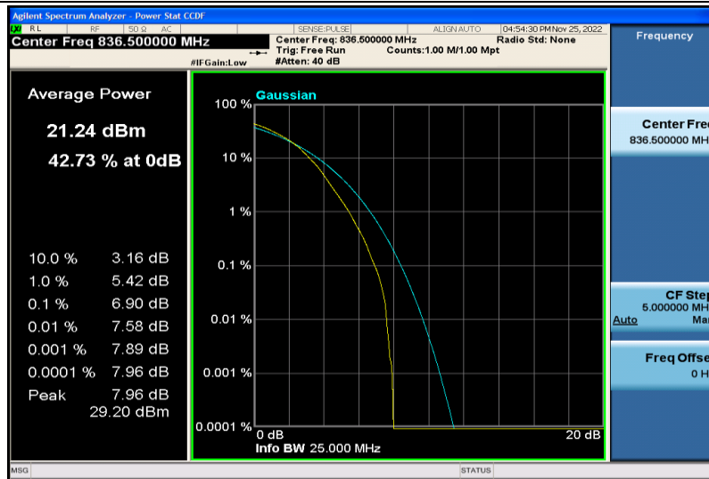
Band5-1.4MHz-64QAM-20525-6RB#0
