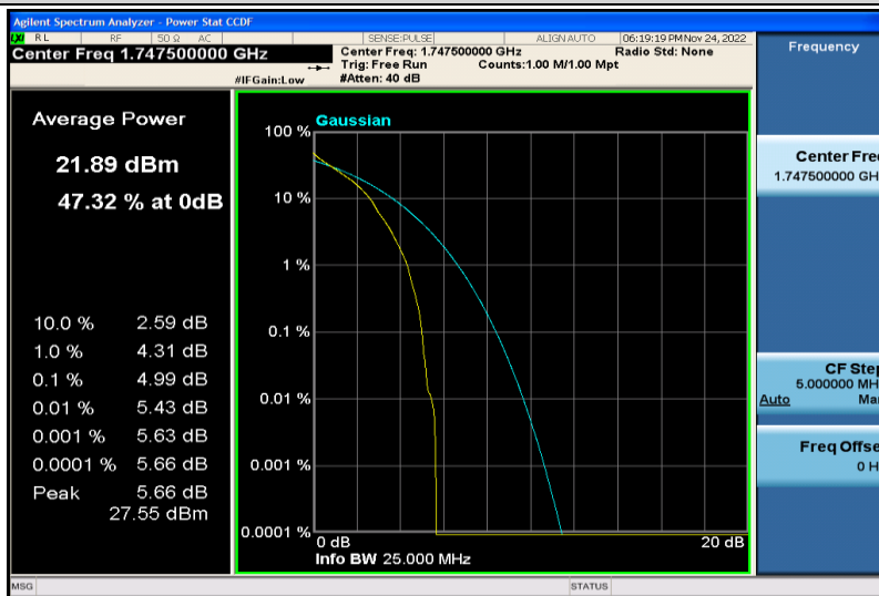
Band4-15MHz-QPSK-20325-1RB#0
