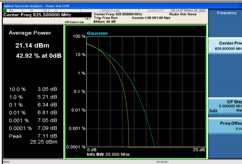
Band5-3MHz-64QAM-20415-15RB#0
