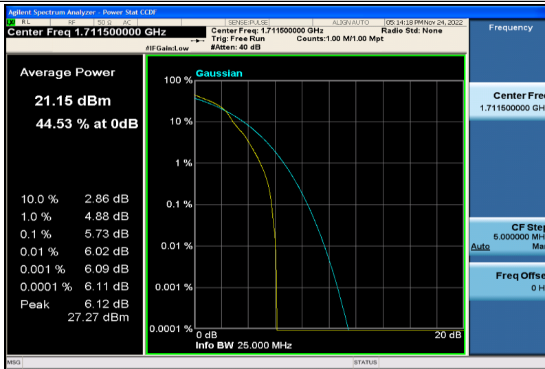
Band4-3MHz-16QAM-19965-1RB#0
