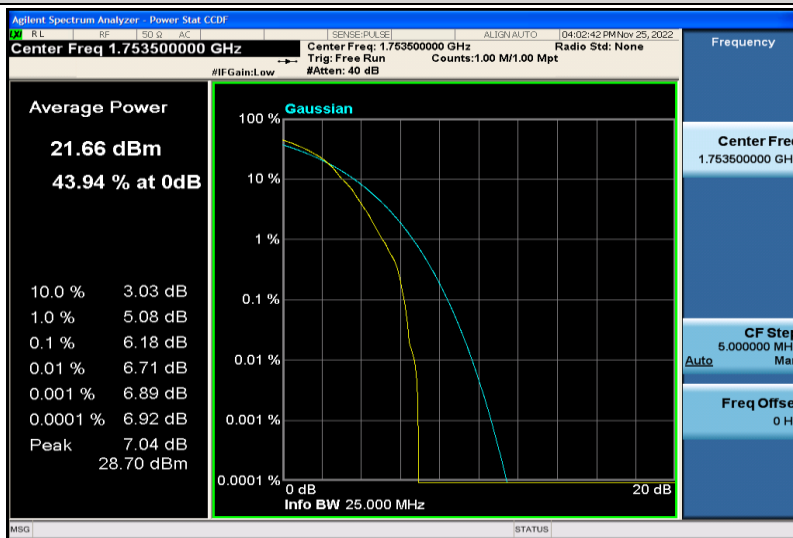
Band4-3MHz-64QAM-20385-1RB#0
