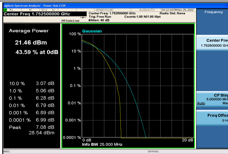
Band4-5MHz-64QAM-20375-1RB#0
