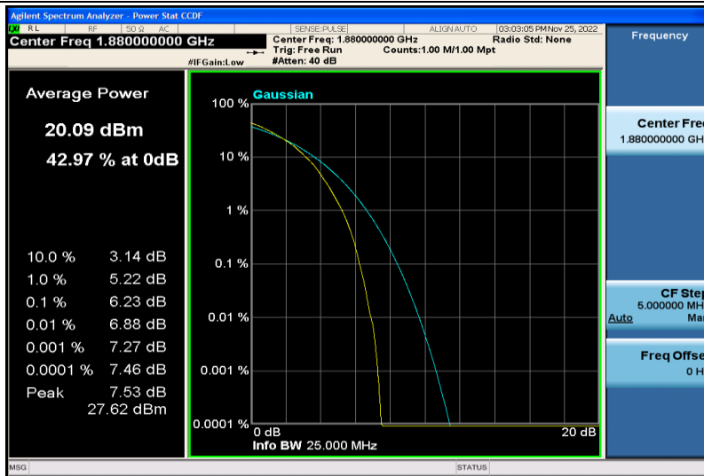
Band2-15MHz-64QAM-18900-75RB#0
