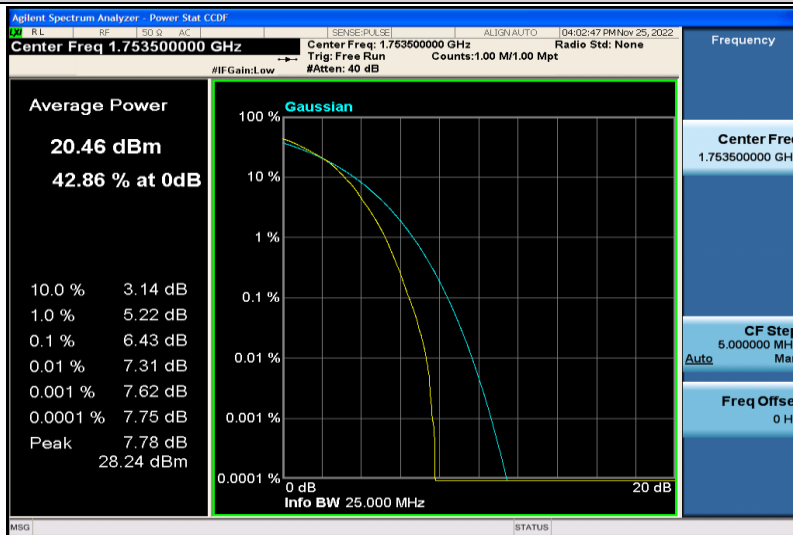
Band4-3MHz-64QAM-20385-15RB#0
