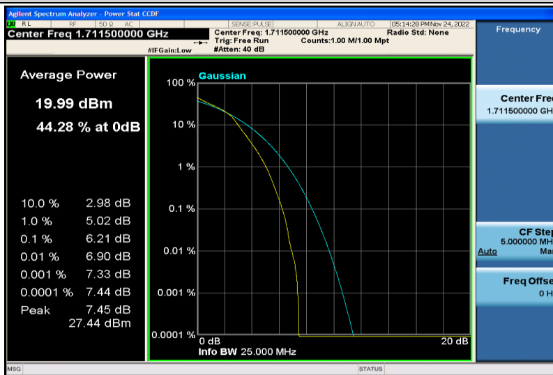
Band4-3MHz-16QAM-19965-15RB#0
