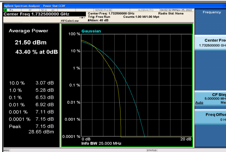
Band4-3MHz-64QAM-20175-1RB#0
