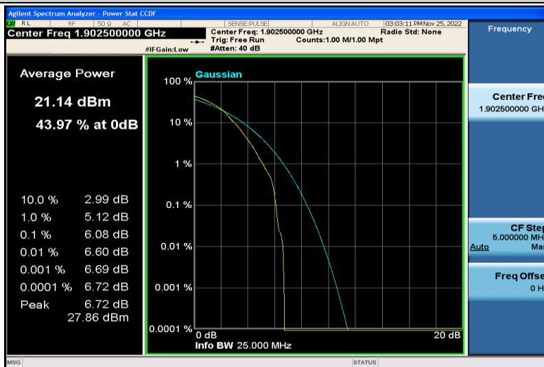
Band2-15MHz-64QAM-19125-1RB#0
