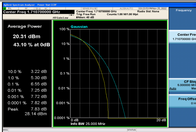
Band4-1.4MHz-64QAM-19957-6RB#0
