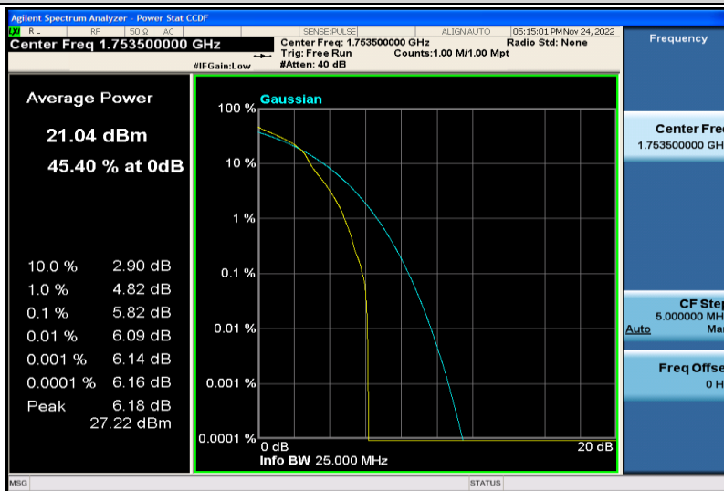
Band4-3MHz-16QAM-20385-1RB#0
