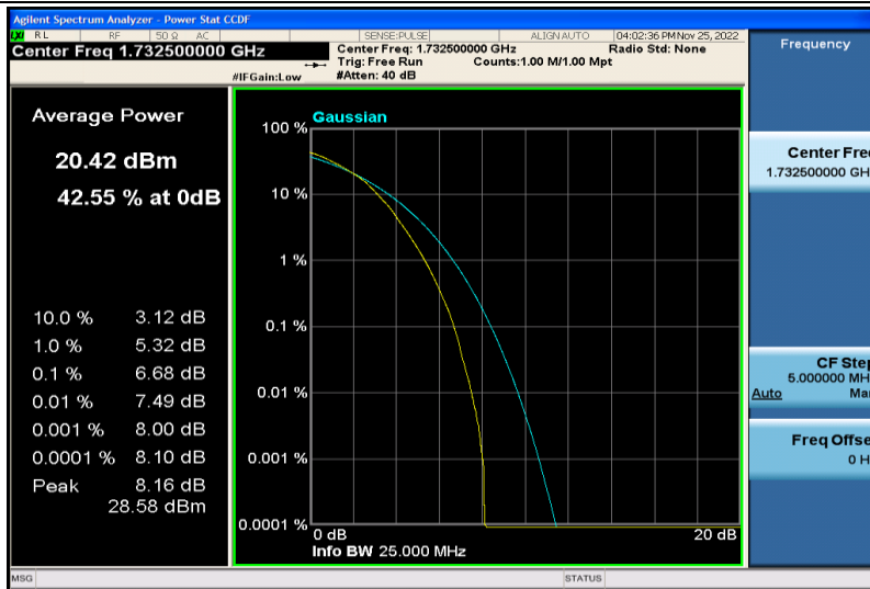
Band4-3MHz-64QAM-20175-15RB#0
