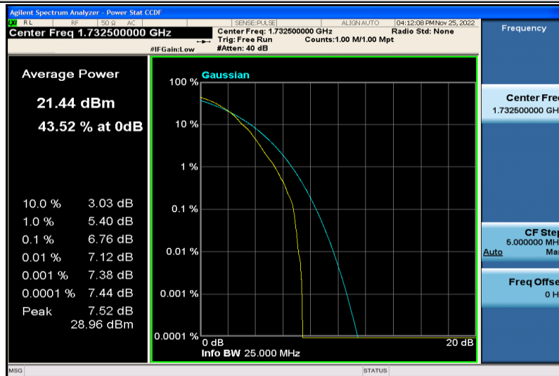
Band4-5MHz-64QAM-20175-1RB#0
