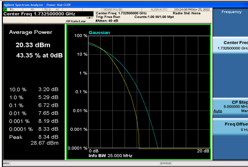
Band4-1.4MHz-64QAM-20175-6RB#0
