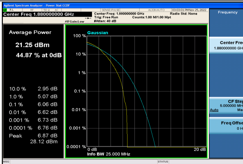
Band2-15MHz-64QAM-18900-1RB#0
