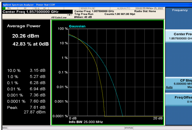
Band2-15MHz-64QAM-18675-75RB#0
