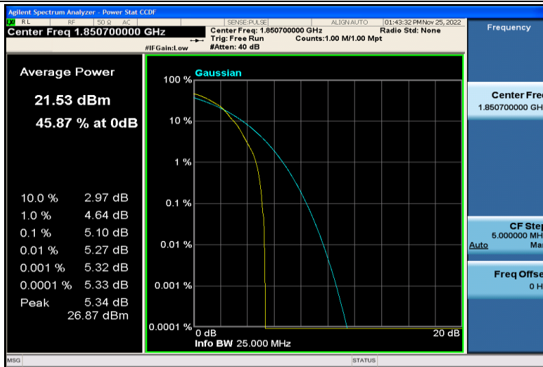
Band2-1.4MHz-64QAM-18607-1RB#0
