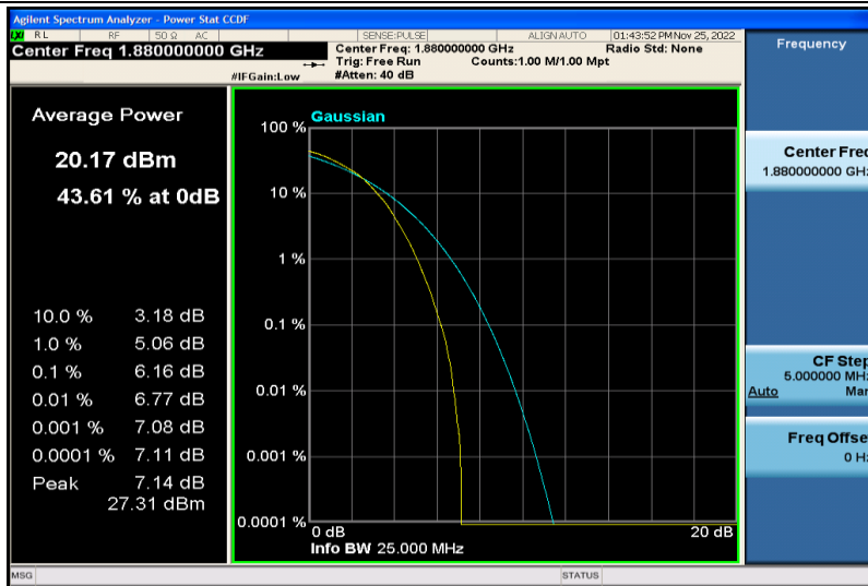
Band2-1.4MHz-64QAM-18900-6RB#0
