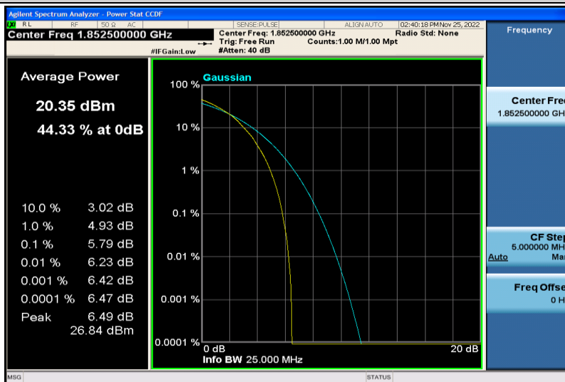
Band2-5MHz-64QAM-18625-25RB#0
