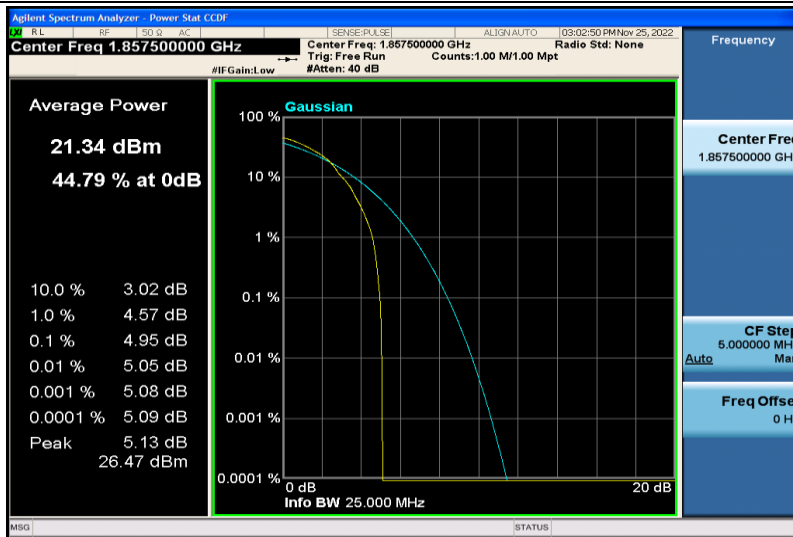
Band2-15MHz-64QAM-18675-1RB#0
