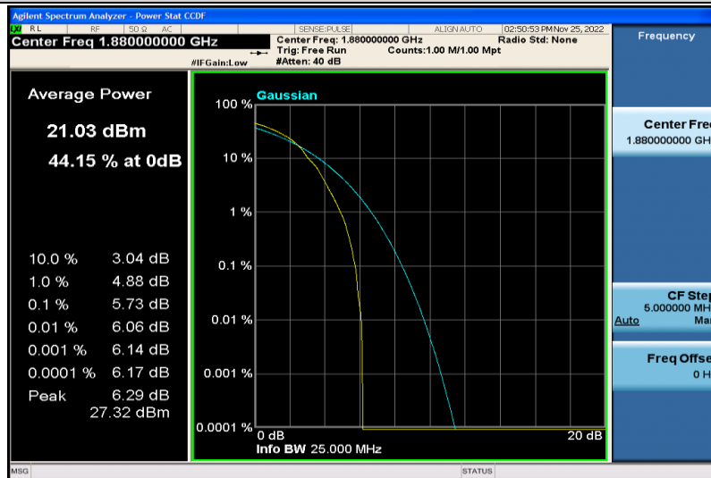
Band2-10MHz-64QAM-18900-1RB#0
