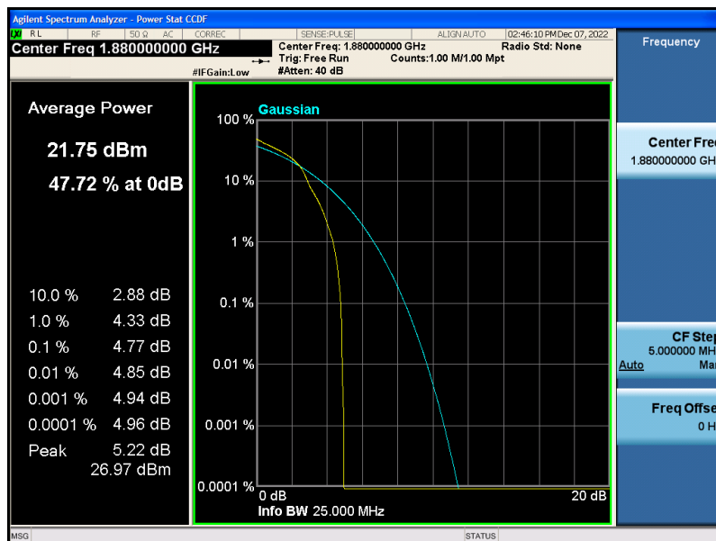
Band2-1.4MHz-16QAM-18900-1RB#0
