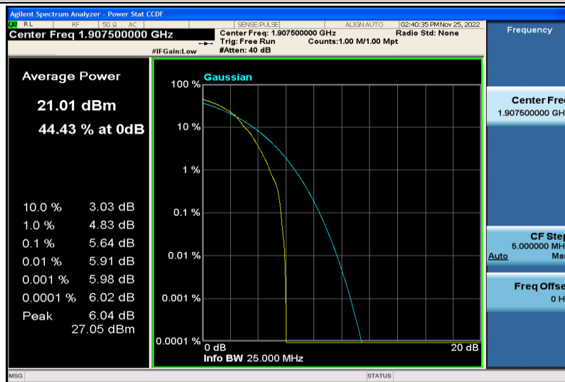
Band2-5MHz-64QAM-19175-1RB#0
