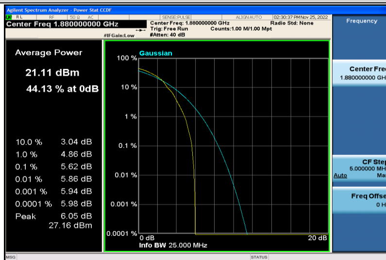
Band2-3MHz-64QAM-18900-1RB#0
