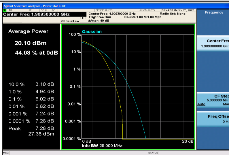
Band2-1.4MHz-64QAM-19193-6RB#0
