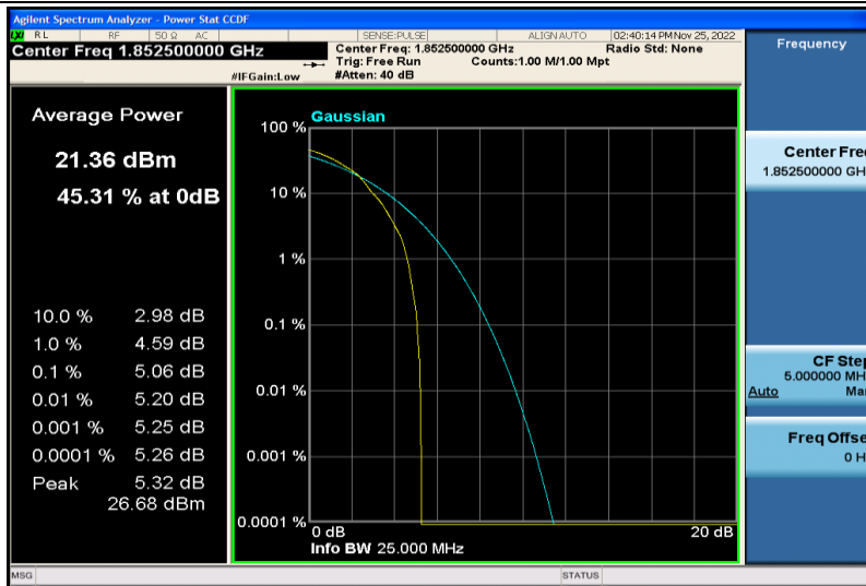
Band2-5MHz-64QAM-18625-1RB#0
