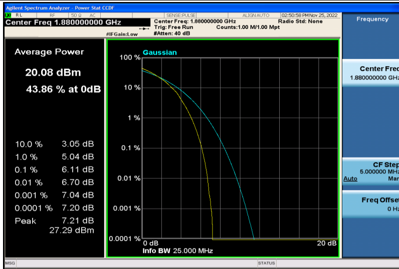
Band2-10MHz-64QAM-18900-50RB#0
