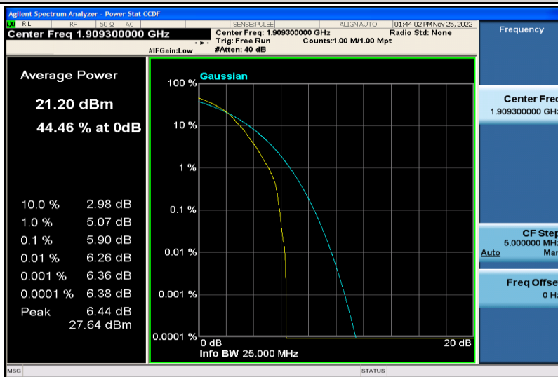
Band2-1.4MHz-64QAM-19193-1RB#0
