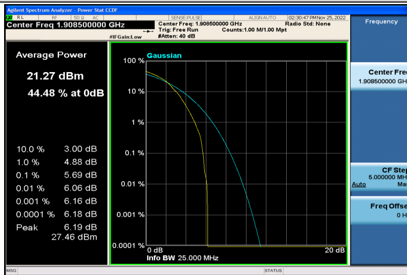
Band2-3MHz-64QAM-19185-1RB#0
