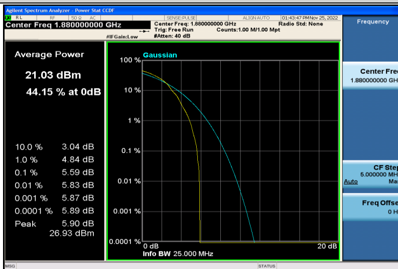
Band2-1.4MHz-64QAM-18900-1RB#0
