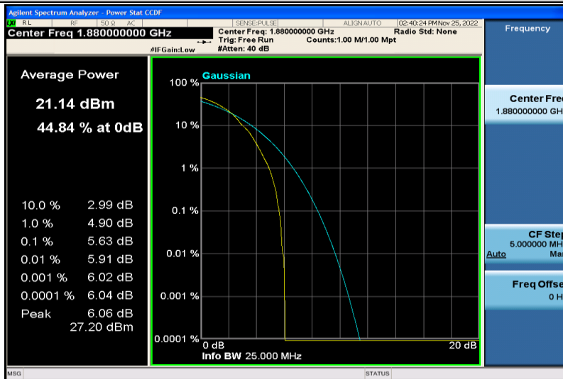
Band2-5MHz-64QAM-18900-1RB#0
