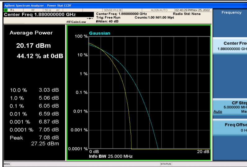
Band2-5MHz-64QAM-18900-25RB#0
