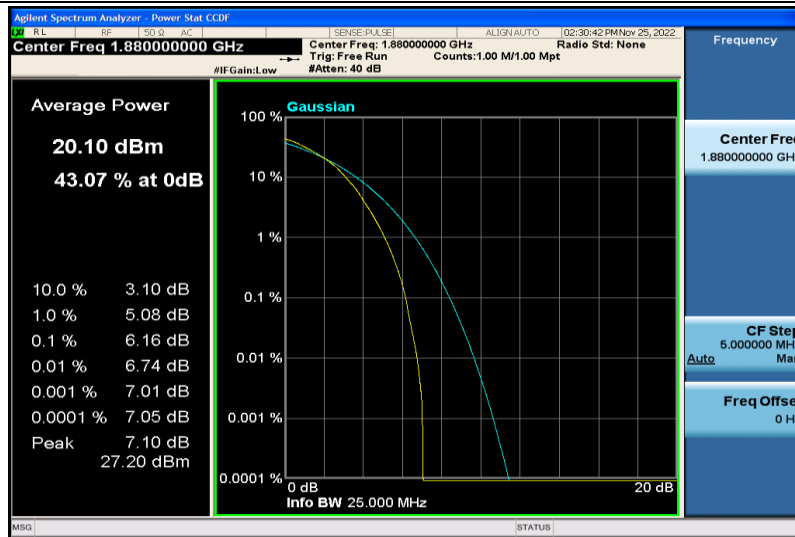
Band2-3MHz-64QAM-18900-15RB#0
