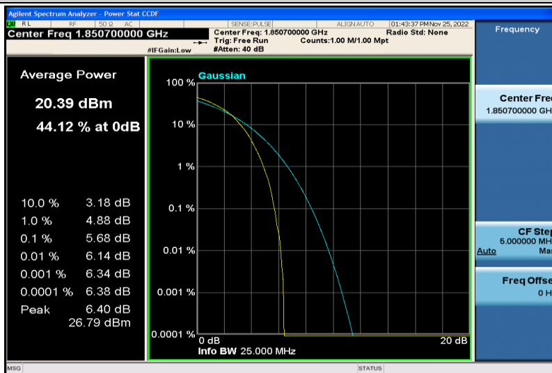
Band2-1.4MHz-64QAM-18607-6RB#0
