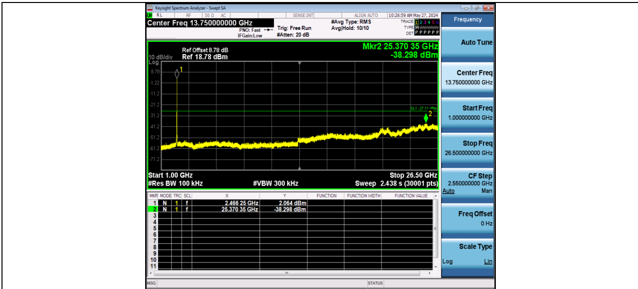
11AX20MIMO Ant2_2462_26Tone_RU8_0~Reference
