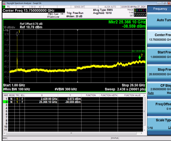
11AX20MIMO Ant2 2437 26Tone RU4 0~Reference
