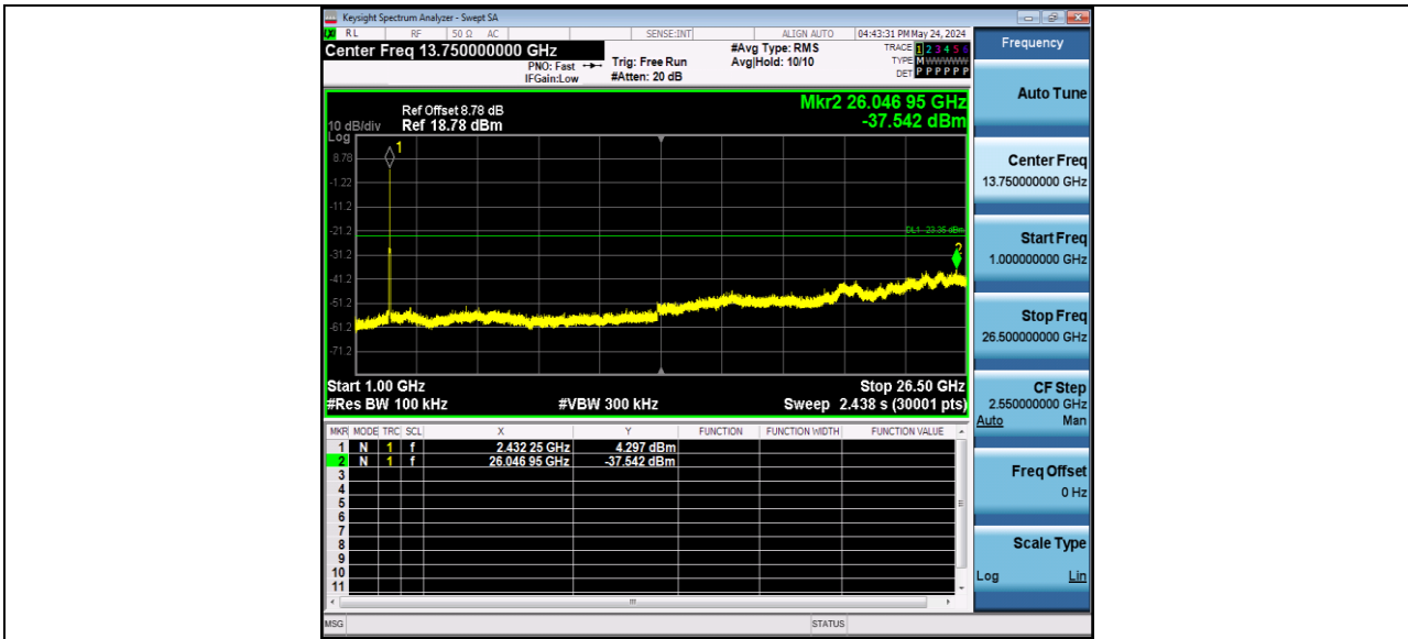
11G-CDD Ant2_2437_0~Reference
