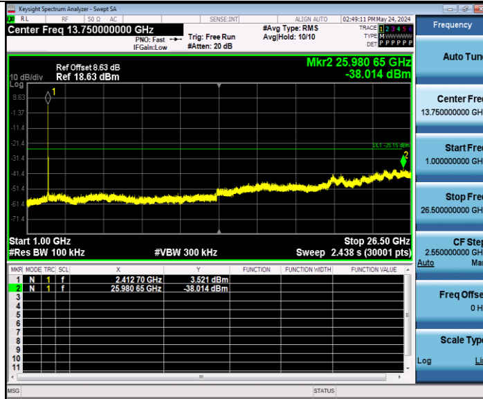
11B-CDD Ant2_2412_0~Reference
