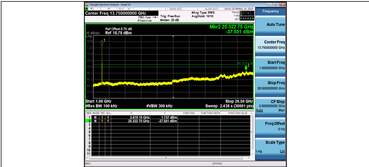
11G-CDD_Ant2_2412_0~Reference
