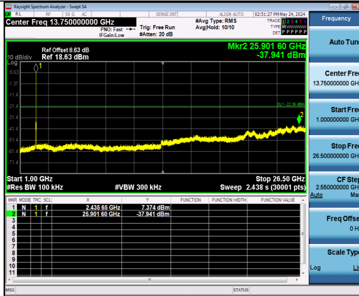
11B-CDD Ant2_2437_0~Reference
