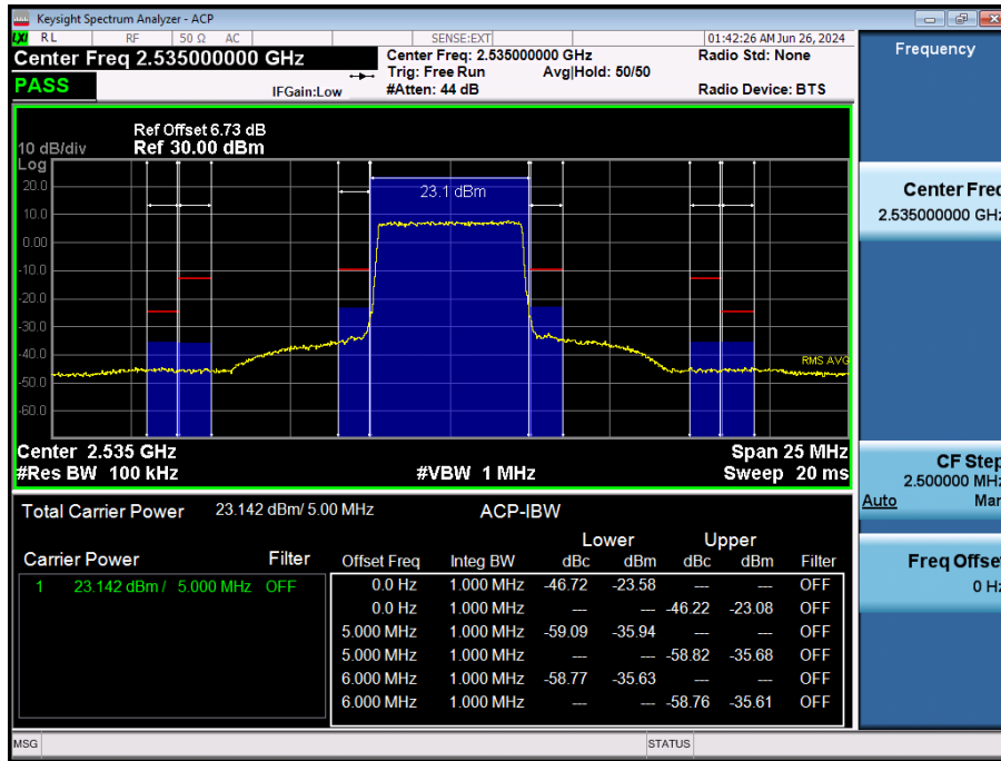
LTE Band 7 / 5MHz / QPSK - RB Size/Offset (Full RB)
