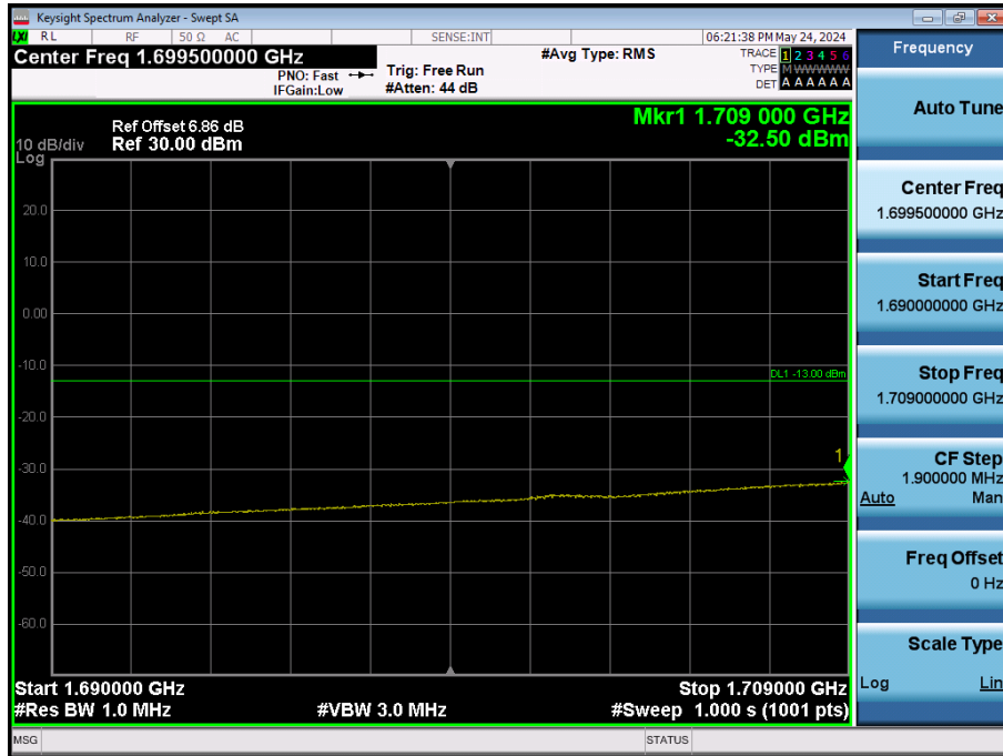
LTE Band 66 / 20MHz / 16QAM - RB Size/Offset (100/0)
