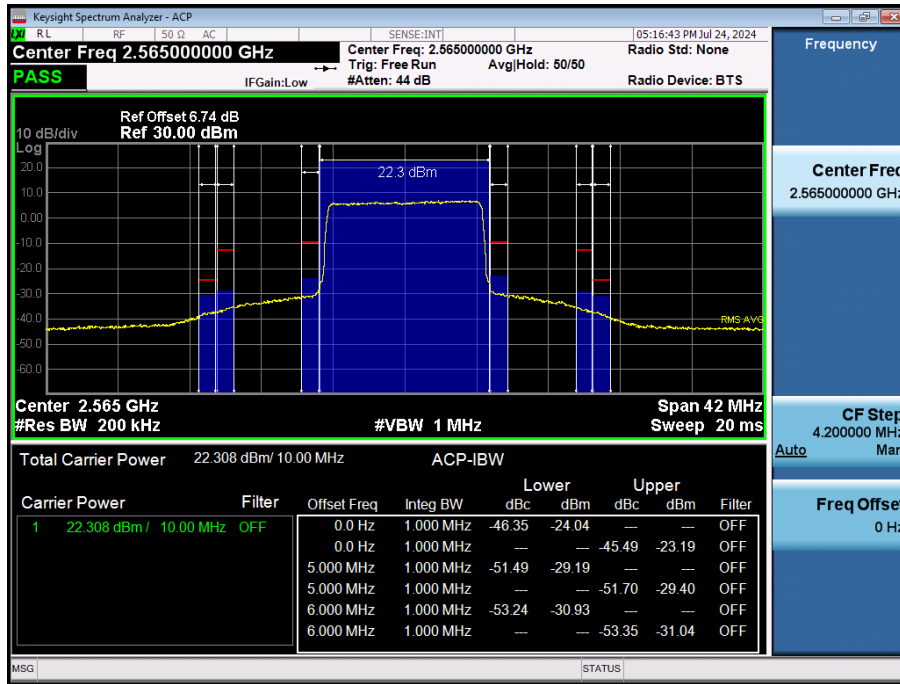
LTE Band 7 / 10MHz / 16QAM - RB Size/Offset (Full RB)
