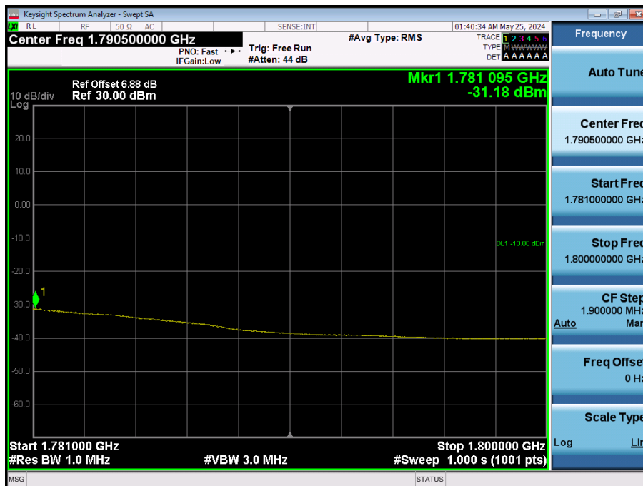
LTE Band 66 / 20MHz / 256QAM - RB Size/Offset (50/50)
