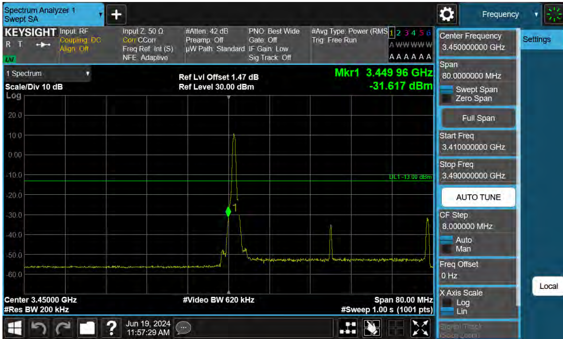
40 MHz / \pi/2 BPSK / RB Size/Offset (1/Edge Left)
