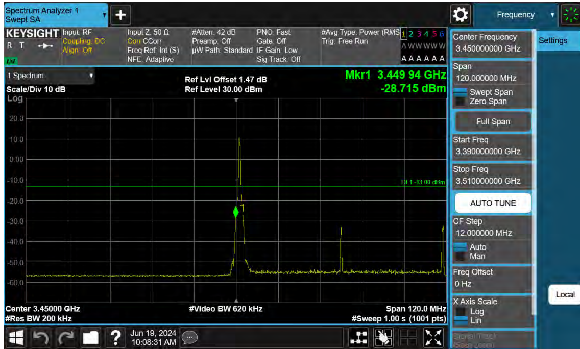
60 MHz / 16QAM / RB Size/Offset (1/Edge Left)
