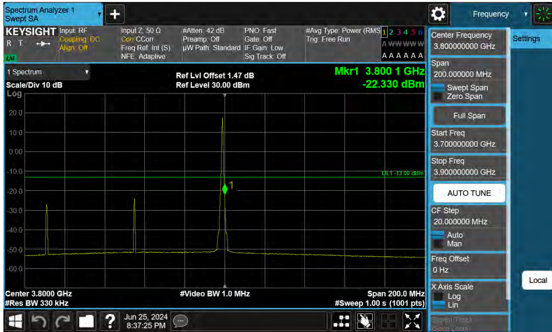
90 MHz / 64QAM / RB Size/Offset (1/Edge Right)
