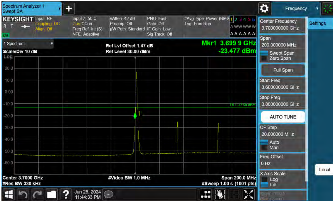
70 MHz / 16QAM / RB Size/Offset (1/Edge Left)
