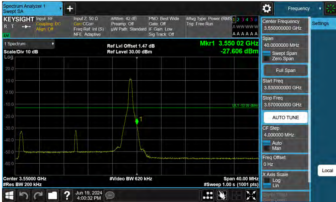
20 MHz / 64QAM / RB Size/Offset (1/Edge Right)
