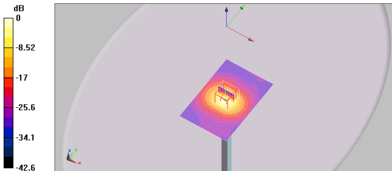
0 dB = 35.4mW/g
