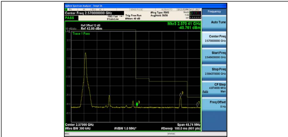
Band7_20MHz_QPSK_21350_100RB#0_-40.92,-37.24,-33.67_PASS
