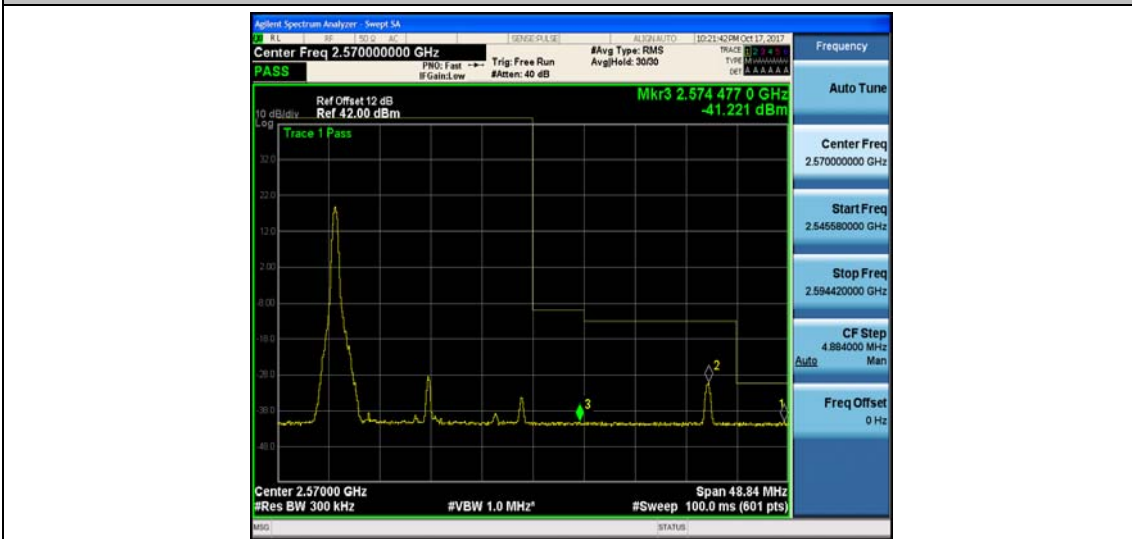
Band7_20MHz_16QAM_21350_1RB#0_-41.22,-30.74,-40.76_PASS
