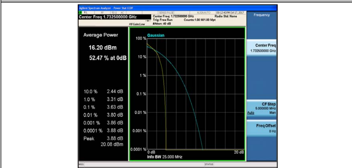
Band4_10MHz_16QAM_20175_1RB#0_4.51_13_PASS
