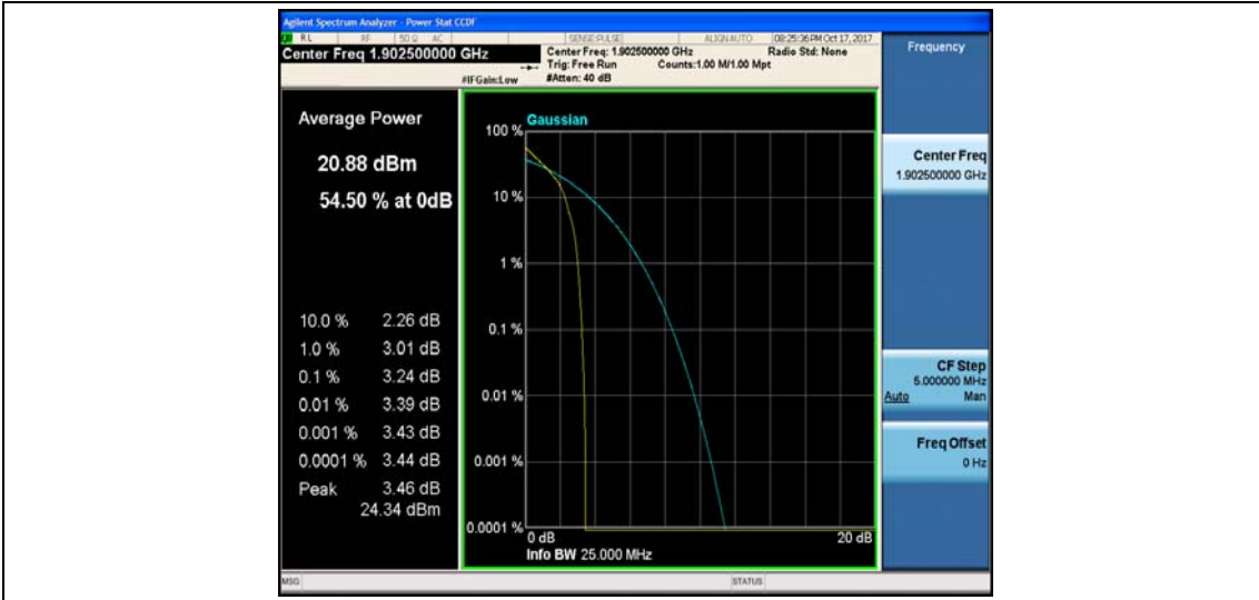
Band2_15MHz_16QAM_19125_1RB#0_4.16_13_PASS
