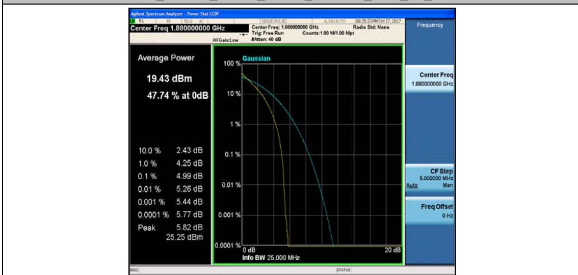
Band2_15MHz_16QAM_18900_75RB#0_5.71_13_PASS
