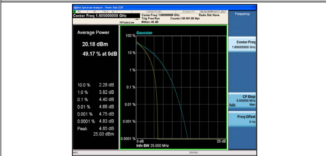
Band2_10MHz_16QAM_19150_50RB#0_5.27_13_PASS
