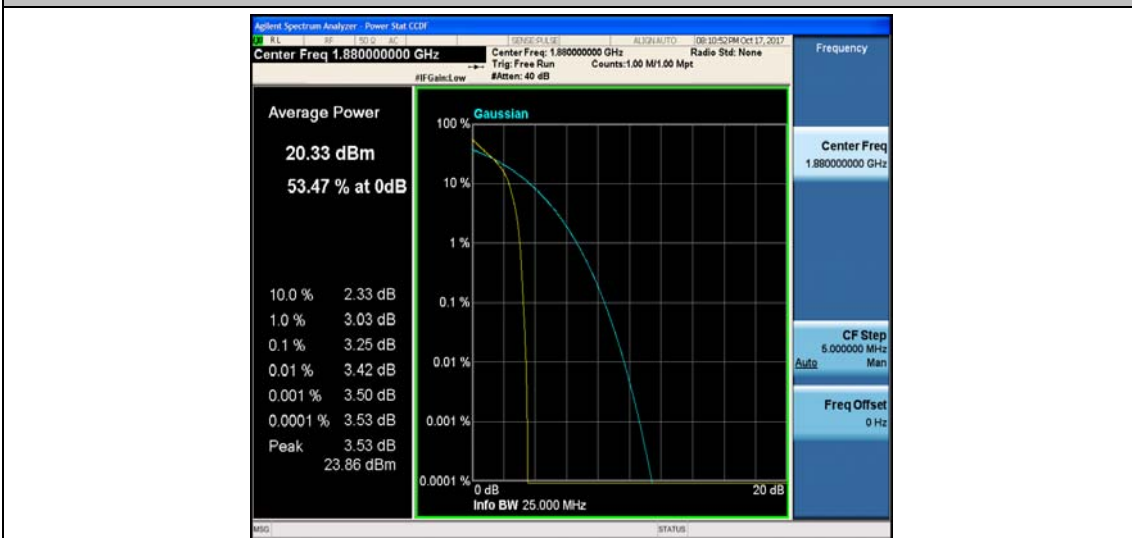
Band2_5MHz_16QAM_18900_1RB#0_4.10_13_PASS
