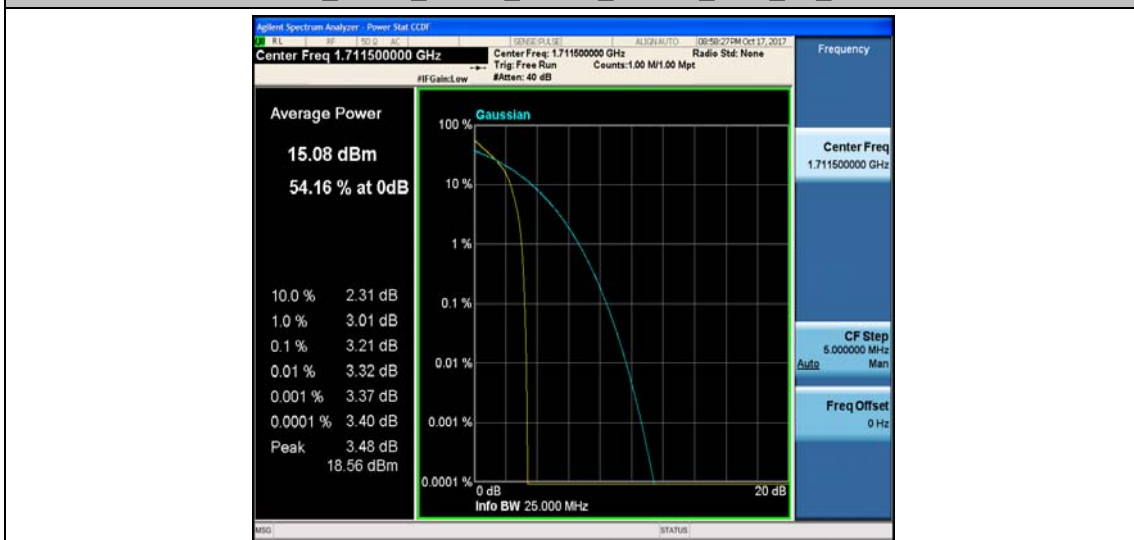
Band4_3MHz_16QAM_19965_1RB#0_4.20_13_PASS
