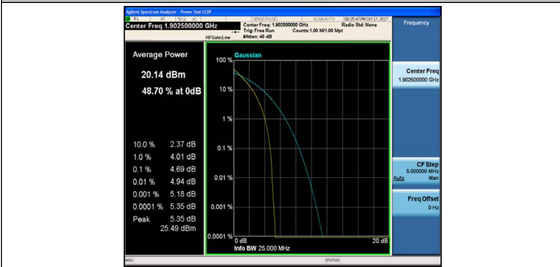
Band2_15MHz_16QAM_19125_75RB#0_5.47_13_PASS
