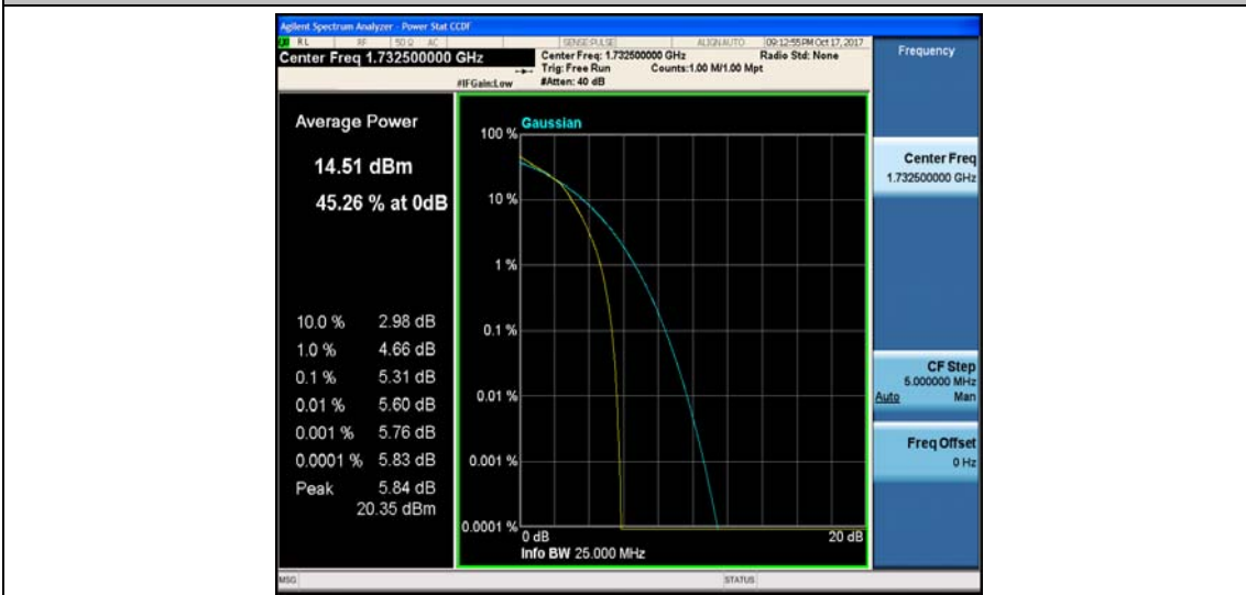
Band4_10MHz_QPSK_20350_1RB#0_3.58_13_PASS
