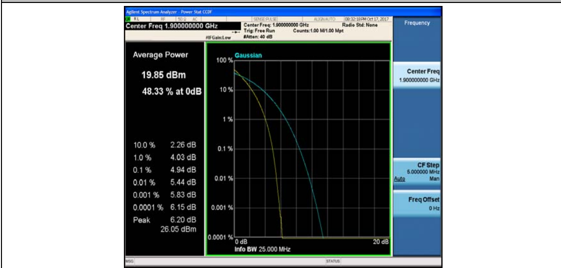
Band2_20MHz_16QAM_19100_100RB#0_5.71_13_PASS
