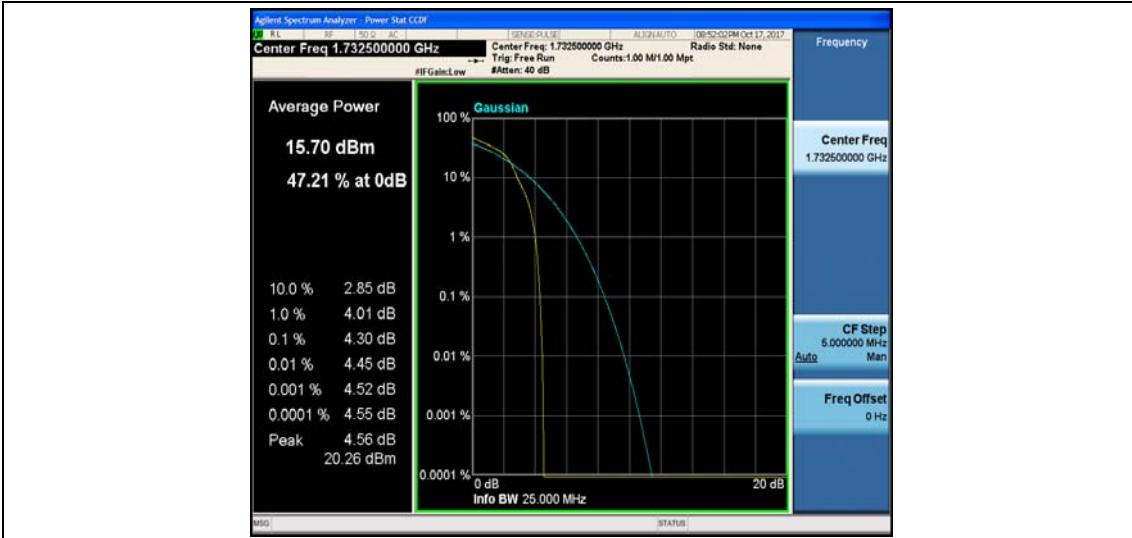
Band4_1.4MHz_QPSK_20175_6RB#0_4.33_13_PASS
