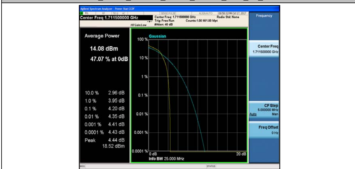
Band4_3MHz_QPSK_19965_15RB#0_4.48_13_PASS
