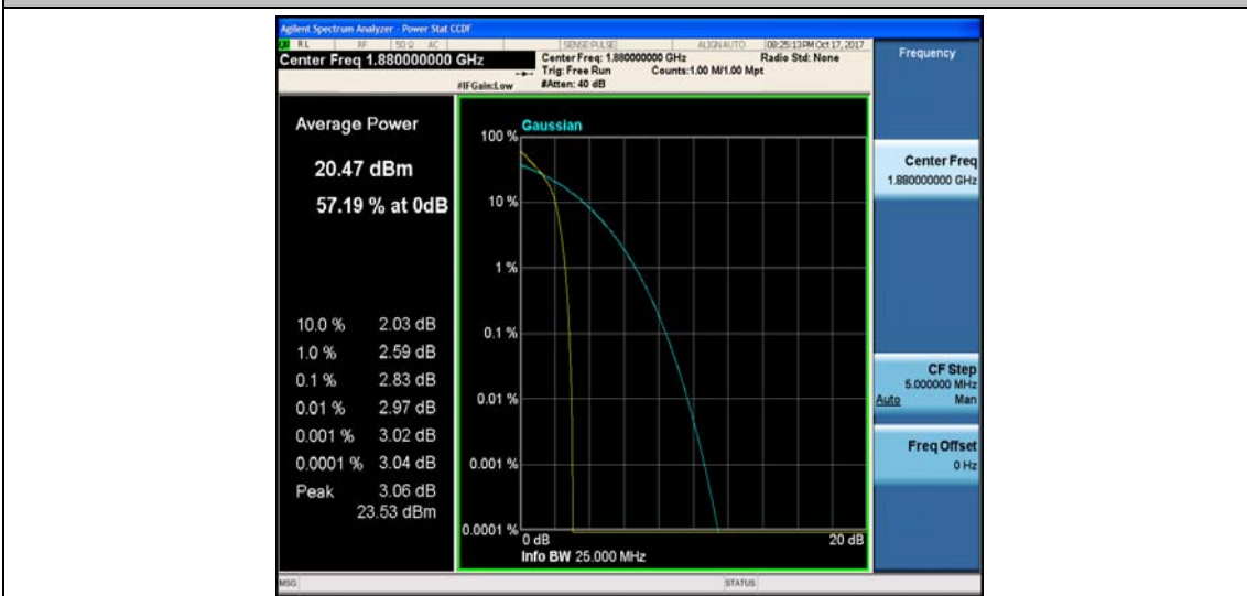
Band2_15MHz_16QAM_18900_1RB#0_3.86_13_PASS
