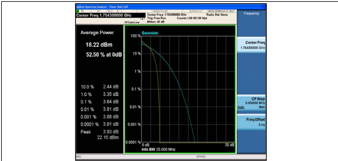
Band4_1.4MHz_16QAM_20393_1RB#0_4.58_13_PASS
