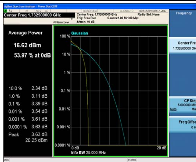
Band4_1.4MHz_16QAM_20175_1RB#0_4.30_13_PASS
