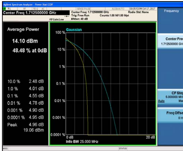
Band4_5MHz_16QAM_19975_25RB#0_5.45_13_PASS
