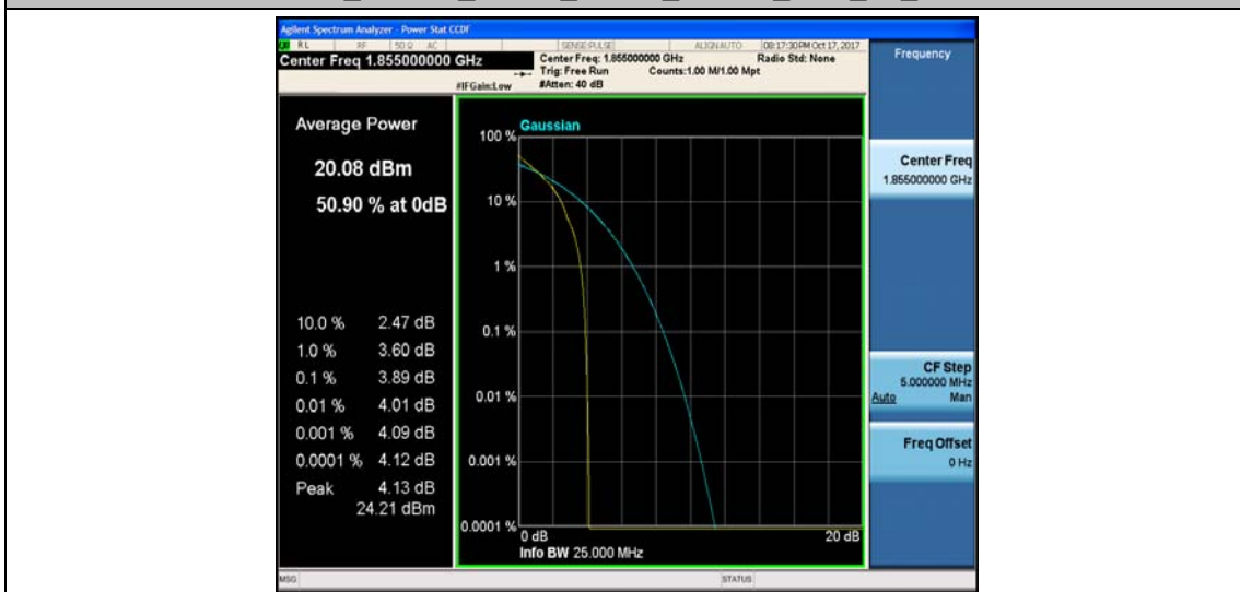
Band2_10MHz_16QAM_18650_1RB#0_4.80_13_PASS
