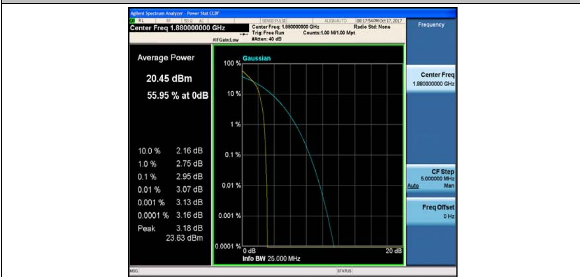
Band2_10MHz_16QAM_18900_1RB#0_3.92_13_PASS
