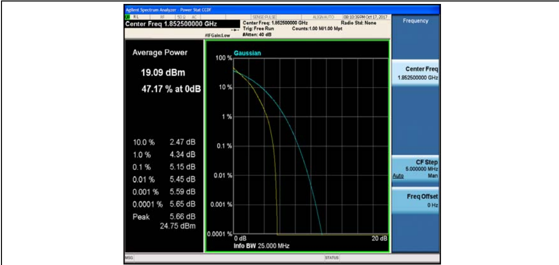
Band2_5MHz_16QAM_18625_25RB#0_5.99_13_PASS
