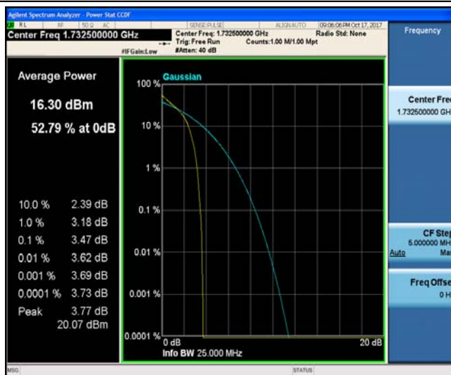
Band4_5MHz_16QAM_20175_1RB#0_4.32_13_PASS
