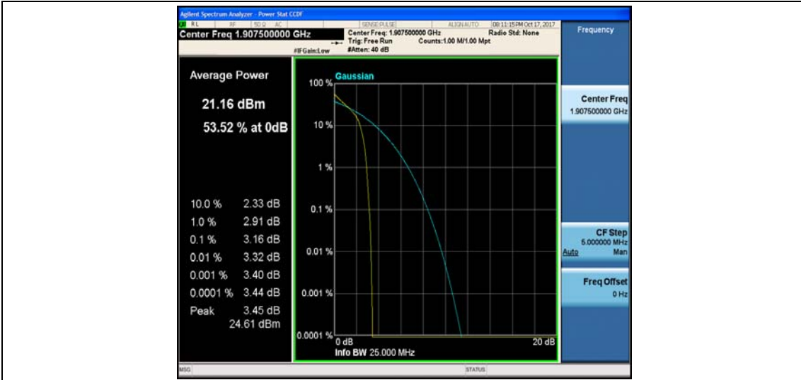
Band2_5MHz_16QAM_19175_1RB#0_3.96_13_PASS
