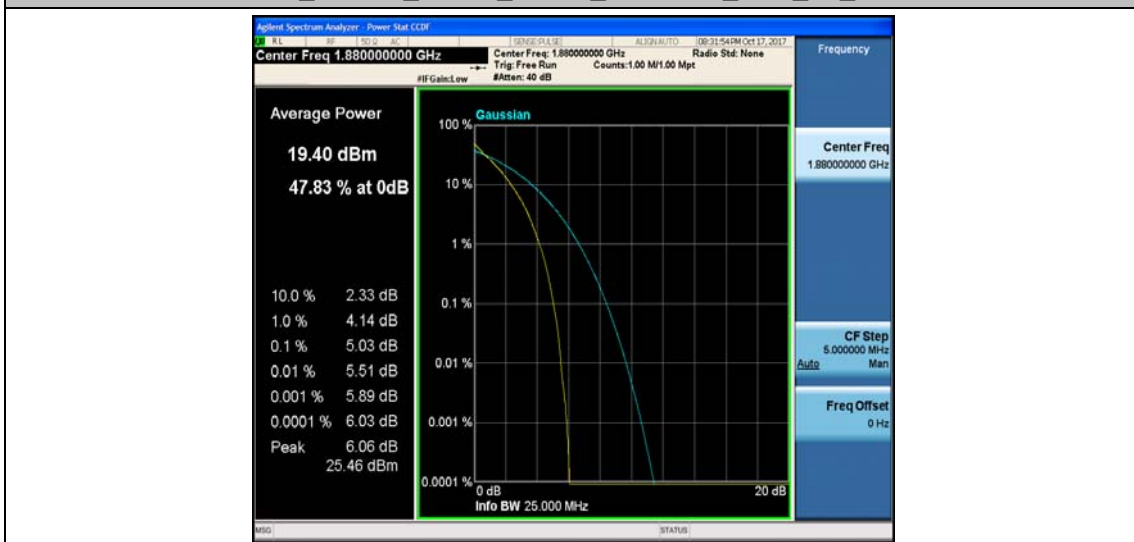
Band2_20MHz_16QAM_18900_100RB#0_5.82_13_PASS
