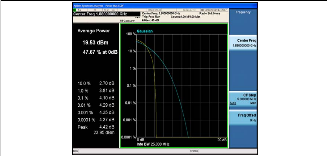
Band2_5MHz_QPSK_18900_25RB#0_4.63_13_PASS
