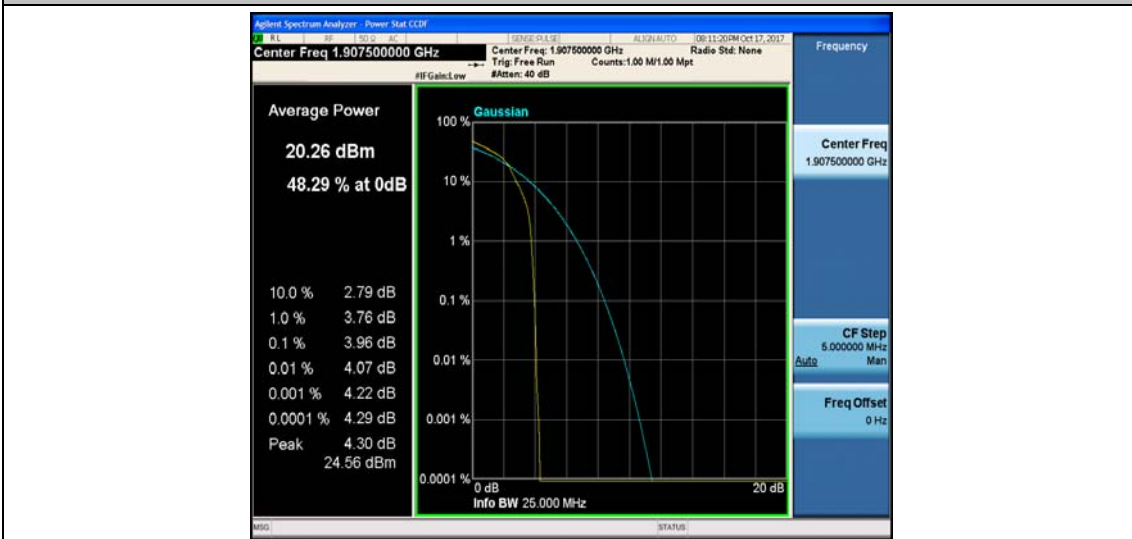
Band2_5MHz_QPSK_19175_25RB#0_4.47_13_PASS
