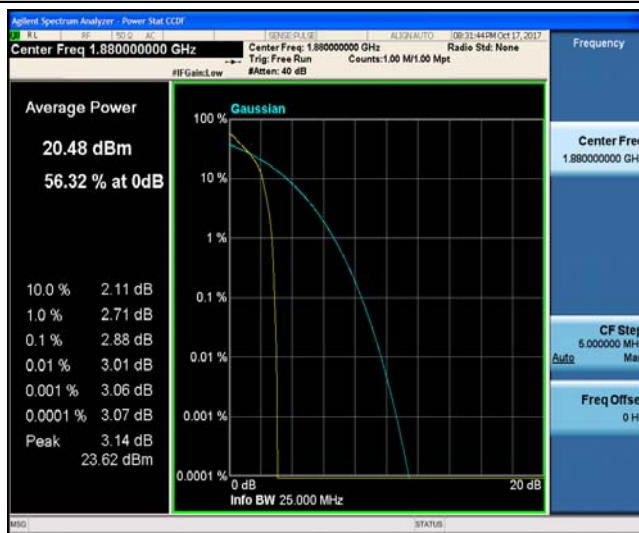
Band2_20MHz_16QAM_18900_1RB#0_3.88_13_PASS
