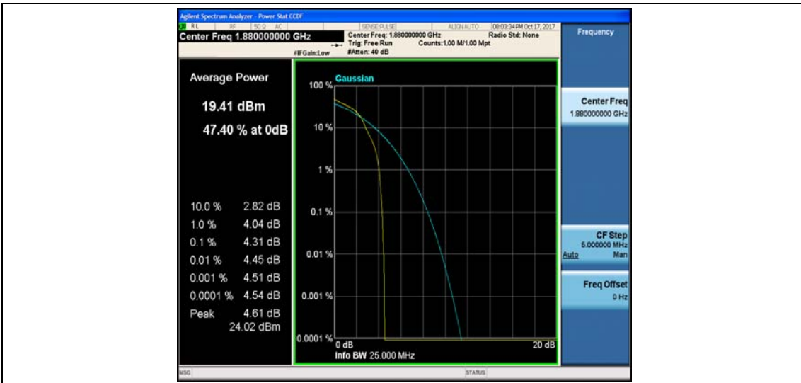
Band2_3MHz_QPSK_18900_15RB#0_4.59_13_PASS
