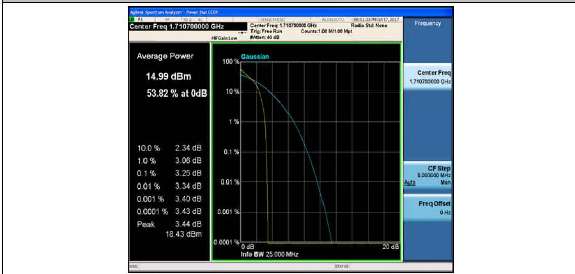
Band4_1.4MHz_16QAM_19957_1RB#0_4.20_13_PASS
