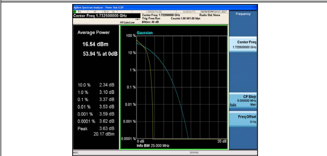
Band4_3MHz_16QAM_20175_1RB#0_4.32_13_PASS
