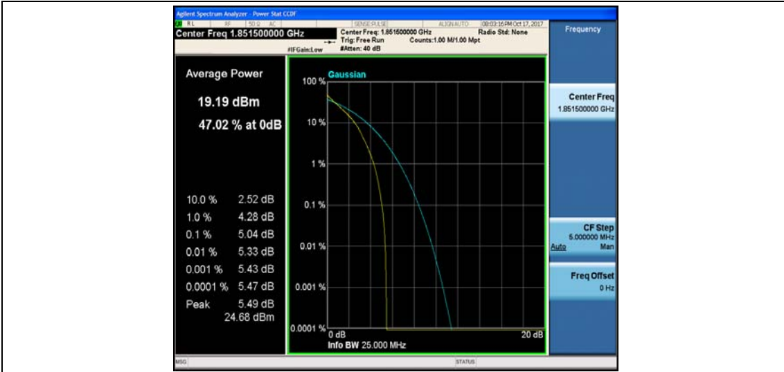
Band2_3MHz_16QAM_18615_15RB#0_5.92_13_PASS
