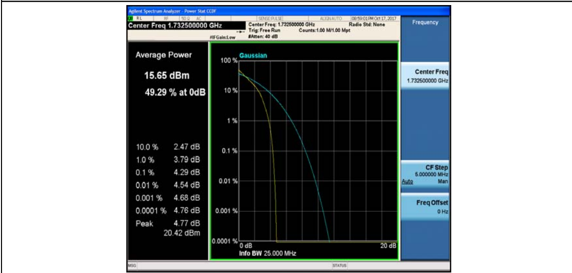
Band4_3MHz_16QAM_20175_15RB#0_5.19_13_PASS
