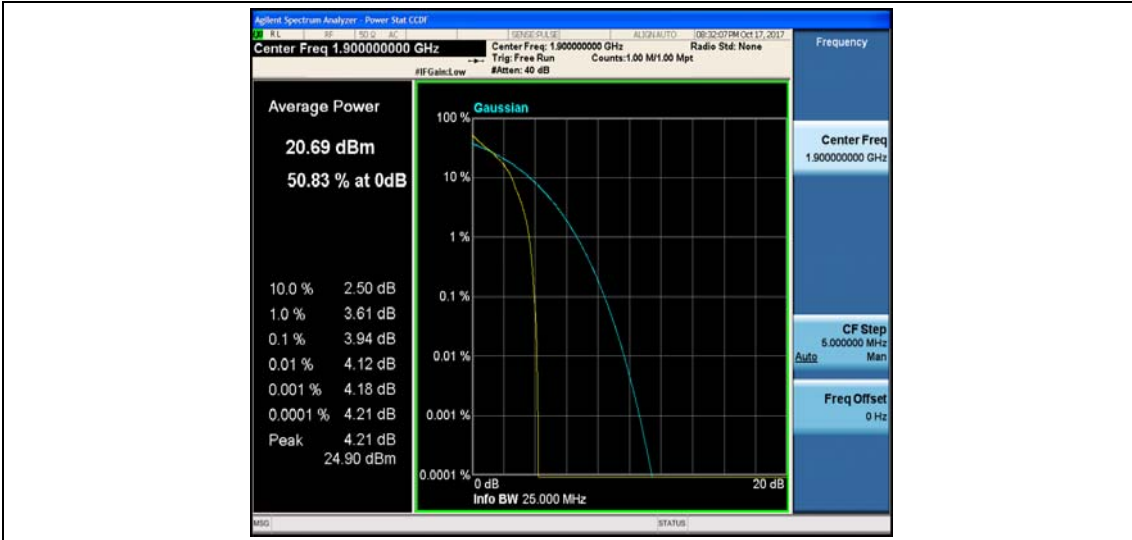
Band2_20MHz_16QAM_19100_1RB#0_4.70_13_PASS
