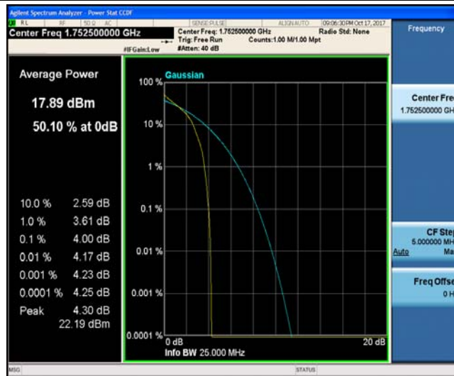
Band4_5MHz_16QAM_20375_1RB#0_4.68_13_PASS
