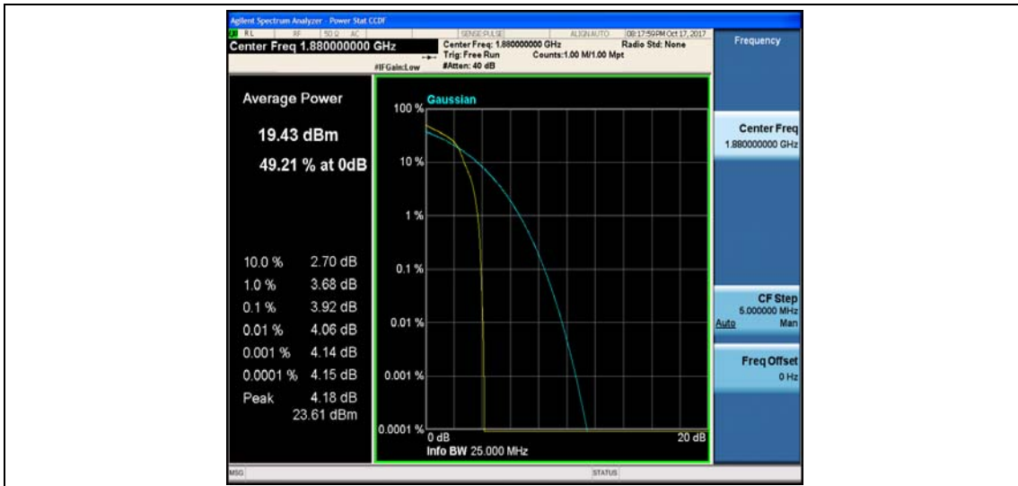
Band2_10MHz_QPSK_18900_50RB#0_4.70_13_PASS
