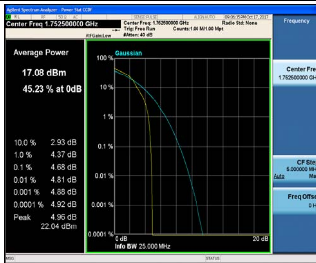
Band4_5MHz_QPSK_20375_25RB#0_4.76_13_PASS
