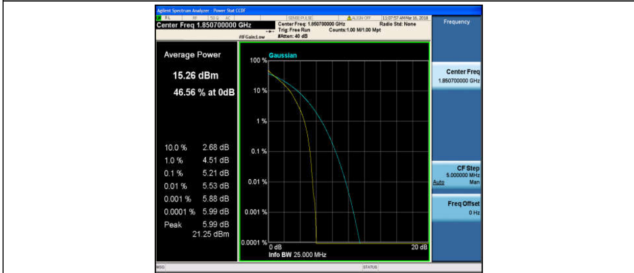
Band2_1.4MHz_QPSK_18607_6RB#0
